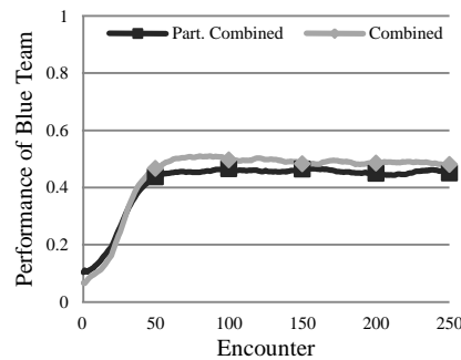
Fig. 3. Results of DS with fully and partially combined rule bases, averaged over all tactics (100 learning episodes per tactic)
