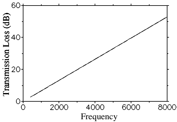
Fig. 3 Transmission loss over porous layer of turbulent boundary layer noise
