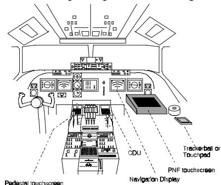
Figure 1: RFS cockpit layout
