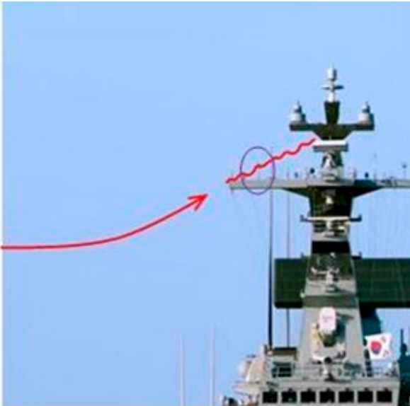
Figure 15: Upwind anemometer in turbulent wake from yard
