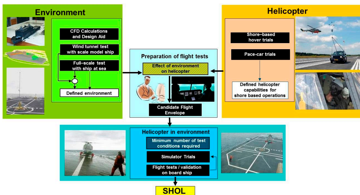
Figure 2: NLR's set-up of helicopter/ship qualification programs
