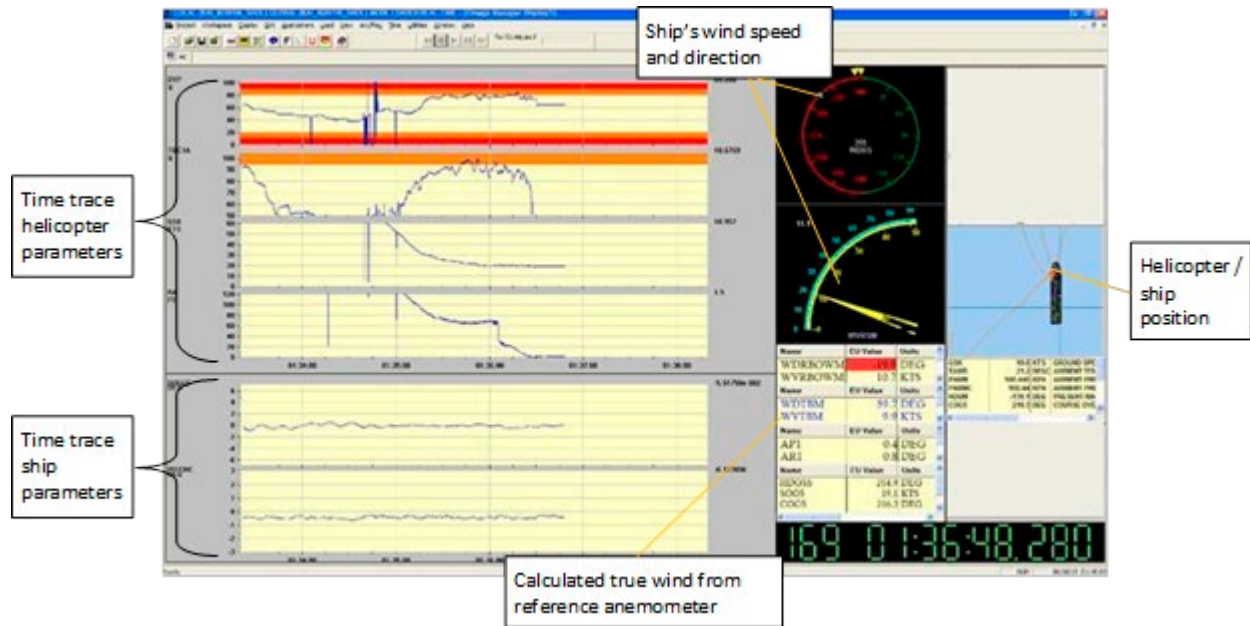
Figure 13: Example of on line data presentation for test supervision
