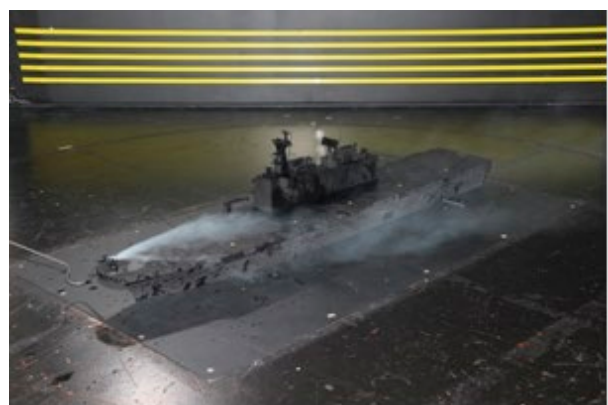
Figure 4: Visualization of the air flow with a smoke rod
