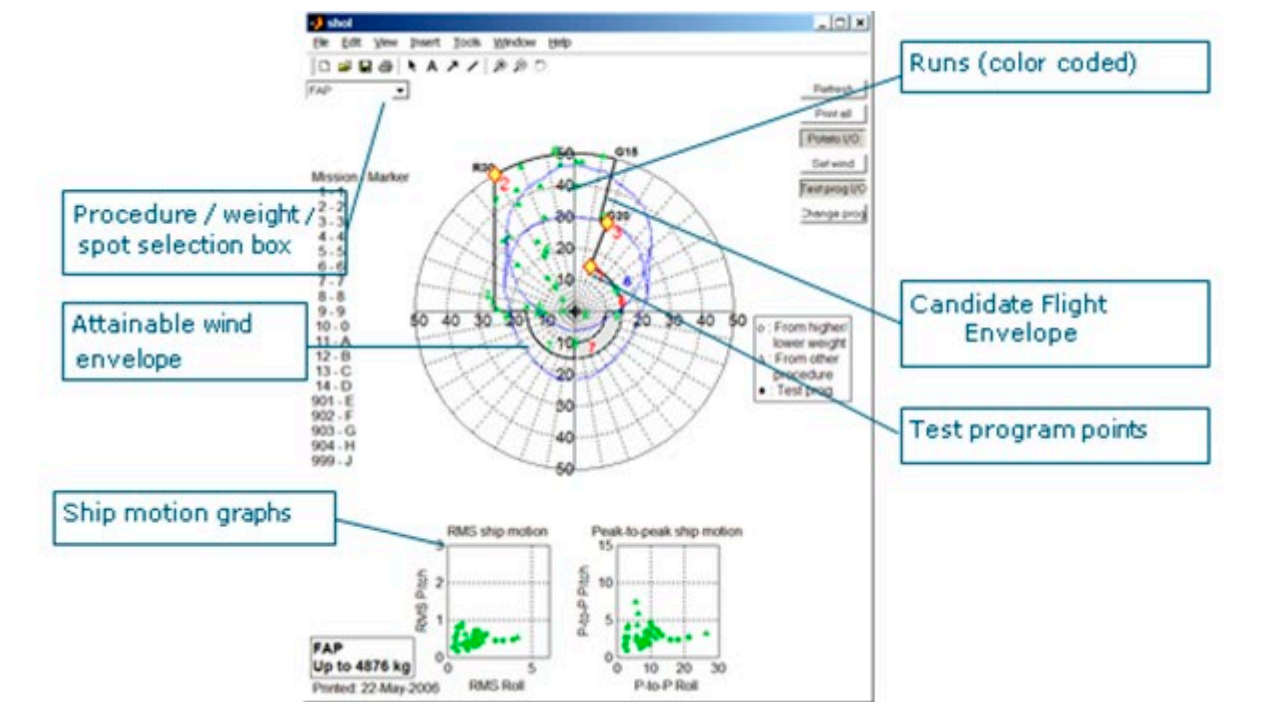
Figure 14: Example of test management tool used during the flight trials (from [2])
