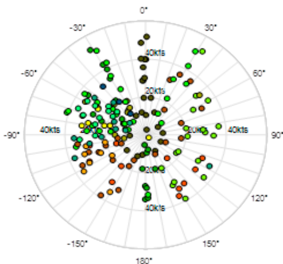
Figure 7: Overview of low speed trial test points (colors indicate flight number)
