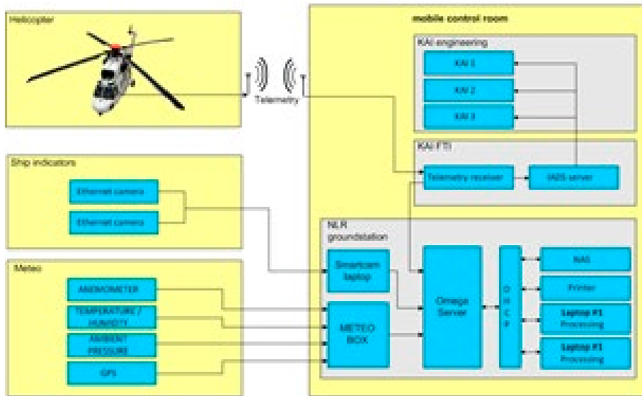
Figure 10: Flight Test Instrumentation system layout
