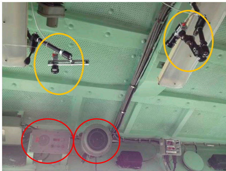
Figure 11: Non-intrusive ship instrumentation (smart cameras) installed in the flyco on board the LST
