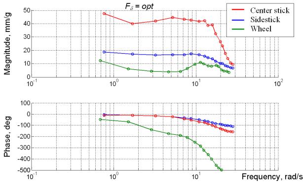
Figure 7. Comparison of the BDI for different types of control inceptors.
