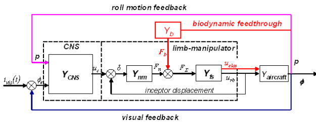
Figure 1. Block-diagram of pilot control activity for elastic aircraft.
