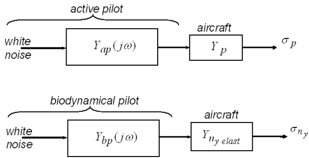
Figure 2. The models to calculate \sigma_{ny} and \sigma_p .
