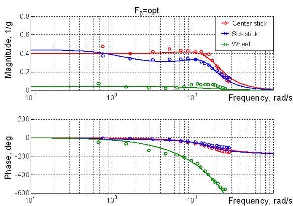
Figure 9. Comparison of the experiments and calculations. Different types of control inceptors.
