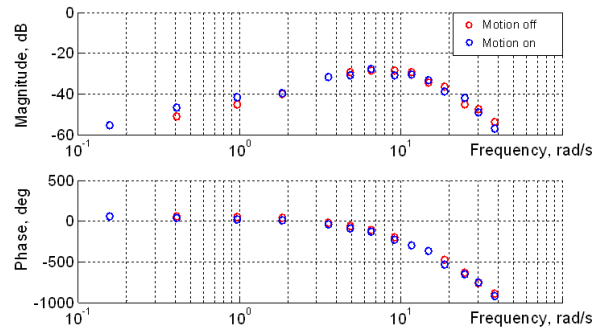
Figure 3. Active pilot describing functions demonstrating effect of high-frequency lateral accelerations
