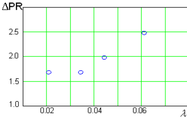
Figure 10. Effect of sidestick damping on pilot rating of elastic aircraft HQ.
