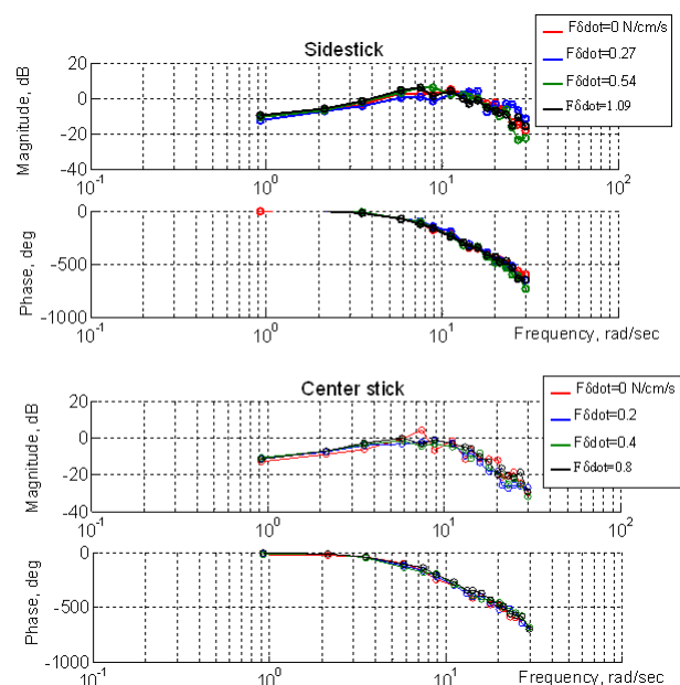
Figure 4. Effect of inceptor damping on the describing functions of the active pilot model.
