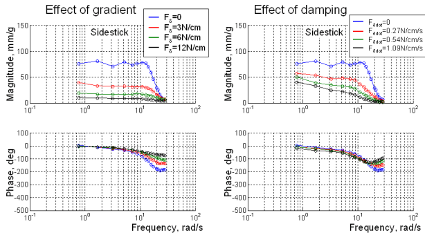
Figure 8. Effect force gradient and damping on BDI for the sidestick.
