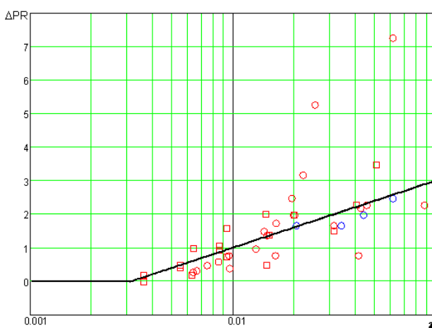
Figure 11. Empirical criterion to assess the effect of structural elasticity on pilot rating worsening.
