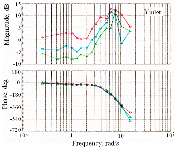
Figure 6. Effect of control sensitivity on active pilot model.
