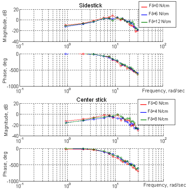
Figure 5. Effect of inceptor force gradient on the describing functions of the active pilot model.
