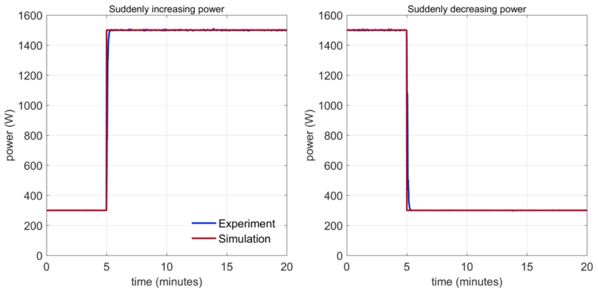
Figure 8 Evaporator heat input for both the experiment and simulation
