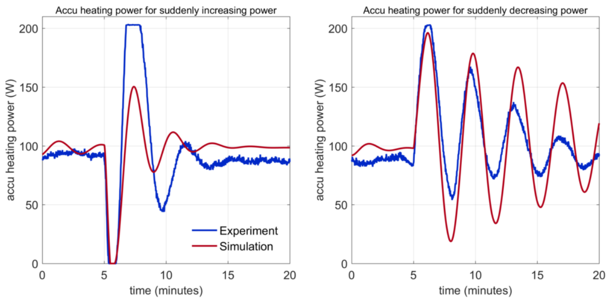
Figure 11 Heating power in the accumulator. This heating power is regulated with a PID controller
