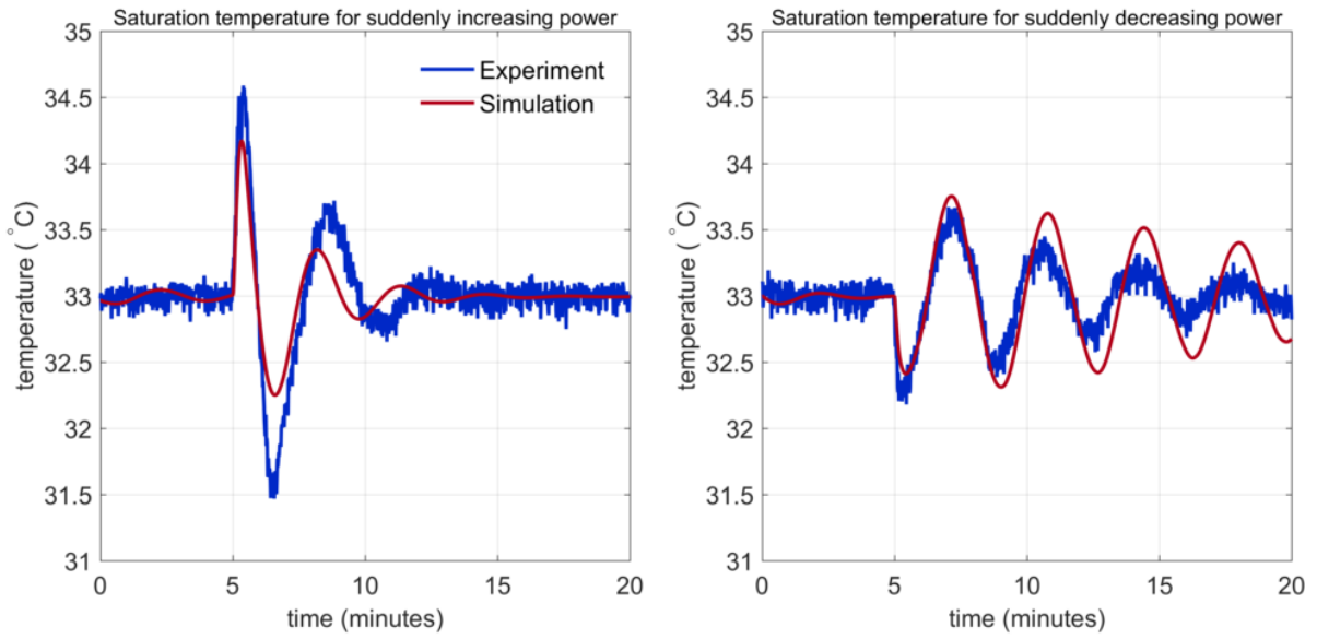
Figure 10 Saturation temperature after the evaporator
