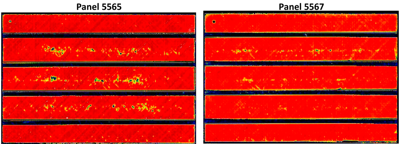
Figure 2: Ultrasonic C-scan inspection results on the skin and rib-skin. This is a composition picture of multiple inspection results. Yellow-black colour in the skin area indicates voids
