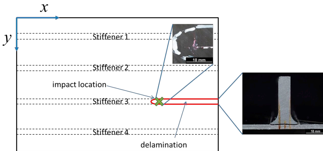
Figure 3: Schematic drawing of the rib-stiffened panel. Delamination size and location are similar to both panels
