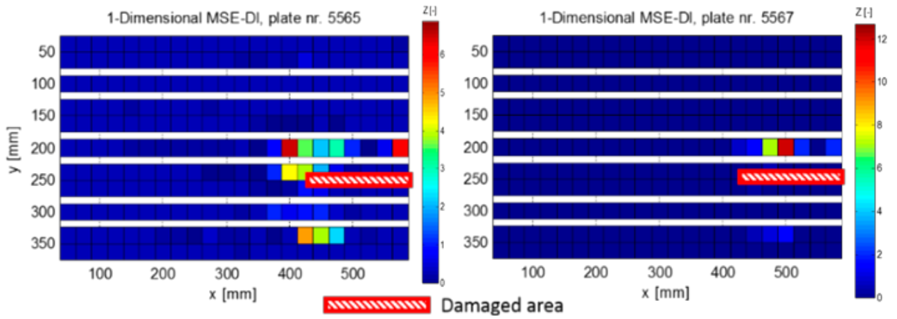
Figure 6: MSE-DI extracted from panel 5565 and 5567
