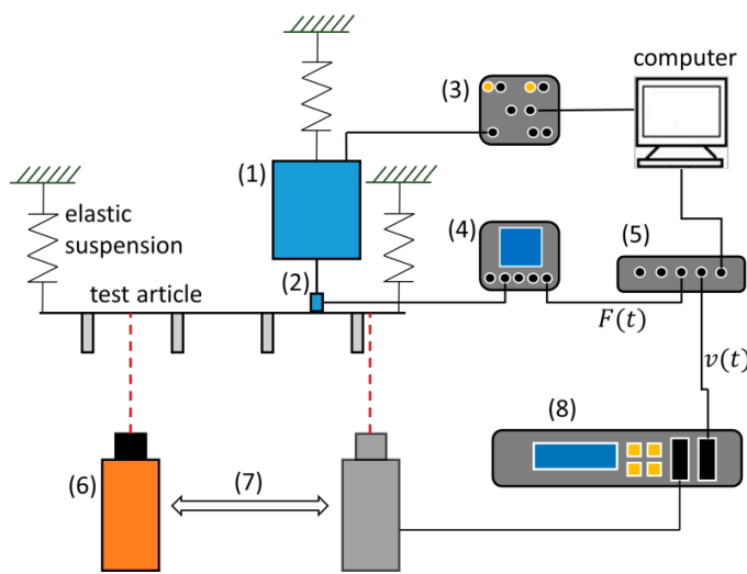
Figure 4: Experimental test setup
