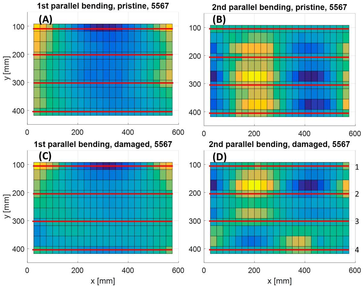
Figure 5: ODS of the plate 5567, relevant for the parallel bending moment mode shapes. (A) and (C) represent 1st bending moment before and after the impact damage respectively, (B) and (D) represent 2nd bending moment before and after the impact
