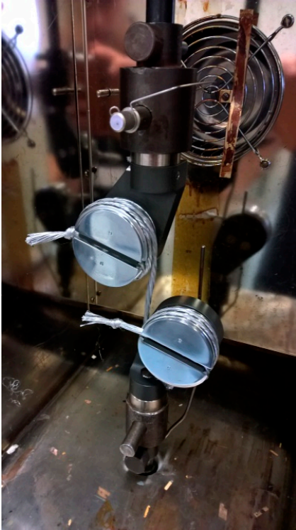
Figure 7: SPIE rope yarn strength test
