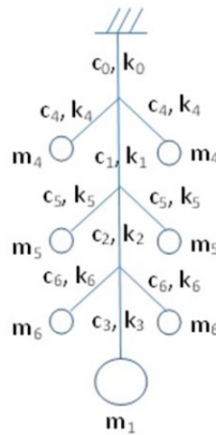
Figure 5: Mass-spring-damper model of SPIE rope
