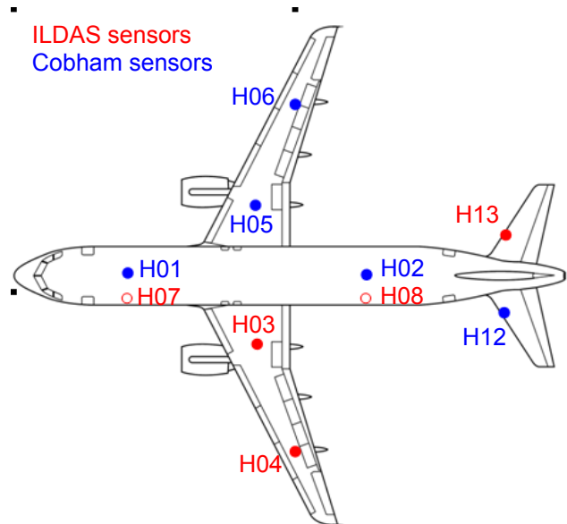
Figure 15. Sensor set on A320. Red ILDS sensors, blue Cobham sensors
