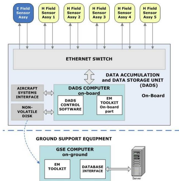
Figure 3. ILDAS System concept
