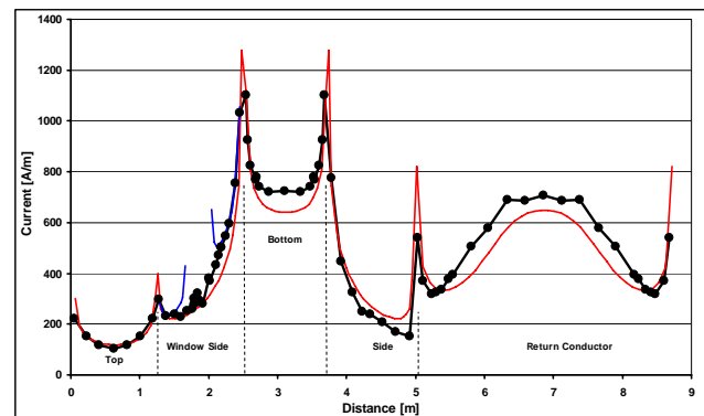
Figure 9. Measured (black and blue (window edge)) and predicted (red) current density variation around a section through the rig. The data has been normalized to an injected current of 2 kA
