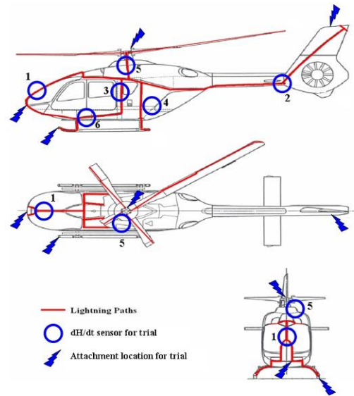
Figure 19. Sensor locations on the EC135
