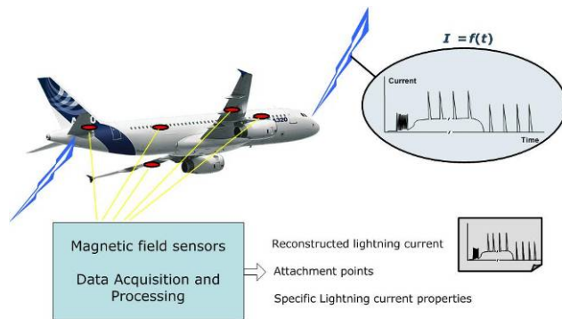
Figure 2. Lightning Characterization on the aircraft
