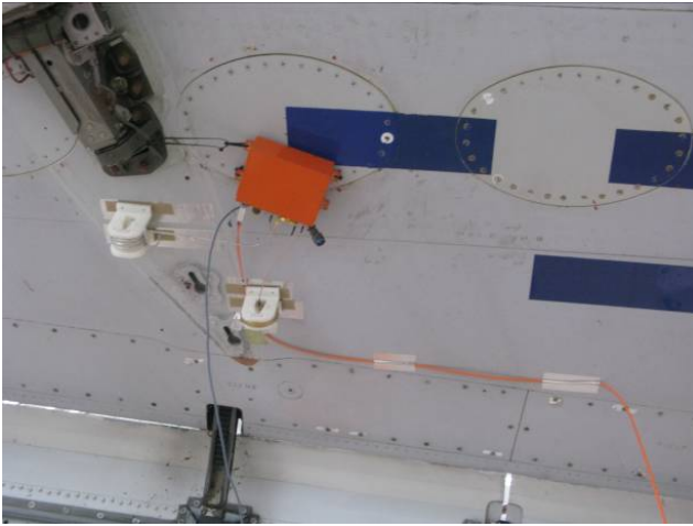
Figure 16. Inboard port wing sensor coils and electronics unit
