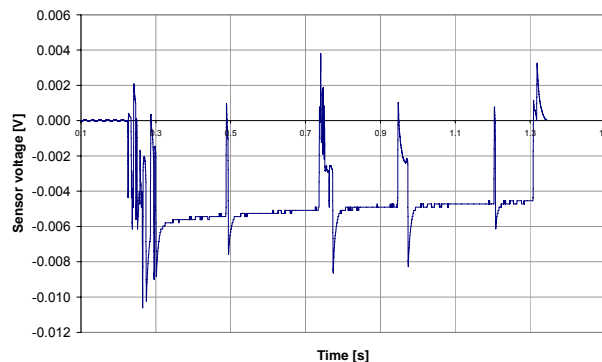
Figure 12. Voltage (proportional to continuing current) from shunt voltage sensor
