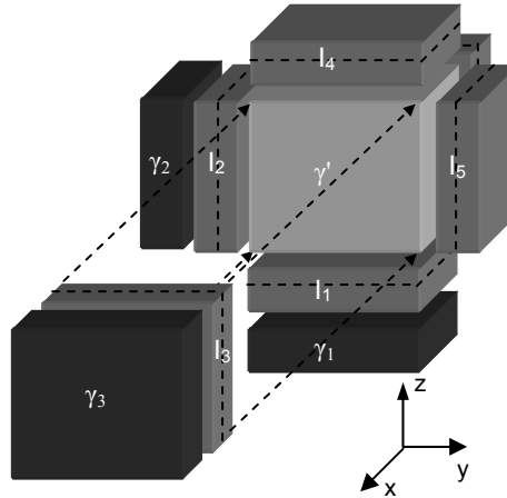
Fig. 3. Schematic Overview of Multi-phase Unit Cell.
