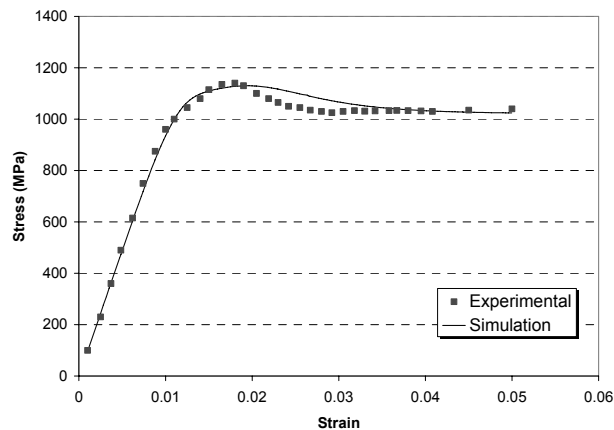
Fig. 4. Simulated stress-strain curve for CMSX-4 at 850°C at a strain rate of 3.33 \cdot 10^{-4} \text{ s}^{-1} compared to an experimentally determined curve.
