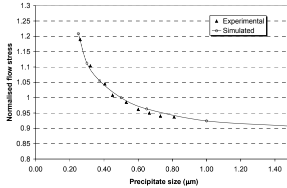
Fig. 7. Effect of changing microstructural dimensions on the steady-state flow stress for CMSX-4 at 850 °C. Experimental data for PWA1480 at 760 °C obtained from [12].
