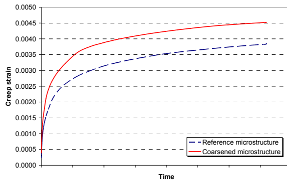
Fig. 10. Comparison of the creep strain accumulation in at a position in the root of the blade for the two different microstructures.
