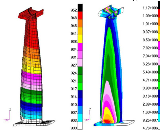
Fig. 8. Temperature (°C) and stress (Pa) distribution in the turbine blade as used for the creep analysis.
