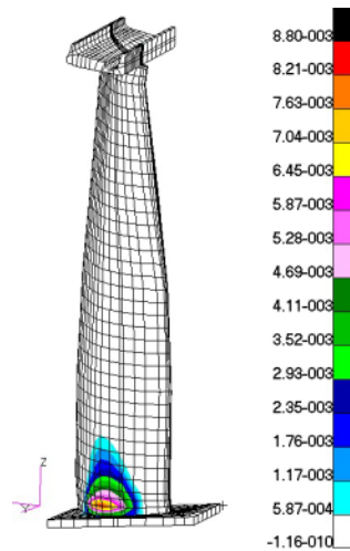
Fig.2 Calculated creep damage
