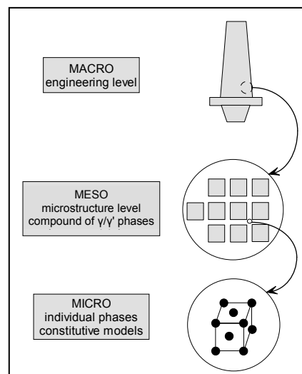
Fig. 2. Schematic Overview of Multi-scale Approach.
