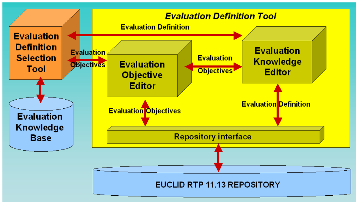
Figure 5: Evaluation Definition Tool architecture
