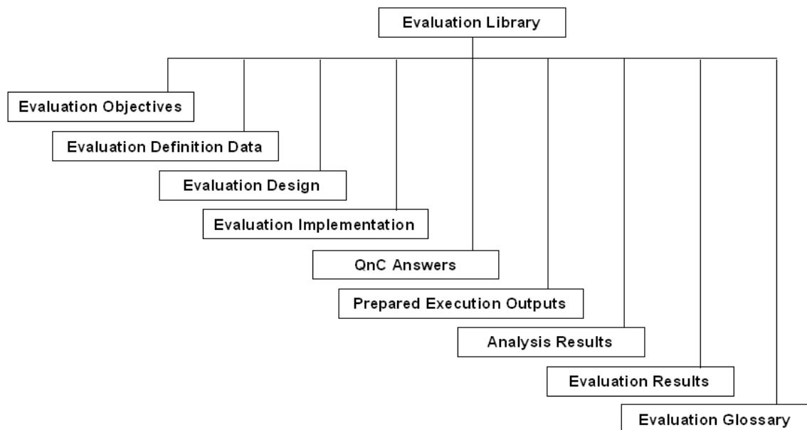
Figure 4: Evaluation Data Structure
