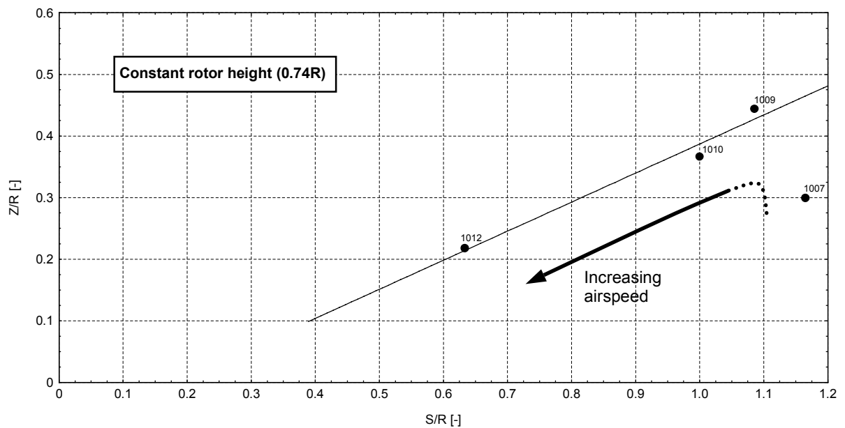
Figure 7 Measured ground vortex core positions in LLS-plane for varied air velocities
