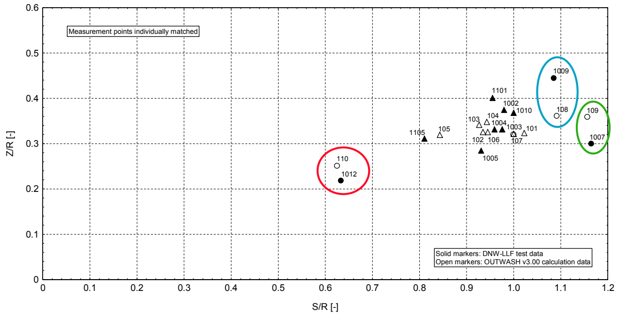
Figure 10 Comparison between OUTWASH (adapted settings) and experimental results
