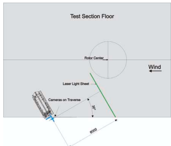
Figure 3 Location of measurement plane
