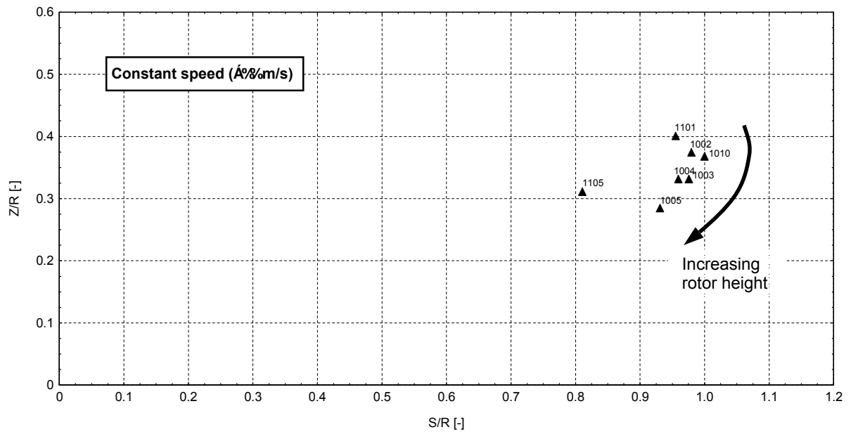
Figure 6 Measured ground vortex core positions in LLS-plane for varied rotor height
