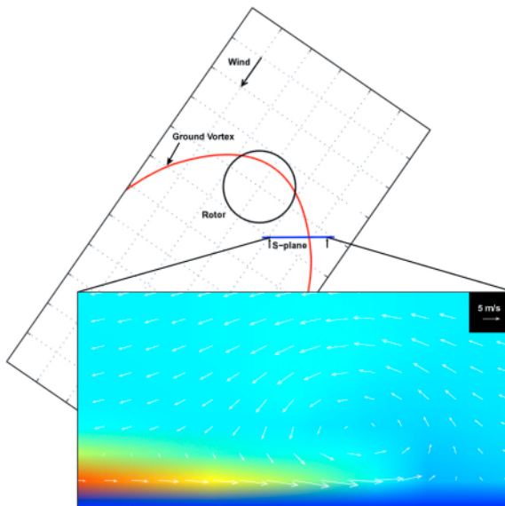
Figure 2 OUTWASH calculated ground vortex
