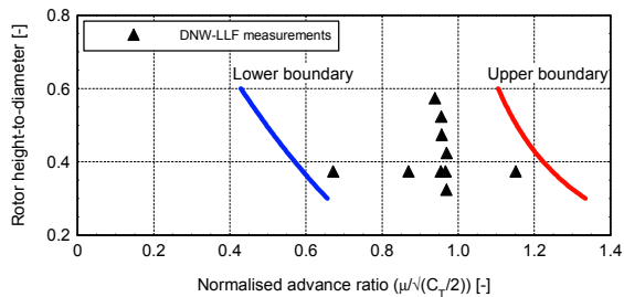
Figure 8 Boundaries for ground vortex flow regime
