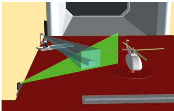
Figure 4 Test set-up in \frac{3}{4} open test section
