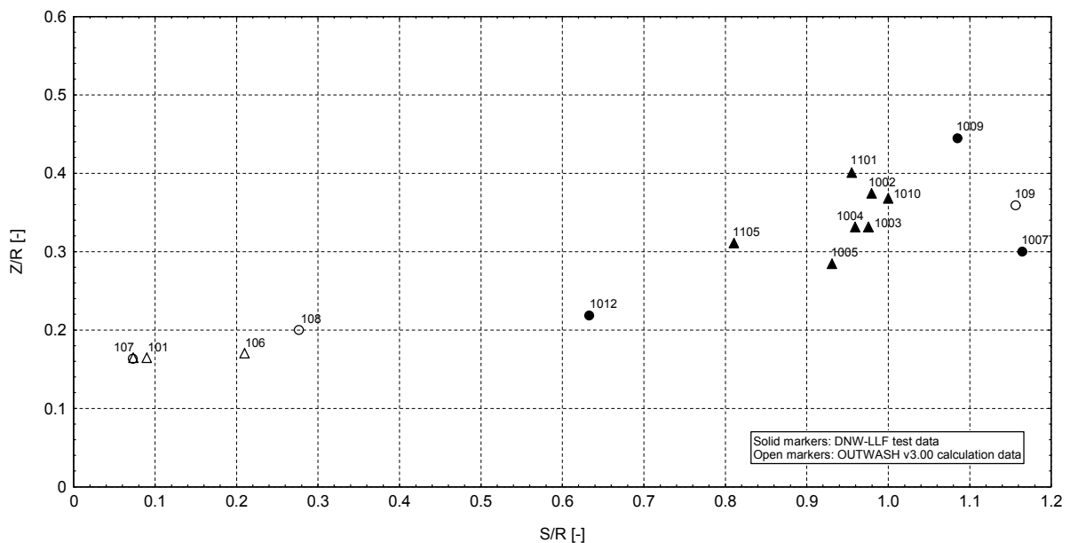
Figure 9 Comparison between OUTWASH (pre-test settings) and experimental results
