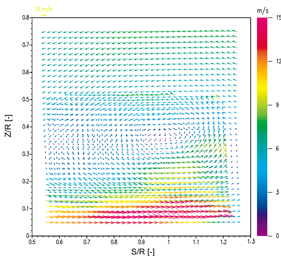
Figure 11 Comparative average vector map (run no. 1002 and OUTWASH condition no. 101).
