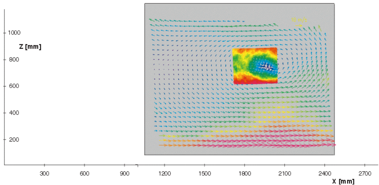
Figure 5 Ground vortex LLS and PIV average vector maps
