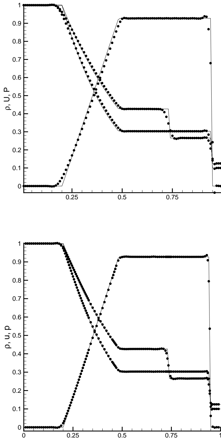
Fig. 9 Results of Sod's shock tube problem at t = 0.2531 on a uniform (top) and adapted mesh (bottom). Computed results plotted as circles, exact solution plotted as lines.
