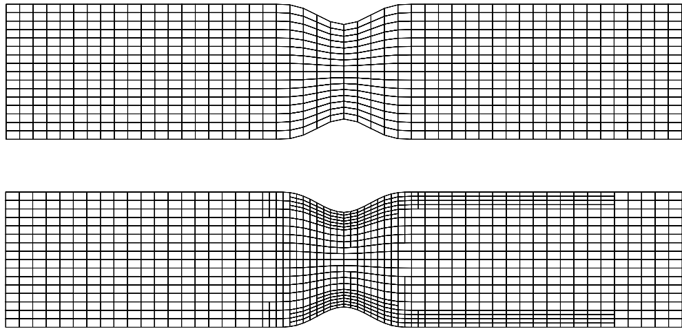
Fig. 10 Original and one time adapted mesh for converging-diverging channel.
