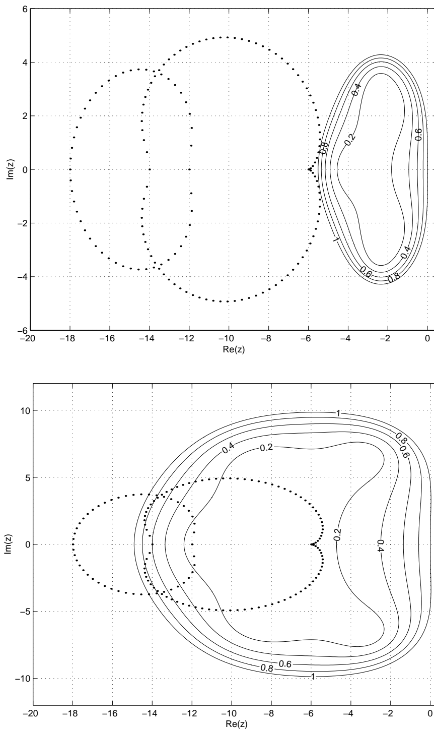
Fig. 7 Locus of the eigenvalues z_m(\theta) , \theta \in [0, 2\pi) , (dots) of the DG discretization of u_t + au_x = 0 and the stability domain of the explicit 5-stage Runge-Kutta method (40) with optimized coefficients (top) and the five stage semi-implicit Jameson Runge-Kutta scheme (bottom). CFL_{\Delta t} = 1.0 . CFL_{\Delta \tau} = 6.0 , no grid velocity.
