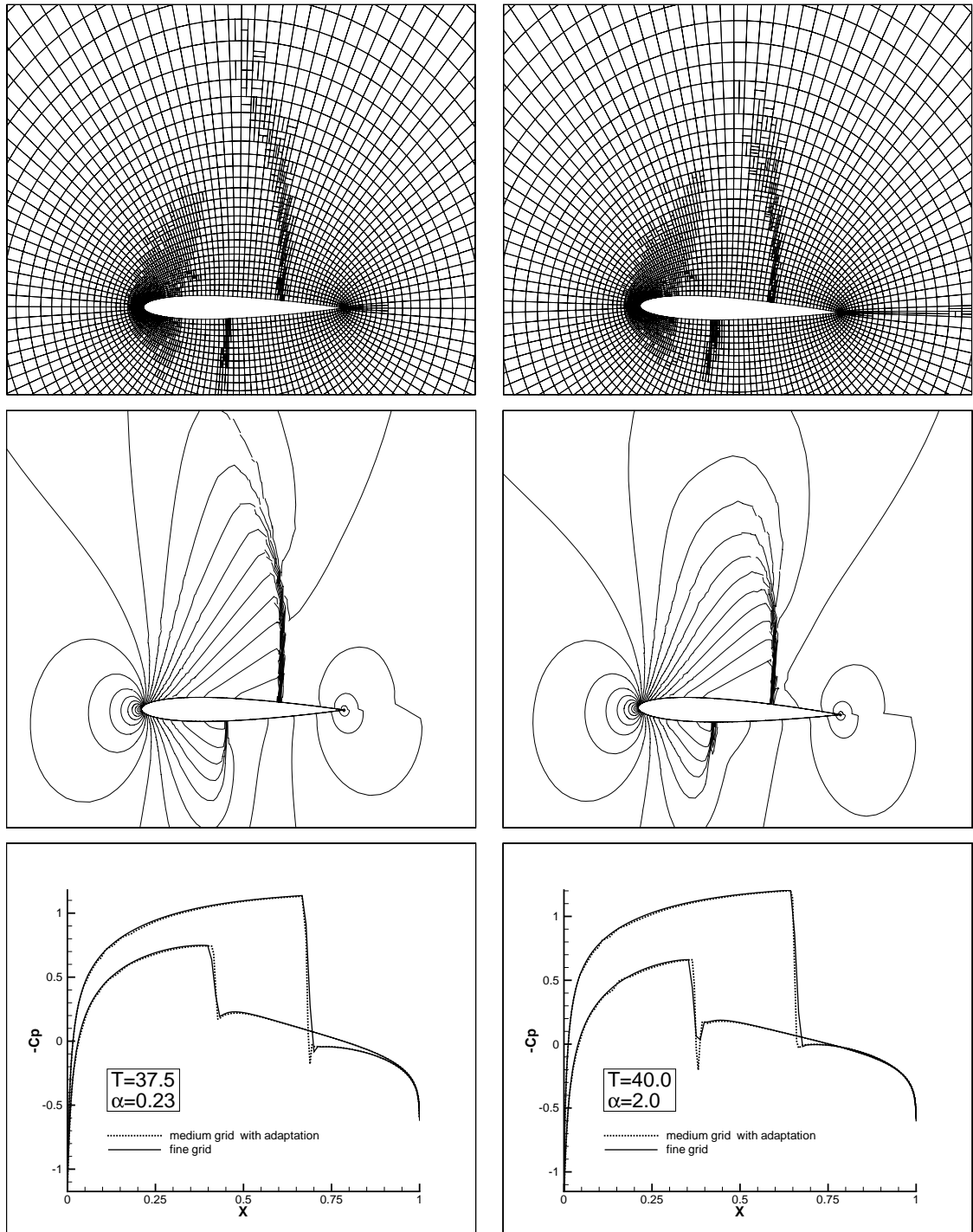
Fig. 14 Adapted mesh around oscillating NACA 0012 airfoil, contours of density, and pressure coefficient C_p on the airfoil surface for \alpha = 0.23^\circ (pitching upward) and \alpha = 2.0^\circ (pitching upward) ( M_\infty = 0.8 , \omega = \pi/10 ).
