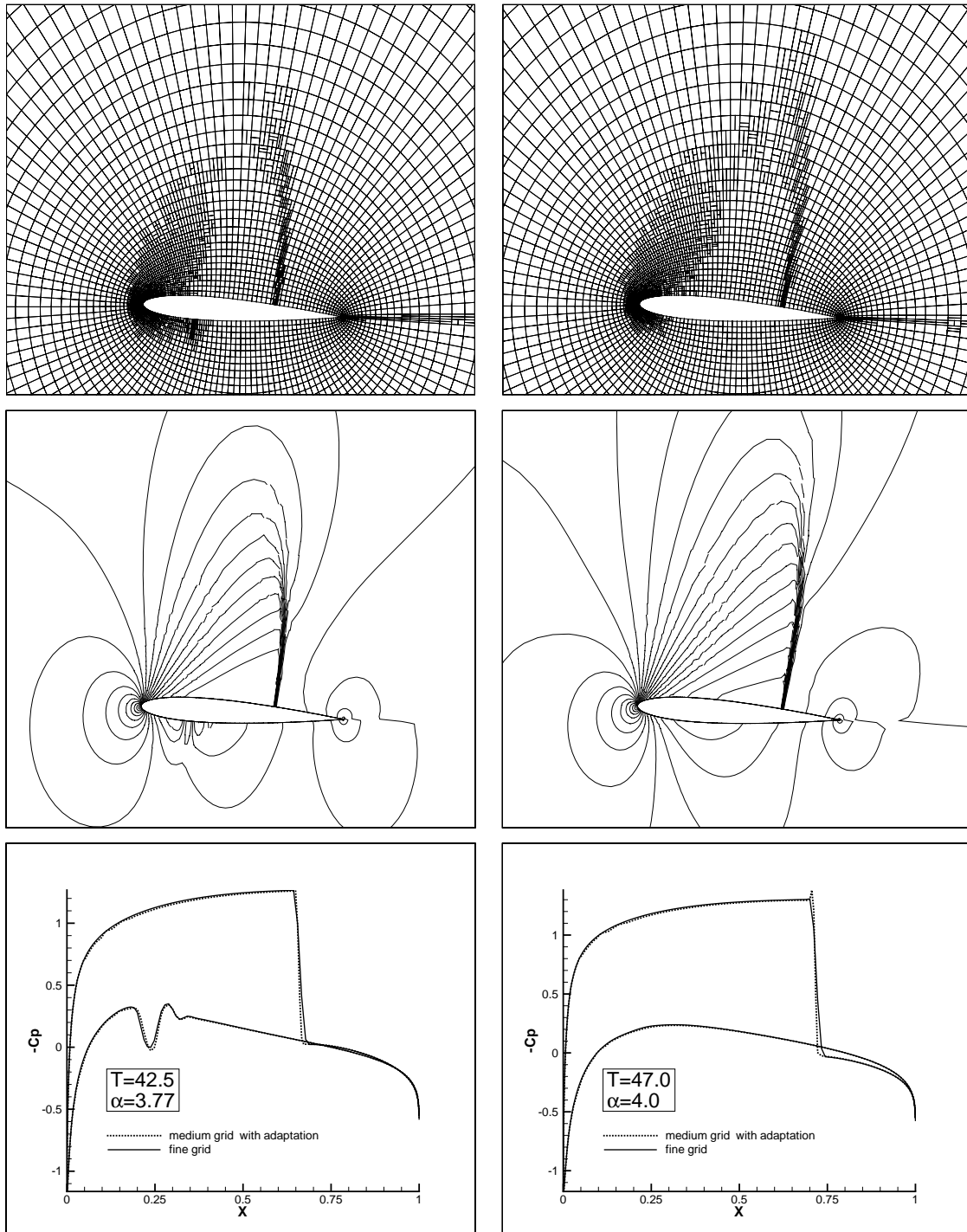
Fig. 15 Adapted mesh around oscillating NACA0012 airfoil, contours of density, and pressure coefficient C_p on the airfoil surface for \alpha = 3.77^\circ (pitching upward) and \alpha = 4.0^\circ (pitching downward) ( M_\infty = 0.8 , \omega = \pi/10 ).
