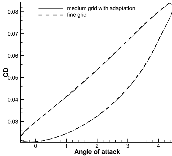
Fig. 12 Lift and drag coefficient on oscillating NACA 0012 airfoil ( M_\infty = 0.8 , \omega = \pi/10 ).
