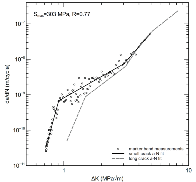
Fig. 12. Small crack growth measurements and small crack depth vs. cycles fit. The long crack a-N fit corresponds to the 7075-T7351 M(T) specimen in Fig. 5.
