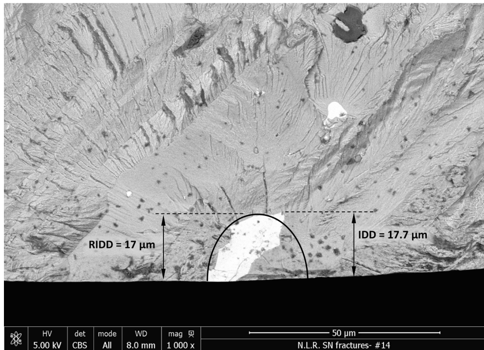
Fig. 16. SEM image of an \text{Al}_{12}\text{Fe}_3\text{Si}(\text{Cr,Cu}) constituent particle from which crack nucleation occurred. The black ellipse has a depth of 17 \mu\text{m} and an a/c ratio of 1.29.
