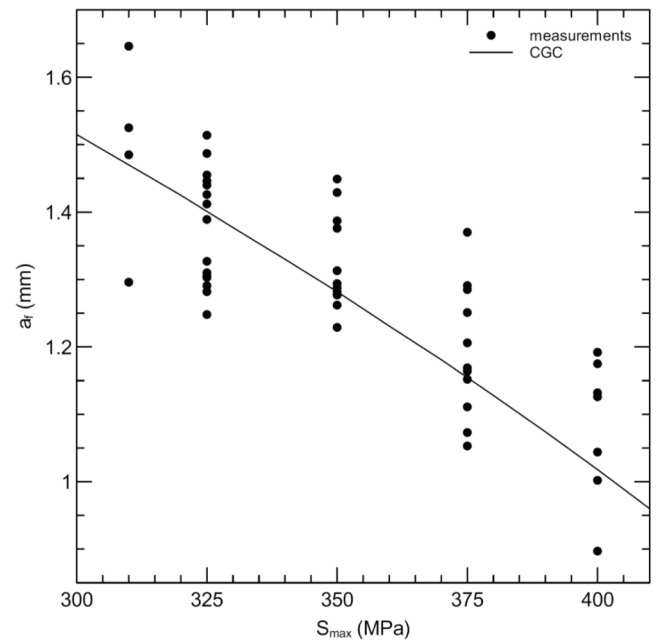
Fig. 19. Crack depth at failure as a function of the maximum stress for the smooth round S-N coupons ( R = 0.1 ).
