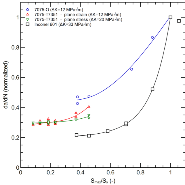
Fig. 11. Normalized FCGR as a function of normalized S_{max} for different materials and R = 0.1 . The S_{max} and the FCGR at 12 and 33 MPa \sqrt{m} for 7075-O and Inconel 601, respectively, are normalized by the material's yield stress and the FCGR at those \Delta K values for the specimens tested with a maximum stress equal to the yield stress. The FCGR for 7075-T7351 was arbitrarily scaled such that the normalized FCGR is 0.3 at S_{max} = 80 MPa ( S_{max}/S_y = 0.185 ). The curves are best fit by eye.
