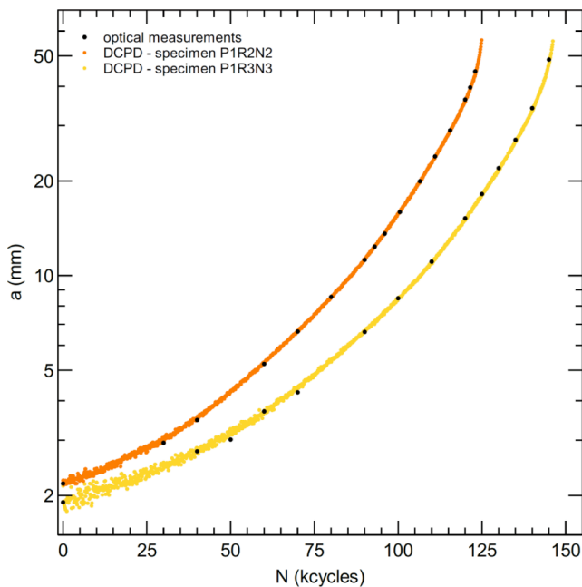
Fig. 2. Crack length vs. cycles ( a - N ) curve for two 7075-T7351 M(T) specimen tested at S_{\max} = 80 MPa and R = 0.1 . The coloured points indicate the crack length measurements using DCPD and the black dots indicate the optical crack length measurements.
