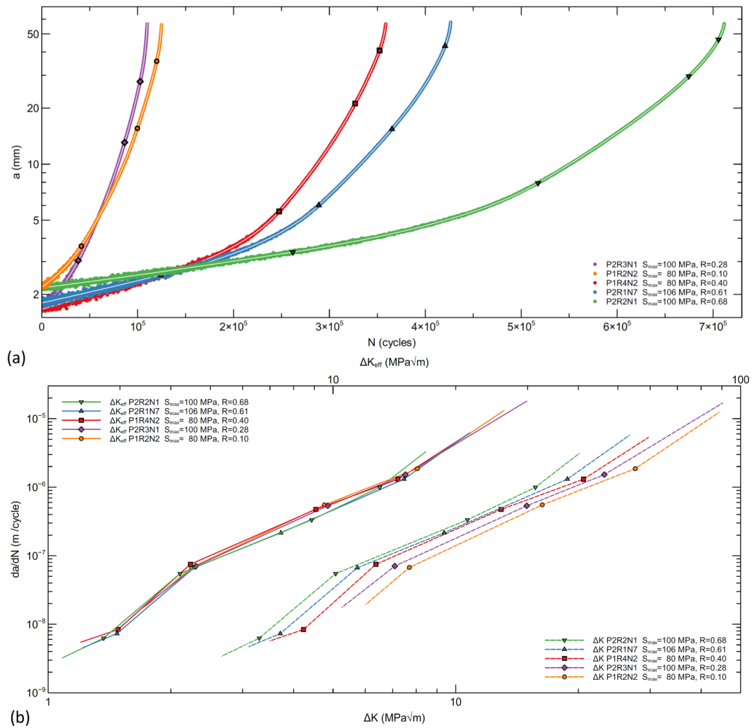
Fig. 4. (a) Crack length vs. cycles ( a - N ) curves for 7075-T7351 M(T) specimens tested at different S_{max} and R . The white lines indicate the fit using Eq. (7) and the black symbols in the white lines indicate transitions points. (b) FCGR as a function of \Delta K and \Delta K_{eff} . The transition points are indicated by the same symbols.
