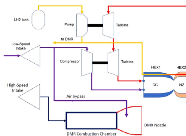
Fig. 7 Schematics of ATR and DMR engine layout
