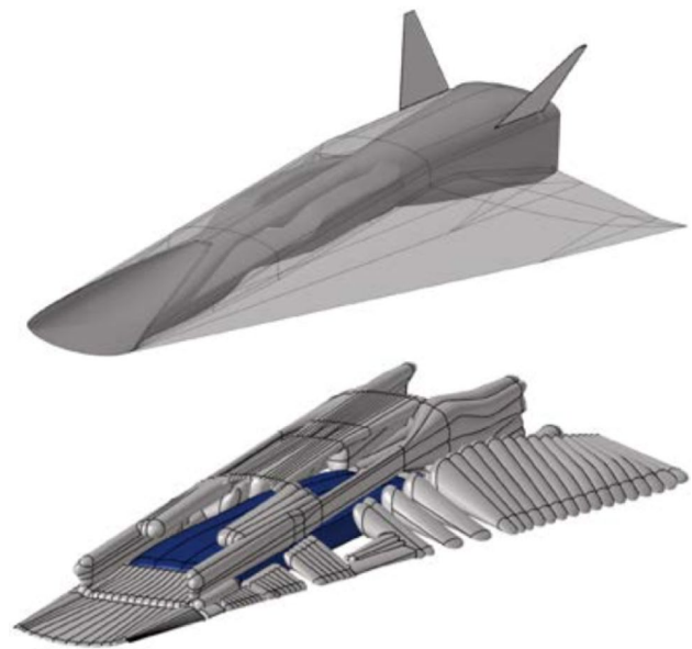
Fig. 5 STRATOFLY MR3 multi-bubble multi-functional structure
