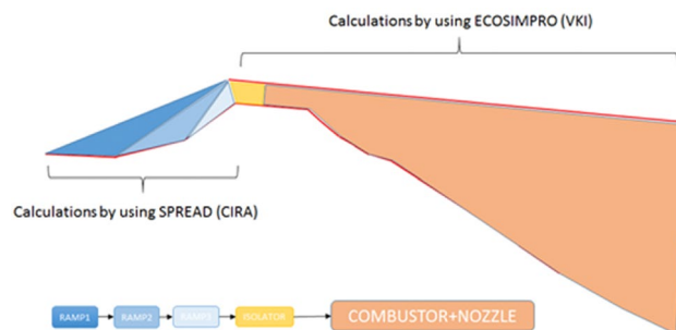
Fig. 12 MR3 DMR engine flowpath sketch
