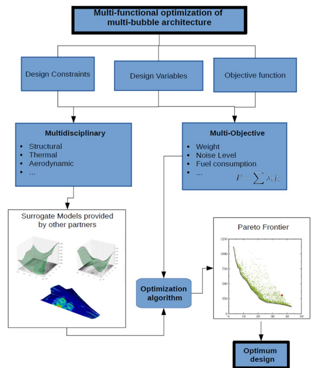
Fig. 6 Flowchart of multi-objective multidisciplinary optimization
