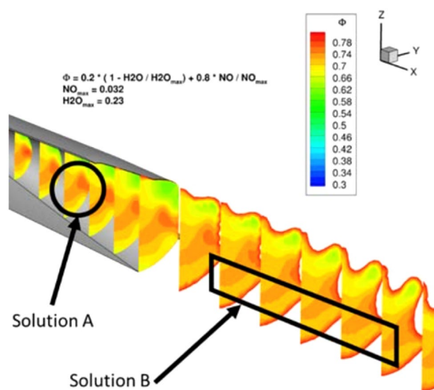
Fig. 11 CFD rebuilding of TC#1478: solutions to locate NO-probe of TDLAS measurement
