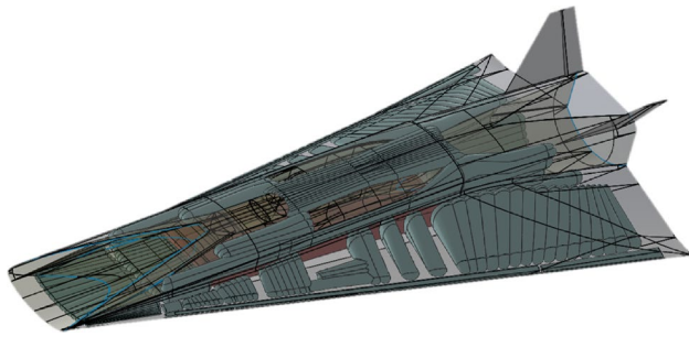
Fig. 4 STRATOFLY MR3 internal layout
