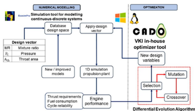
Fig. 8 Sketch of optimization methodology
