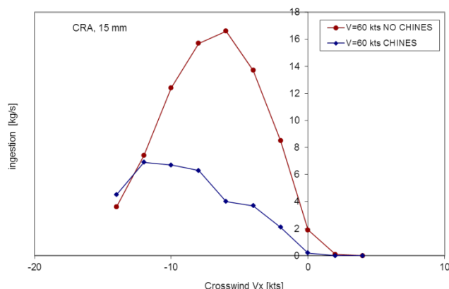
Fig. 14. CRA: ingestion lowered by nose tyre equipped with chines, ground speed 60 kts.
