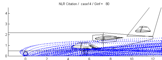
b. calculated nose gear spray
