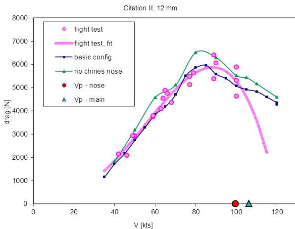
Fig. 7. Citation II: influence of chines
