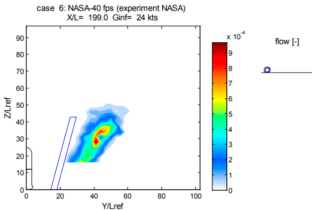
b. NASA measurement
