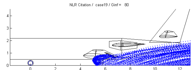
c. calculated main gear spray
