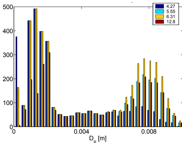
Fig. 8. Typical distribution of particle size at 4 X-positions (Citation, 60 kts, nose tyre spray)
