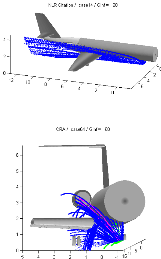
Fig. 10. CRA-aircraft: spray caused by the nose gear at 60 kts and a slight crosswind component of 4 kts towards the aircraft on the side where the engine is located.
