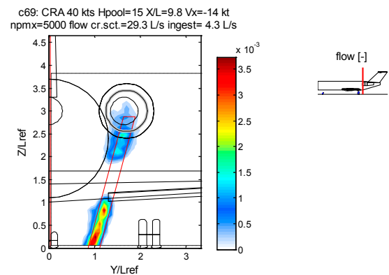
a. ground speed 40 kts, V_X = 14 kts
