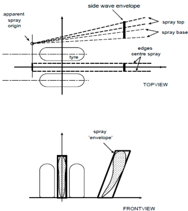
Fig. 1. ESDU spray schematization.
