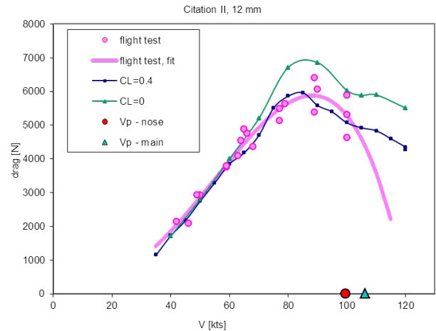
Fig. 5. Effect of wing lift on precipitation drag
