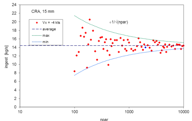
Fig. 9. Dispersion in ingestion rate as function of the number of particles used in the spray calculation for each side spray
