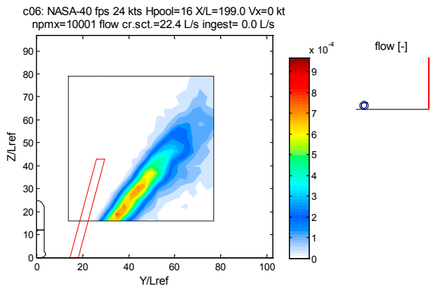
a. CRspray results
