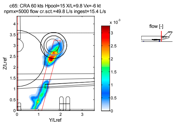
b. ground speed 60 kts, V_X = 6 kts
