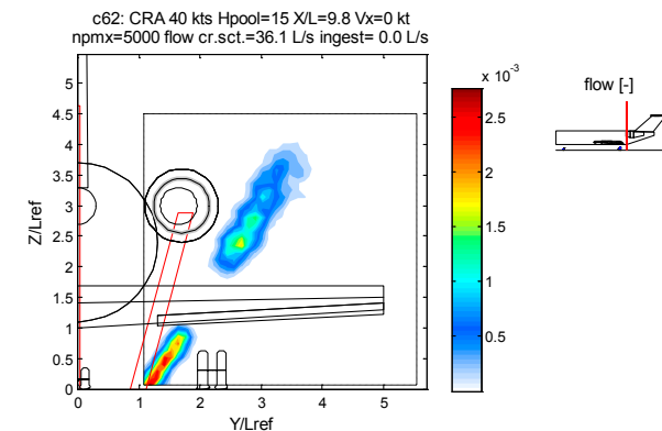
a. ground speed 40 kts
