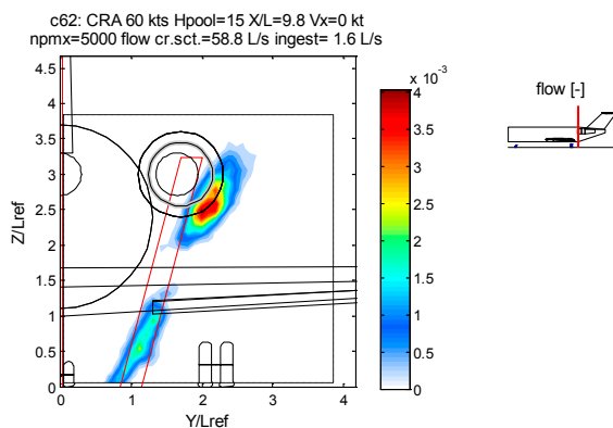
b. ground speed 60 kts
