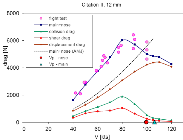
Fig. 4. Cessna Citation II: CRsray-results, compared with flight test data and AMJ rule
