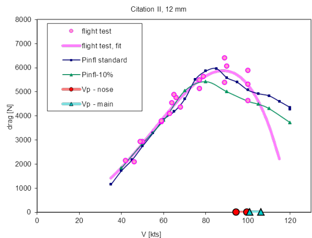
Fig. 6. Effect of reduced tyre pressure.
