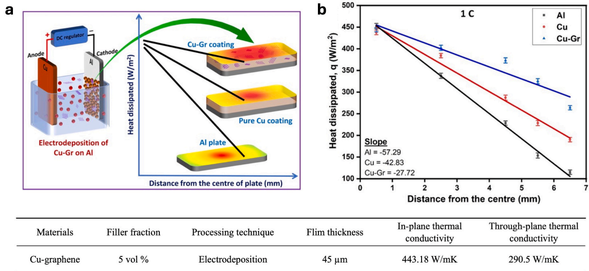
Fig. 29. Heat spreader applications of copper-graphene composite, processed by electrodeposition. (a) Schematic illustrations of the experimental setup for copper-graphene processing, (b) Heat transfer properties of copper-graphene coatings. Copper-graphene presents the highest heat dissipation rate overall coated areas, (c) Thermal properties of copper-graphene heat spreader coating [392].
