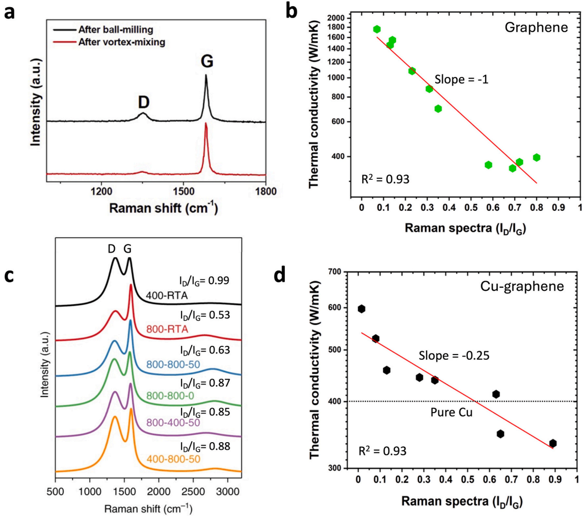
Fig. 25. (a) Raman spectra of graphene after different preparation methods, (b) Thermal conductivity as a function of I_D/I_G taken from the Raman spectrum, (c) Raman spectra of copper-graphene 2DMMC according to their fabrication conditions. The number in the first, second, and third positions presents the experimental condition for thermal annealing temperature, hot-pressing temperature in °C, and hot-pressing pressure in MPa. (d) Thermal conductivity values of copper-graphene as a function of the Raman ratio I_D/I_G taken from the Raman spectrum [49,64,66,327,330,336,338,339,350].
