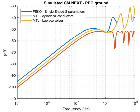
Fig. 2. Simulations of CM NEXT on a PCB with PEC ground. Blue line serves as theoretical baseline and is computed with Feko. The two other results are computed with MTL models, one for cylindrical conductors and one with a Laplace solver in which the exact PCB dimensions were included. Section V will provide more details on the simulations.
