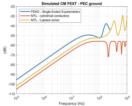
Fig. 3. Simulations of CM FEXT on a PCB with PEC ground. Blue line serves as theoretical baseline and is computed with Feko. The two other results are computed with MTL models, one for cylindrical conductors and one with a Laplace solver in which the exact PCB dimensions were included. Section V will provide more details on the simulations.
