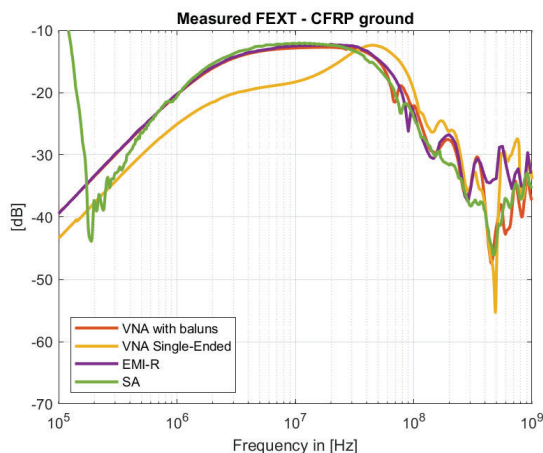
Fig. 9. Measured CM FEXT for the PCB with CFRP ground plane.
