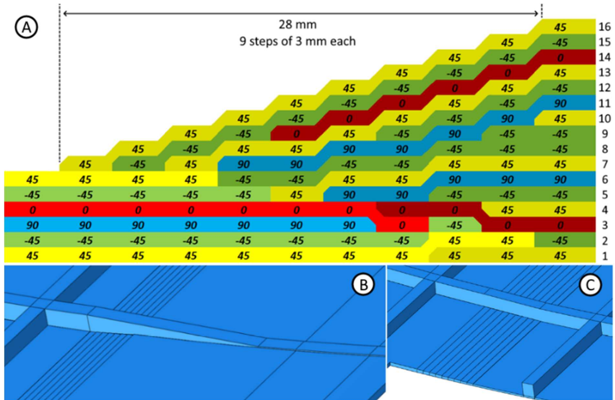
Figure 8: Composite lay-up of the full-scale panel. A) Transition from carbon (light) to glass (dark) layers. B) Transition of the rib at the edge of the panel. C) Transition of the rib at the transition of carbon to glass fibre.
