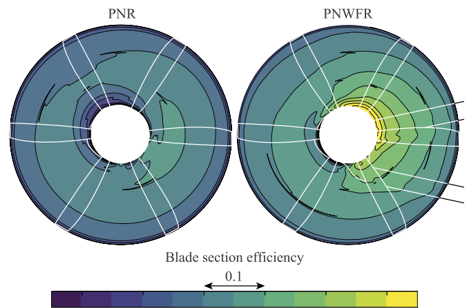
Fig. 8. The blade section efficiency T'V_\infty/P' is plotted for each circumferential position of the left propeller in cruise. The effect of the wings is shown by means of comparison of the PNR and PNWFR configuration.
