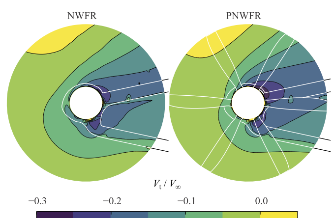
Fig. 9. Time-averaged tangential velocity component is plotted on the plane visualised in Fig. 5, upstream of the left propeller in cruise. The effect of the propeller is shown by means of comparison of the NWFR and PNWFR configuration.
