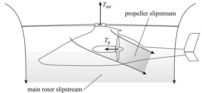
Fig. 14. Sketch of main rotor and propeller aerodynamic interaction in hover, indicating the direction of the main rotor thrust T_{mr} and propeller thrust T_p .
