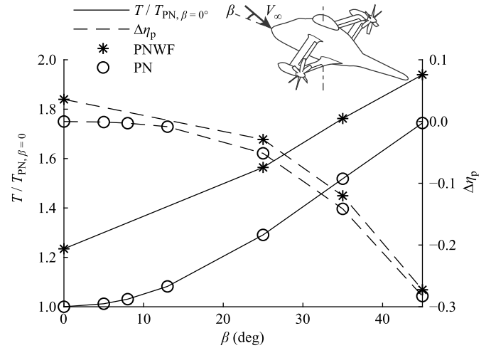
Fig. 13. Right propeller thrust T and propulsive efficiency \eta_p = (TV_\infty \cos \beta) / P are plotted against sideslip \beta at constant blade pitch angle for a reduced manoeuvring cruise speed for V_\infty = 140 kt (72.0 m/s). A comparison is shown between the PNWF and PN configuration and quantities are with respect to PN configuration quantities at zero sideslip.
