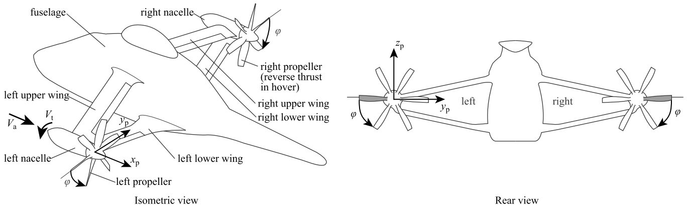
Fig. 1. Sketches of the Airbus RACER without main rotor and tailplanes. Propeller blade phase angle \varphi and axial and tangential velocity components V_a and V_t are indicated.
