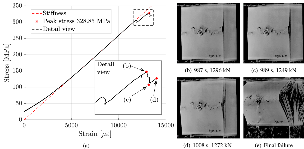
Figure 19. CAI test of a 40 mm thick specimen subjected to a 55 J drop-weight impact (40-QI-LM-55-4) with in (a) the stress-strain curve and detail view of progressive sub-laminate buckling (b)-(d) leading to (e) final failure with a MMP failure mechanism.
