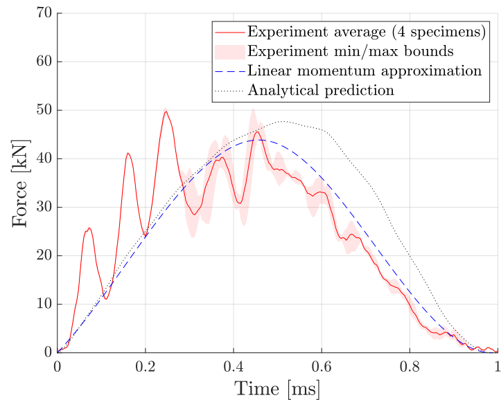
Figure 5. Averaged force history for 55 J drop-weight impact tests on 20 mm thick specimens.
