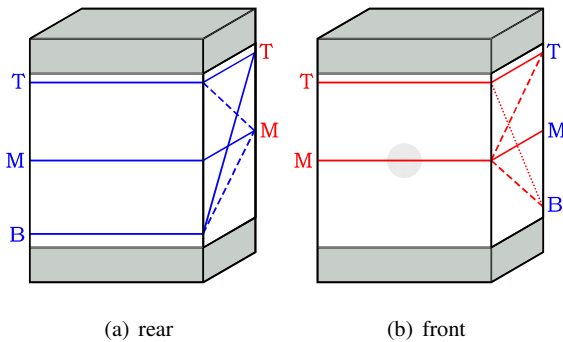
Figure 18. Failure mechanisms observed during the CAI tests with buckling of sub-laminates at the middle (M), top (T), or bottom (B) of the specimen. Distinction is made between symmetric failure (MM and TT) and asymmetric failure (MT, MB, and TB). A distinction between Progressive (P) and Instant (I) failure is made.
