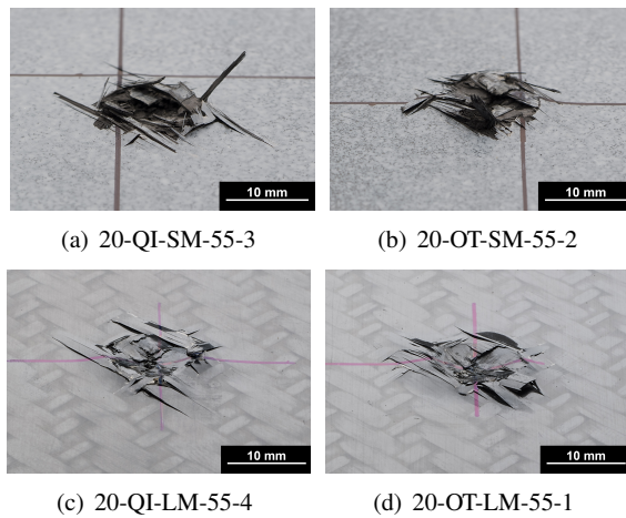
Figure 10. Typical dents for 55 J drop-weight impacts and gas-cannon impacts on 20 mm thick specimens with a QI and OT layout.
