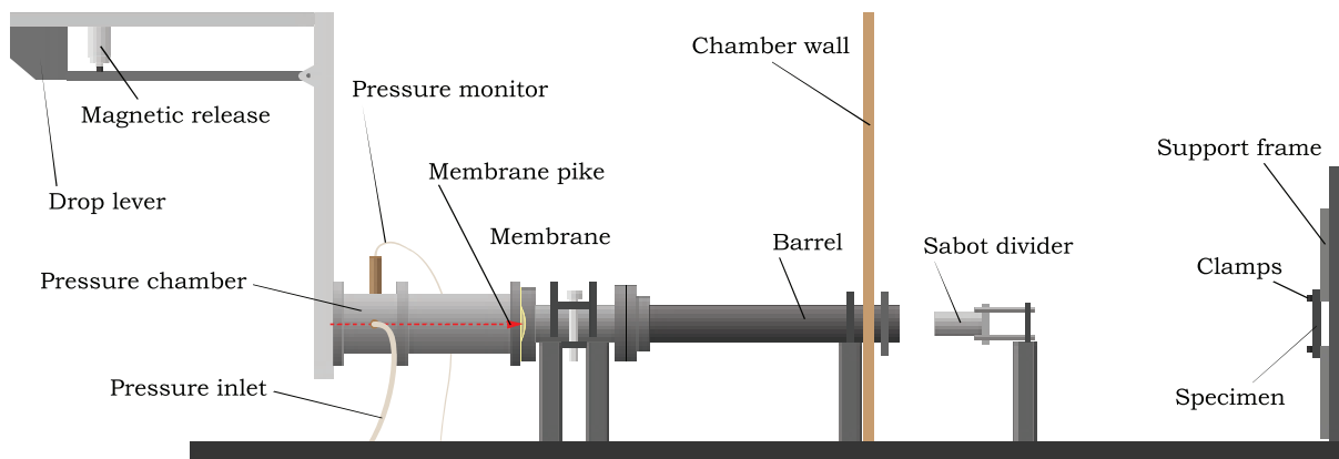
Figure 6. Illustration of the gas-cannon test setup used for small-mass (SM) impacts.
