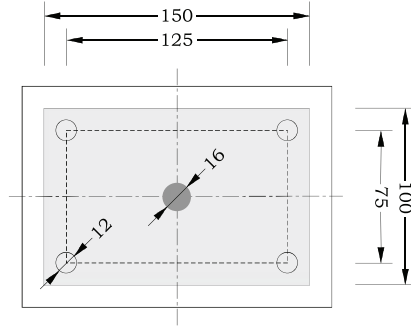
Figure 2. Top-view of the support fixture used for the drop-weight and gas-cannon tests.
