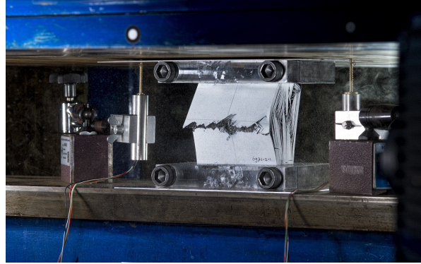
Figure 11. The CAI test setup with a 40 mm thick specimens subjected to a 100 J gas-cannon impact (40-QI-SM-100-1) showing a Middle Top Progressive (i.e., MTP) failure mechanism as classified in Figure 18.
