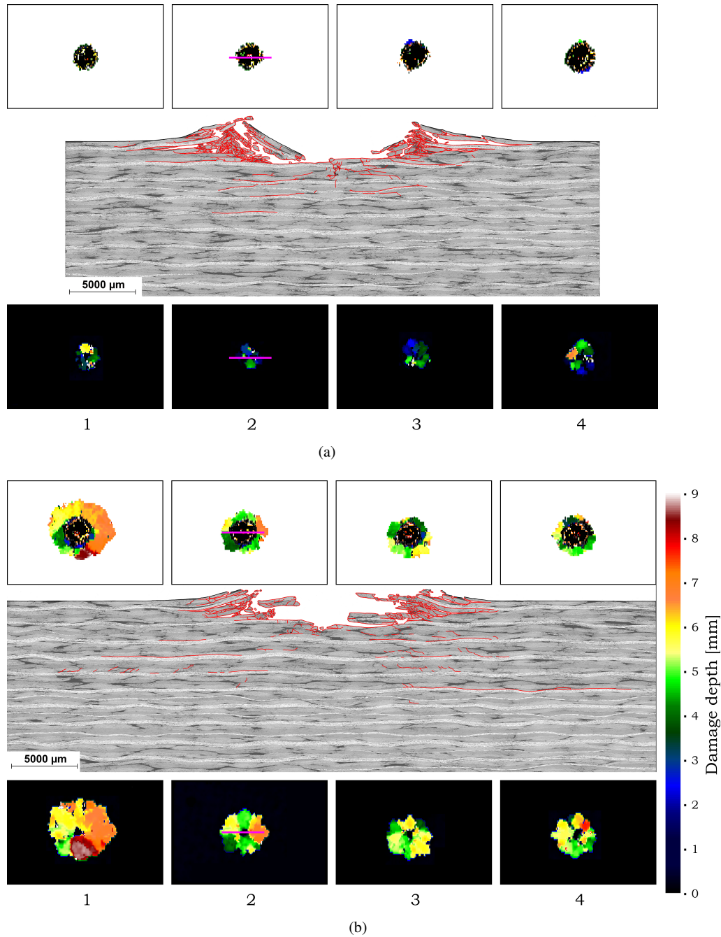
Figure 15. Damage comparison between 100 J (a) drop-weight impacts and (b) gas-cannon impacts on 20 mm thick specimens. In the middle the cross-section of one of the four specimens is shown, 20-QI-LM-100-2 in (a) and 20-QI-SM-100-2 in (b), where the crack boundaries have been highlighted in red. TOF scans are shown for all four specimens, the impact side on top and non-impact side on the bottom.
