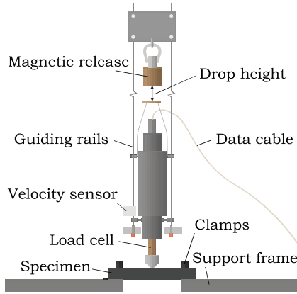
Figure 1. Illustration of the drop-weight setup used for large-mass (LM) impacts.
