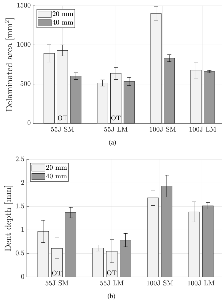
Figure 12. Average impact damage in terms of (a) delaminated area and (b) dent depth for large-mass (LM) drop-weight impacts and small-mass (SM) gas-cannon impacts. Note that the results annotated with OT contain the specimens with an orthotropic layout.
