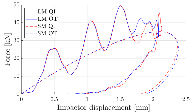
Figure 16. The effect of layup for 55 J large-mass (LM) drop-weight impacts and small-mass (SM) gas-cannon impacts on 20 mm thick specimens.
