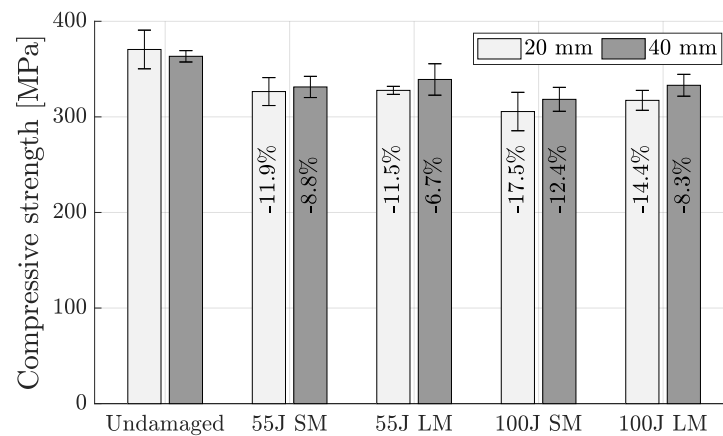
Figure 17. Compressive strength for 20 and 40 mm specimens subjected to large-mass (LM) drop-weight impacts and small-mass (SM) gas-cannon impacts.
