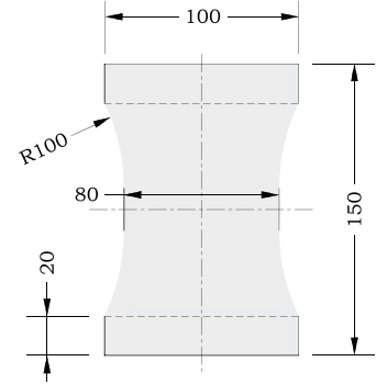
Figure 3. The dog-bone shape used for static compression tests of undamaged specimens.
