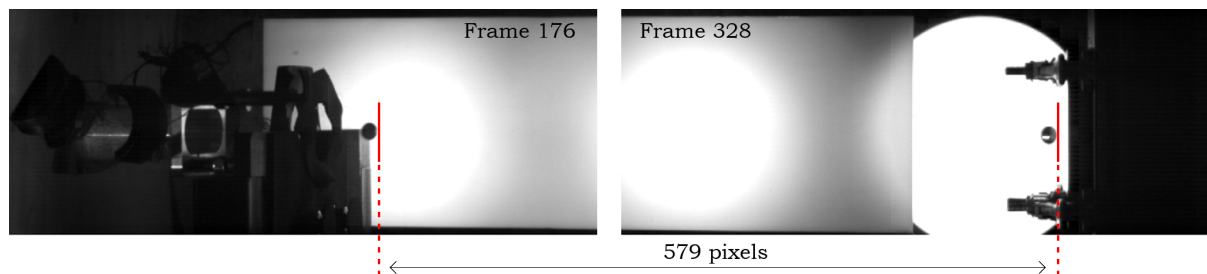
Figure 7. Illustration of the impact velocity determination of a gas-cannon impact on specimen 20-QI-SM-55-1. The impactor is detected at frames 176 and 328, which results in an elapsed time of 7.6 ms over a distance of 579 pixels. Knowing that 1 pixel equals 1.035 mm the resulting impact velocity is 78.87 m/s.
