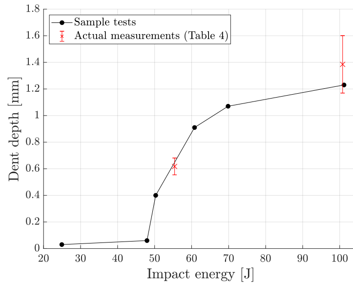
Figure 4. Energy level determination including the dent depths of 55 and 100 J drop-weight impact tests on 20 mm thick QI specimens.
