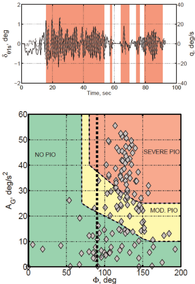
Fig. 30. Example of 'PIO' case - Longitudinal Axis - Pilot inputs and PAC Results.
