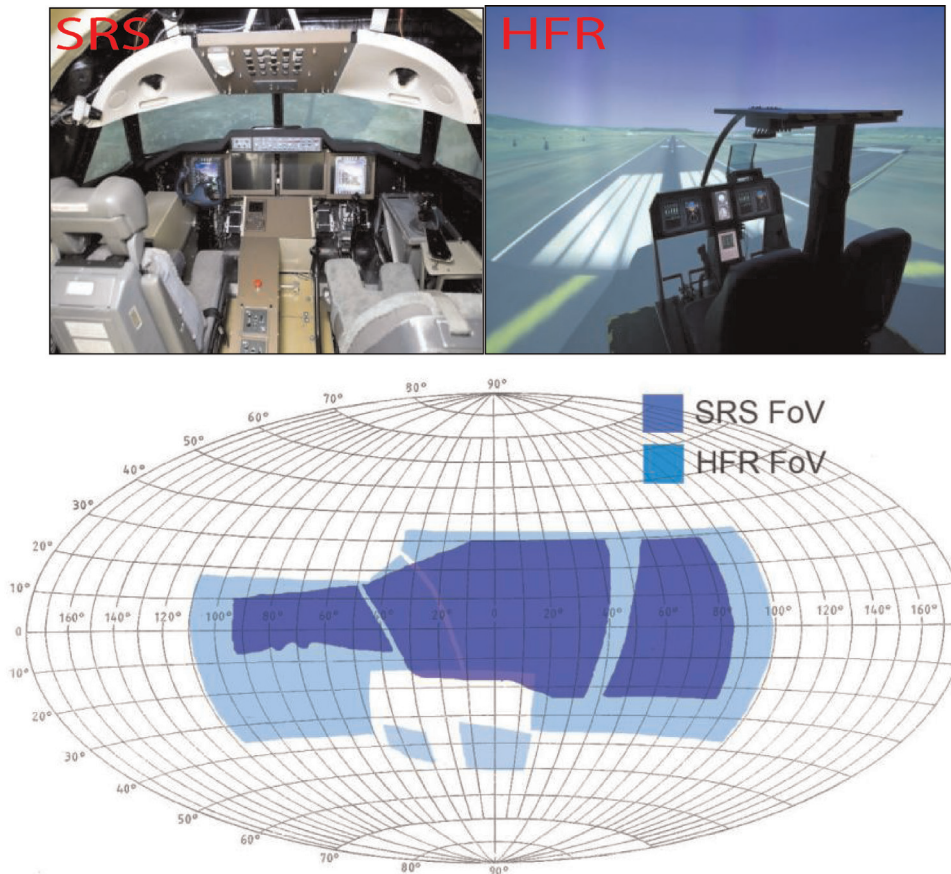
Fig. 15. Pilot view of the outside world from SRS and HFR simulators, right-hand pilot seat.
