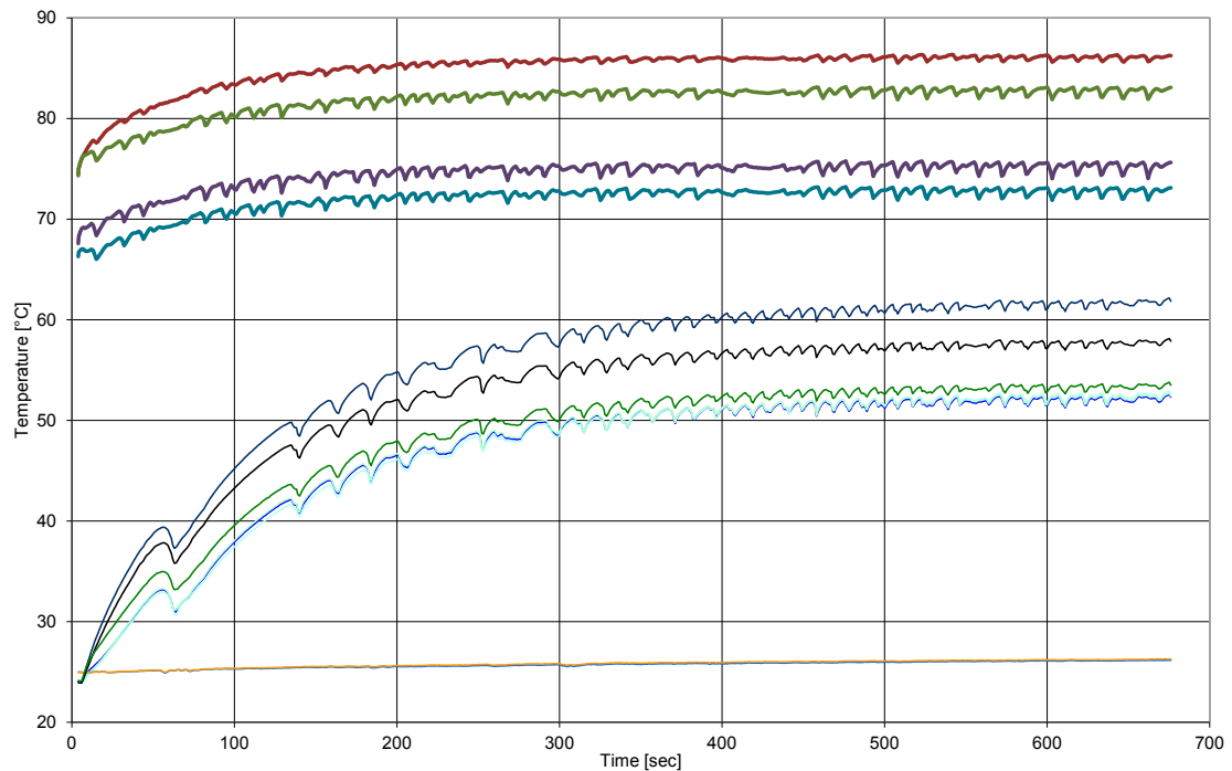
Fig. 3. Measured temperatures of an aircraft cable bundle D=17.5\text{mm} (with braid) in 25^\circ\text{C} air for a 20% above rated currents at 1 bar (4 thick upper lines) and 20% below rated current at 72 mbar (4 thin lines at the middle) at an ambient temperature of 25^\circ\text{C} (lower line).
