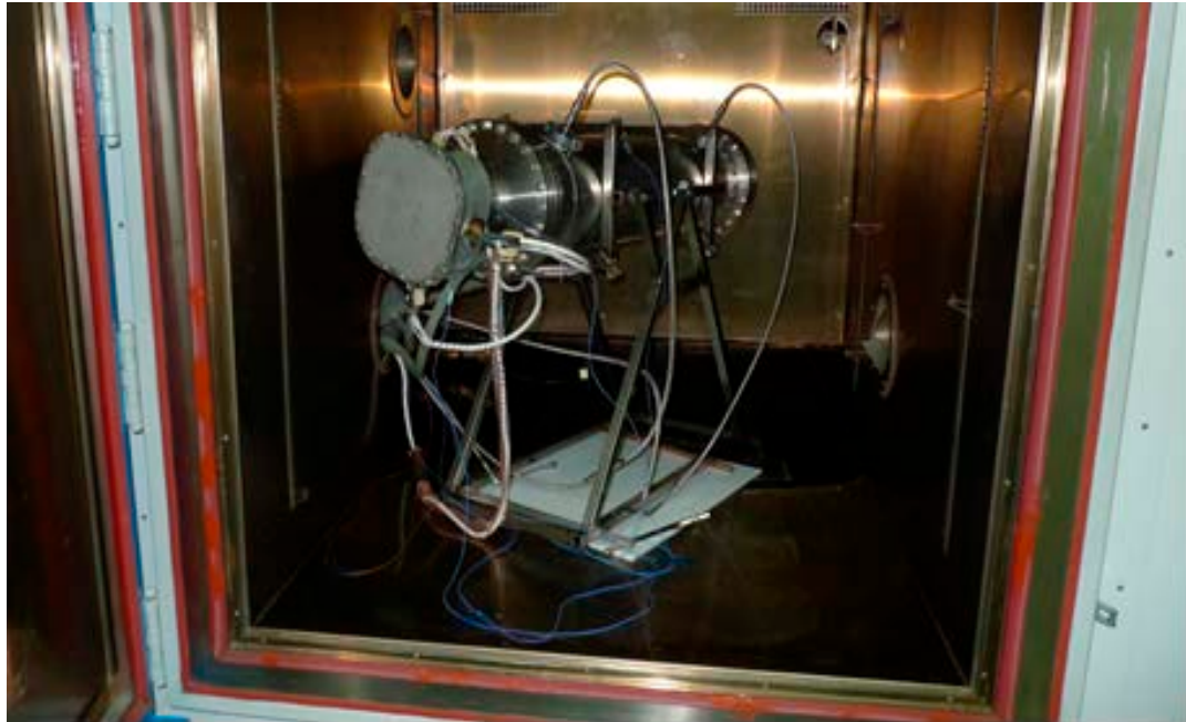
Fig. 1. Photograph of the HDTF for convective environments on a rotatable bench inside NLRs Climate Chamber.
