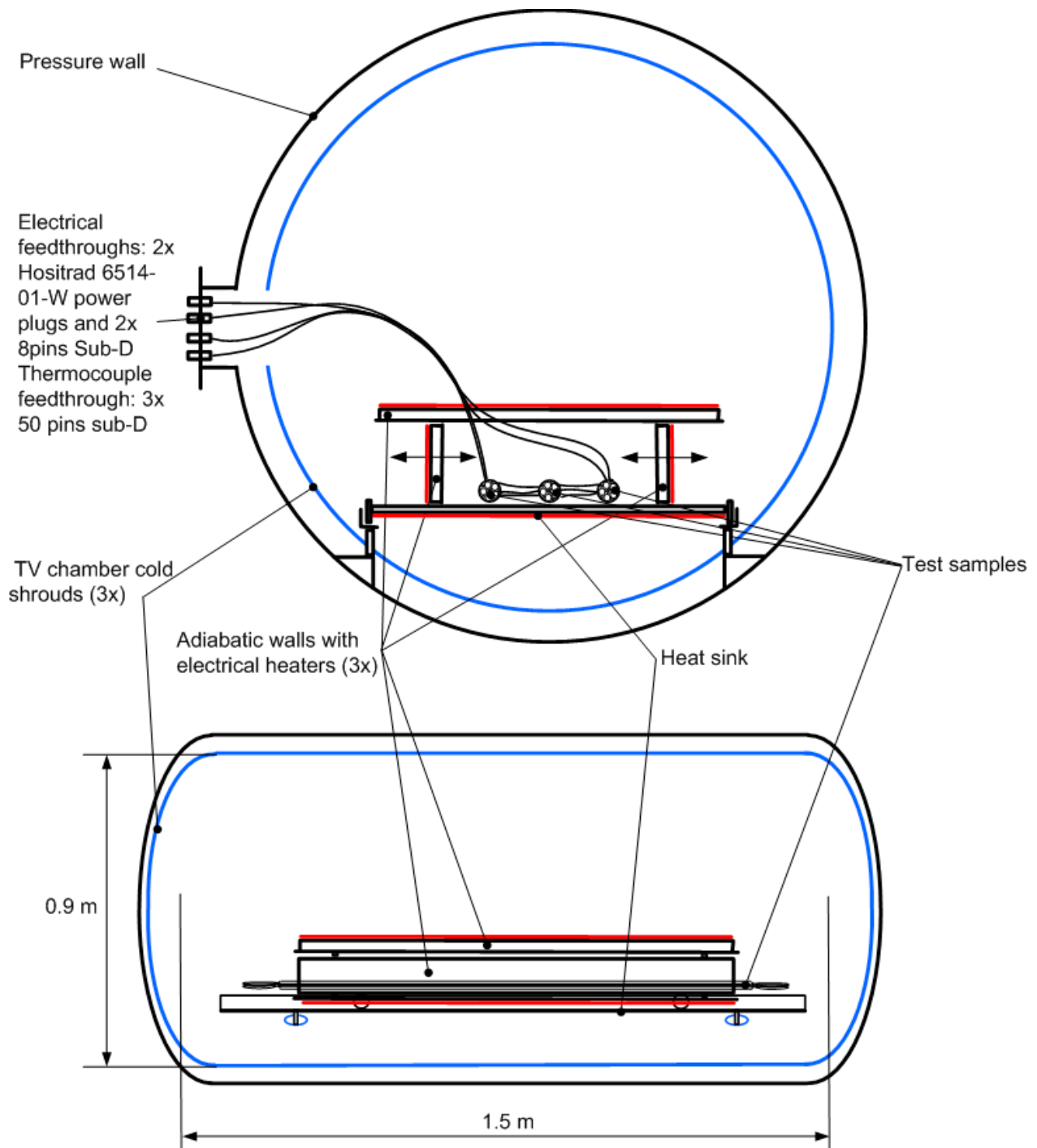
Fig. 5. Cross sections of the proposed HDTF for space environments with a sample bundle suspended in a TV chamber at NLR with adjustable and temperature controlled walls.
