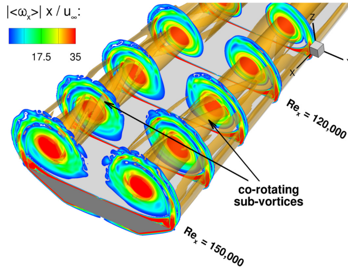
Fig. 19. Axial slices of the magnitude of the time-averaged axial vorticity scaled by the axial location |\langle \omega_x \rangle| x / u_\infty at Re_c = 150,000 computed on the fine computational grid. The iso-surface |\langle \omega_x \rangle| x / u_\infty = 0.29 shows that the time-averaged sub-vortices rotate around the vortex core in the same direction as the flow velocity.
