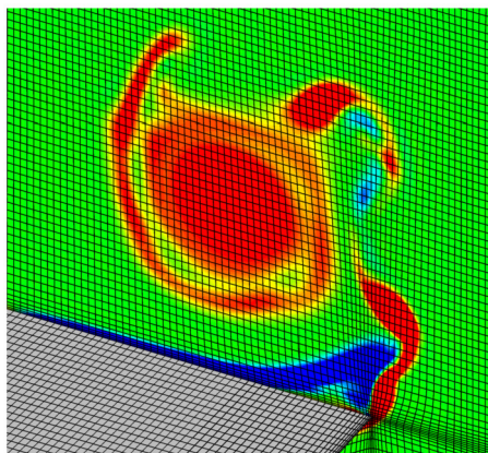
Fig. 6. The coarse mesh on the wing surface and at the axial slice x = 0.8c . Note that the grid is approximately isotropic in the primary vortex.
