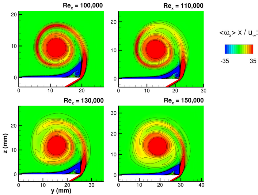
Fig. 20. Slices at several transitional axial local Reynolds numbers of the time-averaged axial vorticity scaled by the axial location \langle \omega_x \rangle x / u_\infty for Re_c = 211,200 as computed on the medium computational grid.
