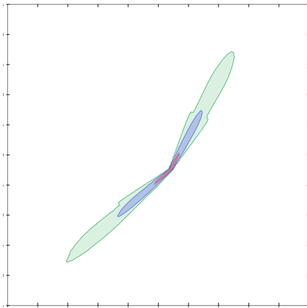
Fig.4 Individual risk contours of a ground-level heliport: 1 \cdot 10^{-5} /year (red), 1 \cdot 10^{-6} /year (blue) and 1 \cdot 10^{-7} /year (green)
