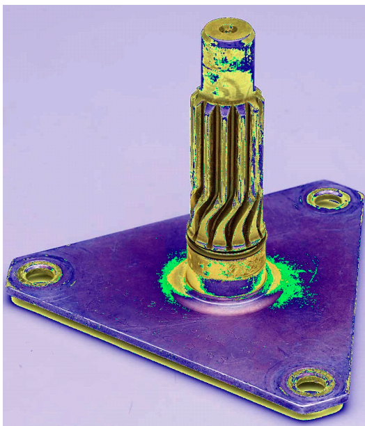
Fig.6 Deformed spline
