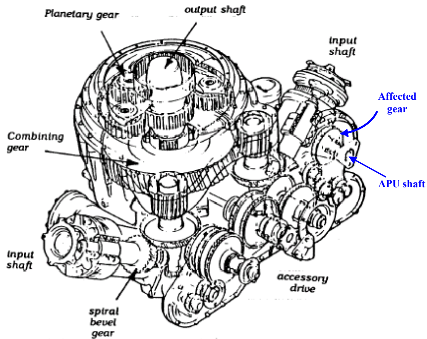
Fig.5 Cutaway view of the AH-64D transmission housing with the affected gear and shaft indicated in blue
