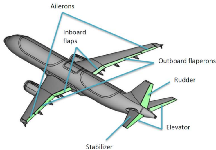
Figure 3 : Flight Control Surfaces of the Scaled Flight Demonstrator
