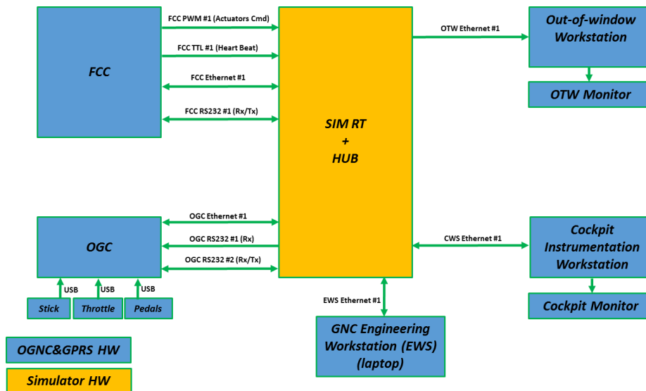
Figure 10 : Overall architecture of the Hardware-in-the-Loop test environment
