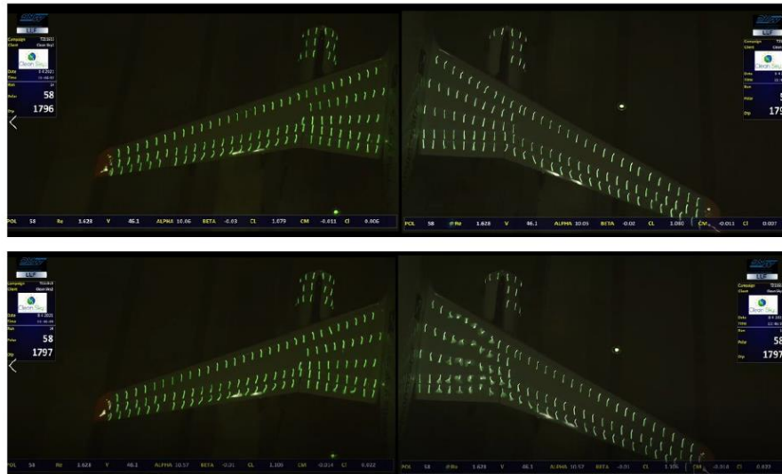
Figure 5 : Tufts visualization on the SFD wing at 46 m/s at 10.06° of Angle of Attack (top) and at 10.57° of Angle of Attack (bottom)
