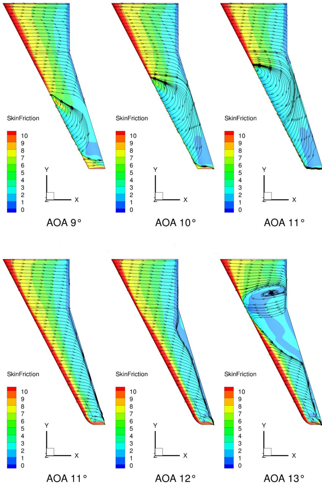
Figure 13 : Wing aerodynamics simulations for the original wing (top) and the redesigned one (bottom)
