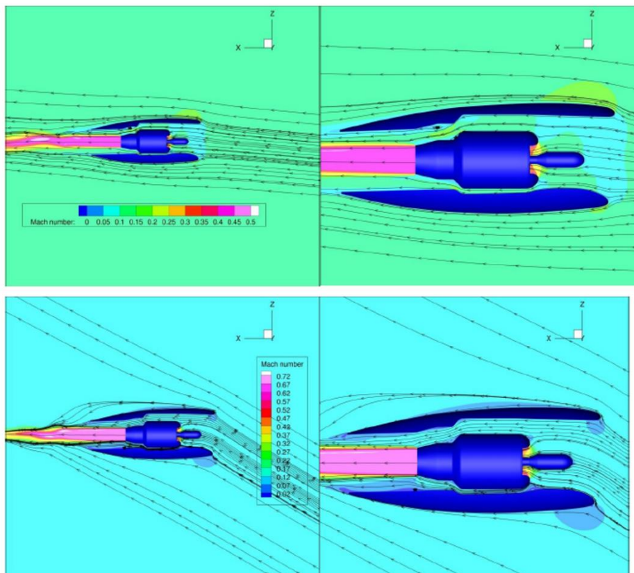
Figure 15 : Revised and final design of the nacelle (cruise condition on top with 5° upwash and take-off condition at the bottom with 30° AOA)
