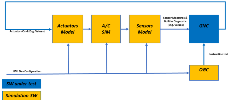
Figure 9 : Offline simulation environment
