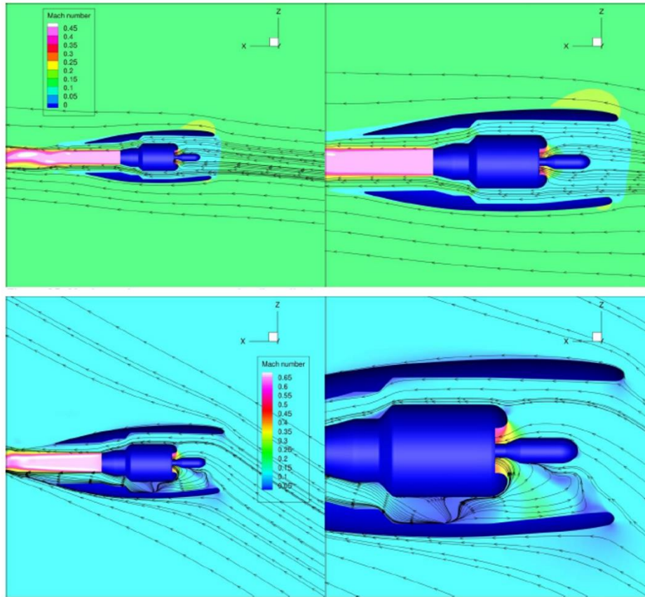
Figure 14 : First design of the nacelle (cruise condition on top with 5° upwash and take-off condition at the bottom with 30° AOA)
