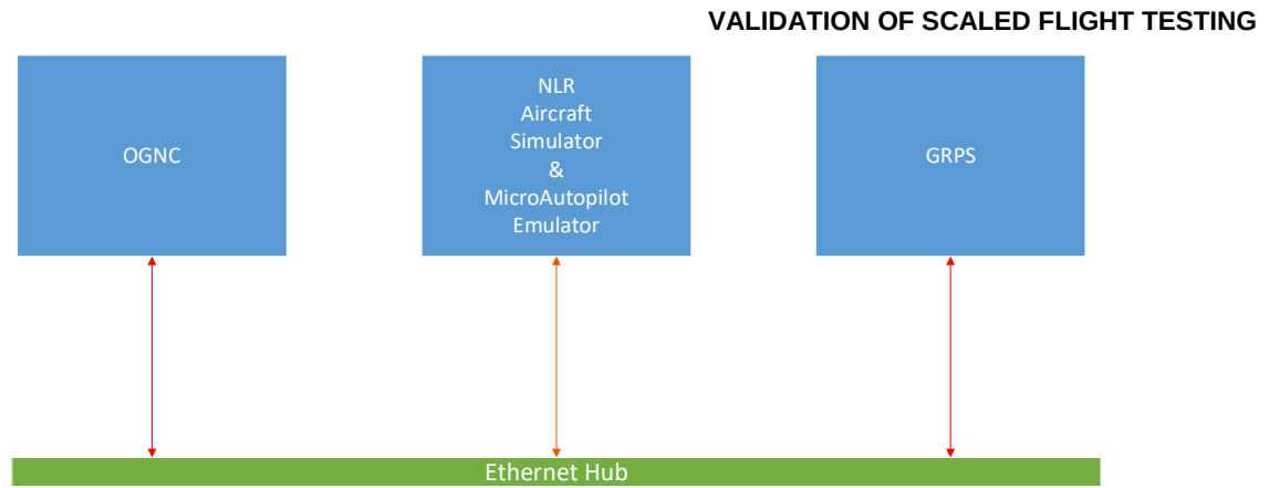
Figure 11 : Architecture of the HW and Pilot in the loop test environment
