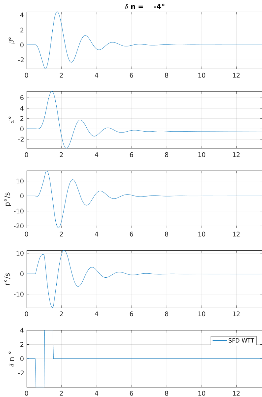
Figure 17 : Responses of the SFD model based on Wind Tunnel Data to a rudder doublet
