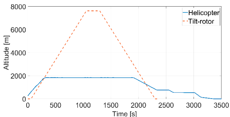
Figure 2: Real helicopter mission vs tilt rotor simulated mission
