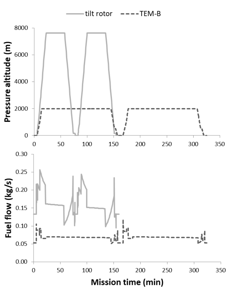
Figure 3: Tilt rotor and TEM-B OAG mission pressure altitude and fuel flow
