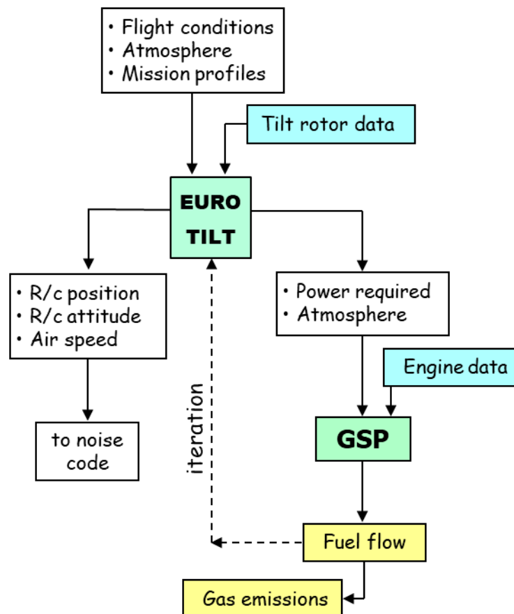
Figure 1: Flow diagram for EURO TILT in combination with GSP and a noise code
