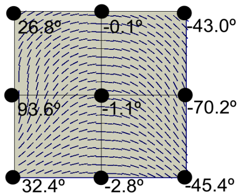
Figure 5: Example of a nine control point field with fibre-angle values of the control points. The vector field is interpolated from these control point locations and values using the spline surface mapping
