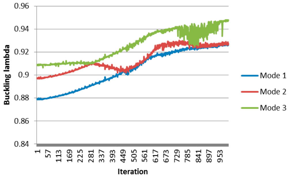
Figure 15: Convergence of mode 1 and 2 for the second local optimization. Initially a larger deviation between the modes is present
