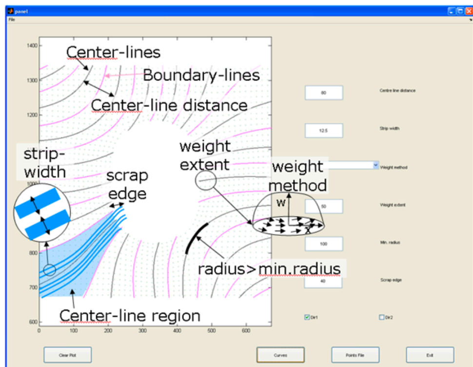
Figure 7: View of the fibre path tool to derive a to be manufactured design from the vector-field
