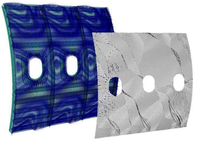
Figure of the fuselage window section with fibre direction vectors depicted on the image to the left. On the figure on the right the variable stiffness optimized fibre path design is shown
