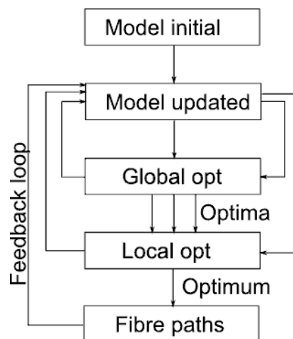
Figure 6: Overview of the optimization and feedback loop. From the global opt. a selection of optima is chosen for the local optimizer. The optimum is analysed with fibre paths and feedback for model update
