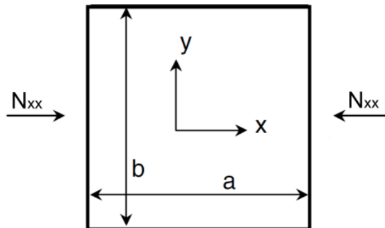
Figure 8: Square plate with simply supported boundary conditions and size of 500 mm (a and b values)
