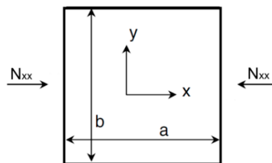
Figure 3: Square plate with simply supported boundary conditions and size of 500 mm (a and b values)
