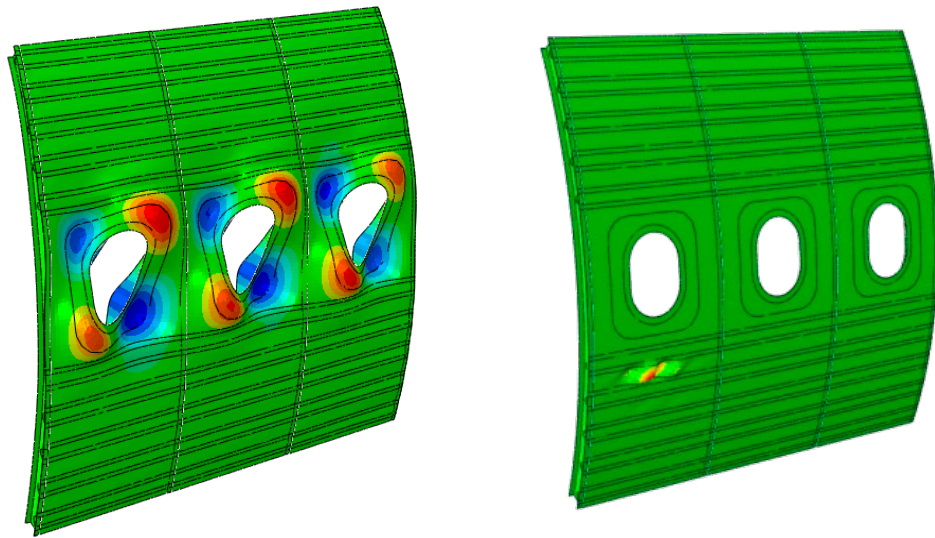
Figure 14: Common buckling modes found in the analyses, window buckling mode (left) and stiffened panel mode (right)
