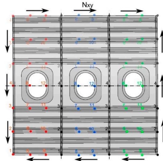
Figure 13: Illustration of the control points used with symmetry and repetition. The shear load N_{xy} applied to the section is shown
