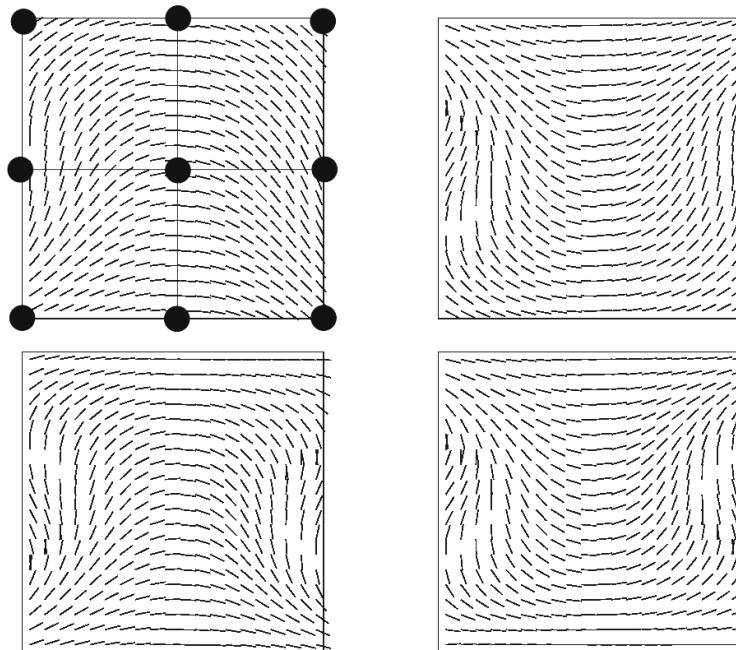
Figure 10: Optimized result of the flat plate buckling for the four ply-pairs. In the upper-left example the nine control points are shown. The orientation vector per element is shown of the optimized result
