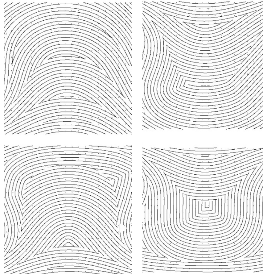
Figure 11: Fibre path designs for the four ply pairs of the optimized flat plate
