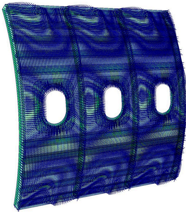
Figure 16: Variable stiffness orientation in the skin of the fuselage side section. The symmetry around the window frames and the repetition between the frames can be observed
