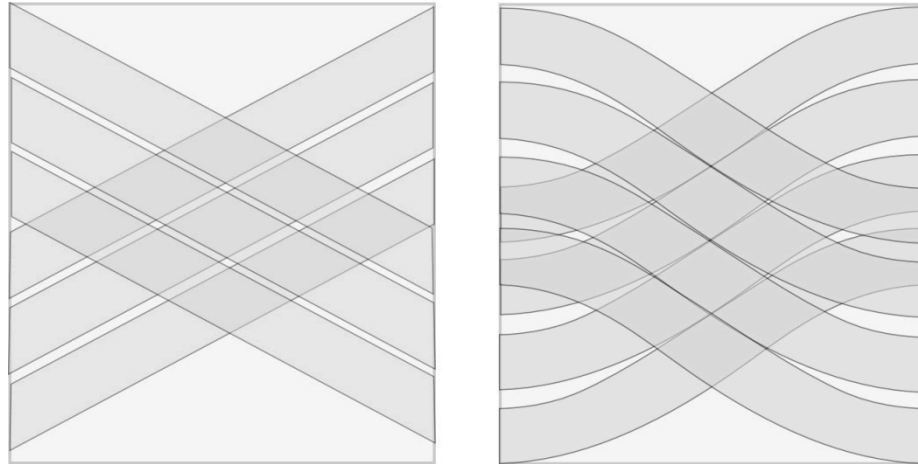
Figure 2: Illustration of composite fibre direction for a conventional constant stiffness laminate (left) and variable stiffness laminate (right)
