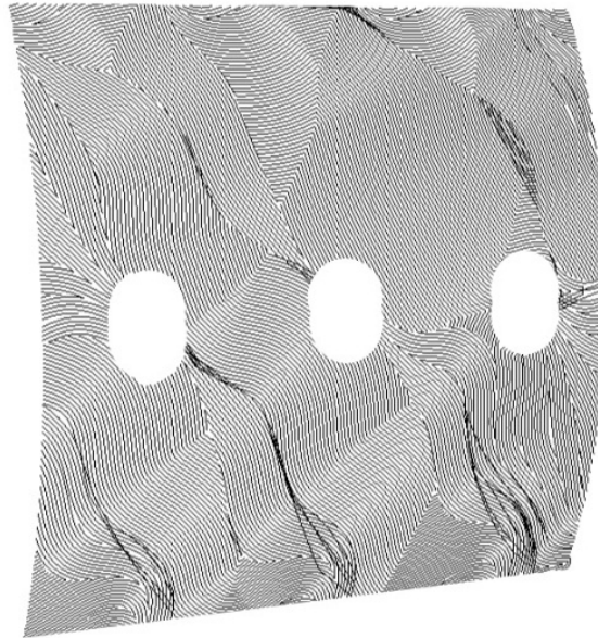
Figure 17: Fuselage window section fibre paths in the skin
