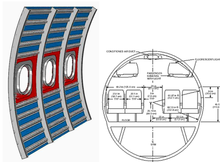
Figure 12: Fuselage window section with frames, stringer and window frames on the left. The skin thickness is lower in the area indicated by blue. On the right an illustration of a fuselage cross-section
