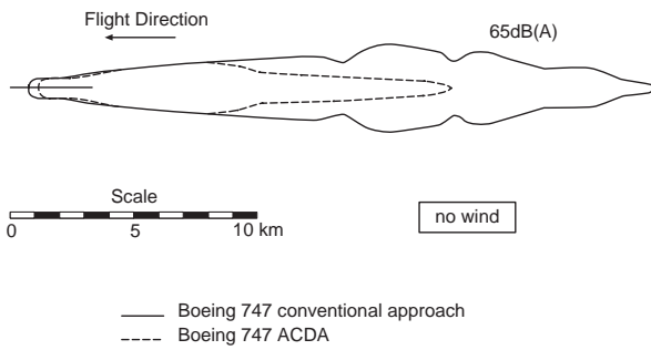
Fig. 8b Comparison of Boeing 747 noise footprints [65 dB (A)] for conventional approach and ACDA
