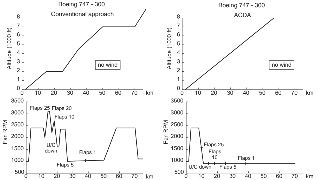
Fig. 8a Comparison of Boeing 747 engine RPM for conventional approach and ACDA
