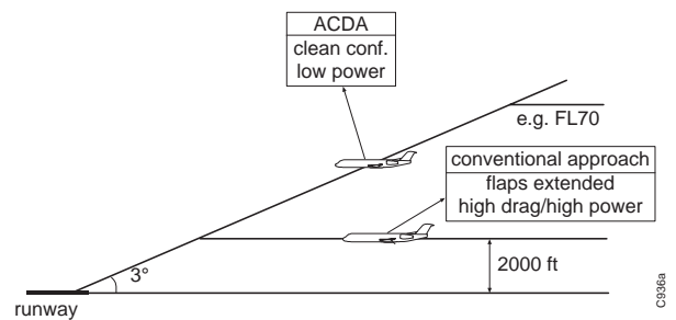
Fig. 7 Comparison of vertical profiles for conventional approach and ACDA
