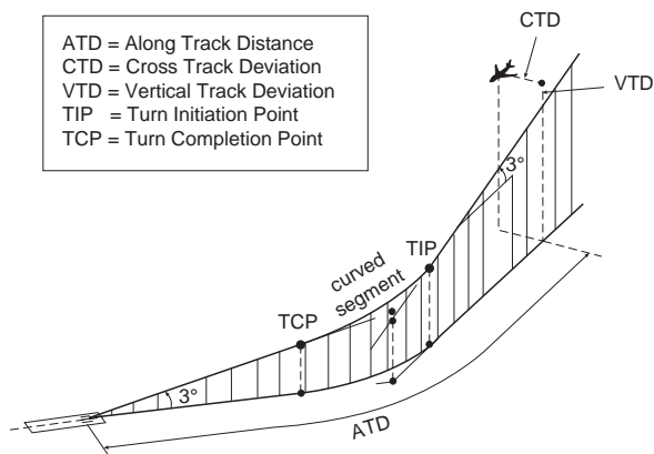
Fig. 6 Definition of aircraft position along a curved approach path
