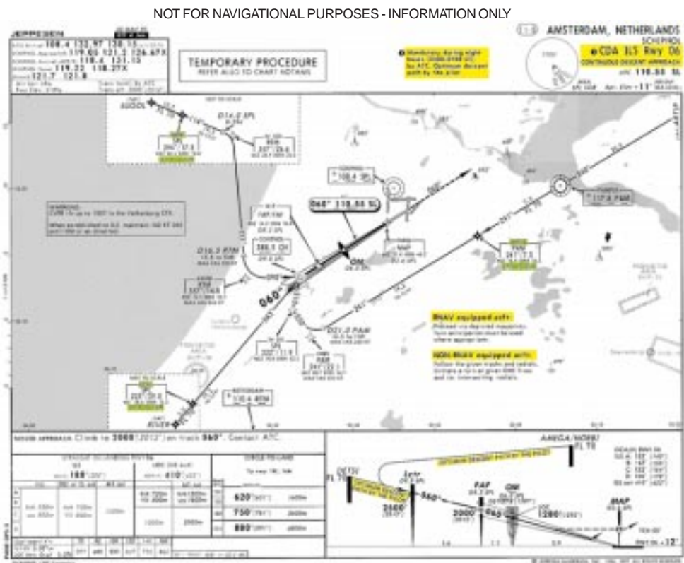
Fig. 3 Approach plate for CDA on ILS runway 06
