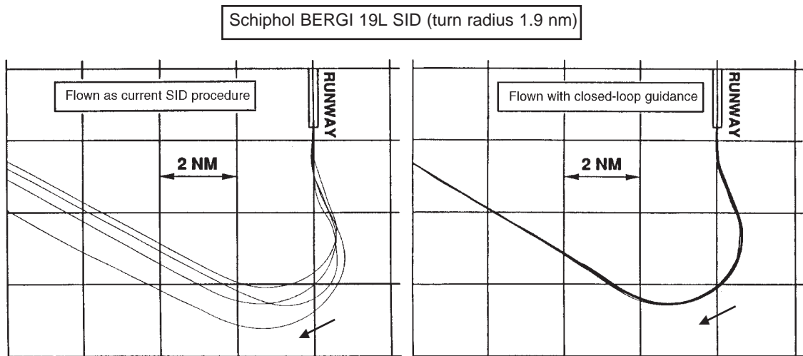
Fig. 10a Comparison of flight simulation results between current and closed-loop guided SID's
