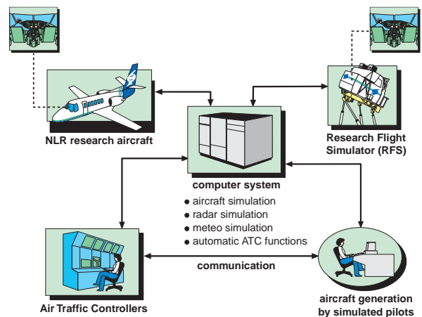
Fig. 11 Possible communications between different NLR research facilities
