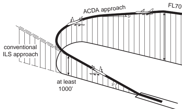
Fig. 5 ACDA concept
