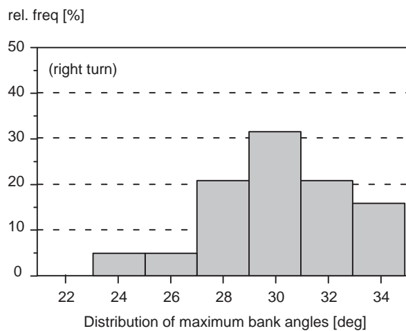
Fig. 10b Histogram of maximum bank angles during the turn of the closed-loop BERGI SID
