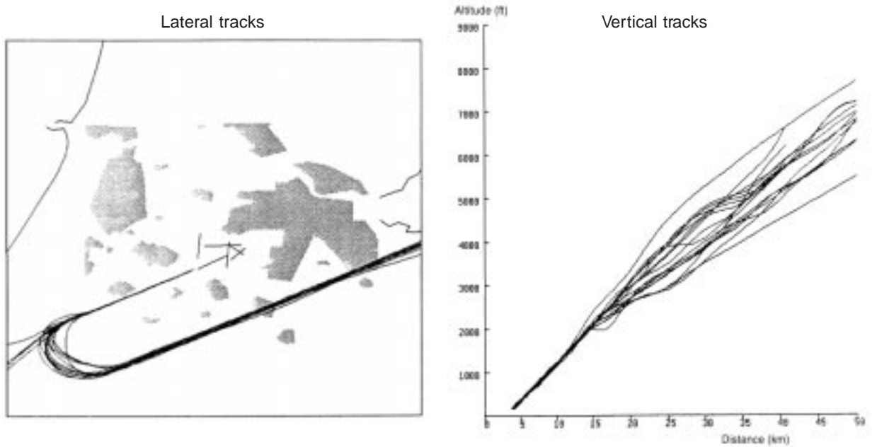
Fig. 4 Lateral and vertical track plots for the AMEGA CDA (source: "Op de bok", aug '96)
