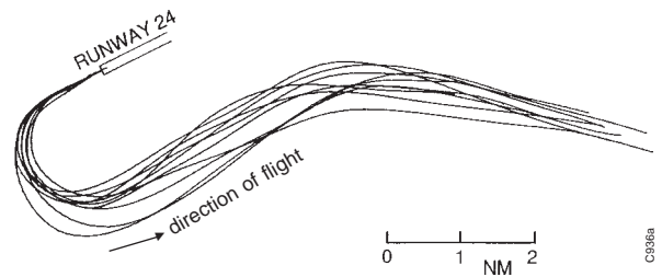
Fig. 9 Recorded Fanomos tracks for actual Boeing 747 departures from Schiphol runway 24
