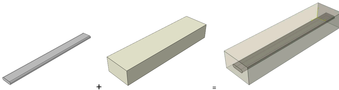
Figure 4: Overview of adding the carbon fibre geometric representation on the left to the nylon ‘host’ material in the middle. The result is a combined material using independent meshes
