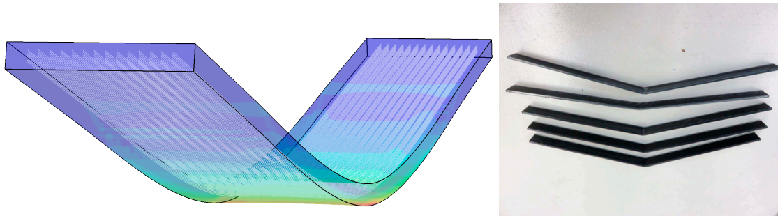
Figure 12: bending simulation using the independent mesh approach showing the strain. On the bottom there is a tensile strain as expected. On the right the failure bending coupons
