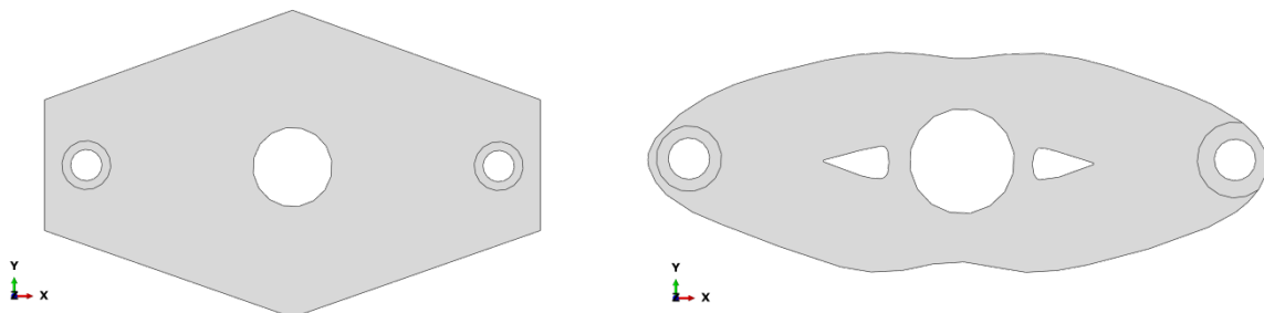
Figure 13: Topology optimization of the geometry on the left. The optimized design is shown on the right. For the topology optimization the Abaqus Tosca is used
