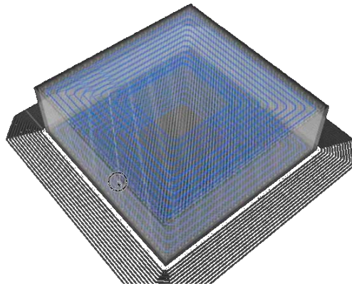
Figure 6: Example from the web-based Eiger tool to design the fibre paths per layer (in blue)
