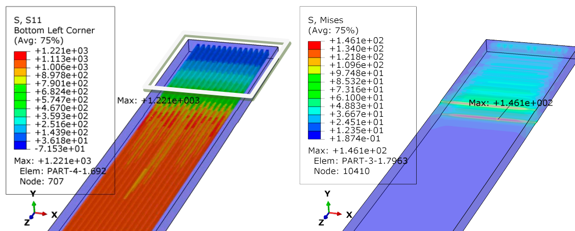
Figure 11: On the left the stress in the carbon fibre yarns with the support region indicated and on the right only the nylon host stress values. At some point in the nylon plasticity will occur which is not included in this simulation
