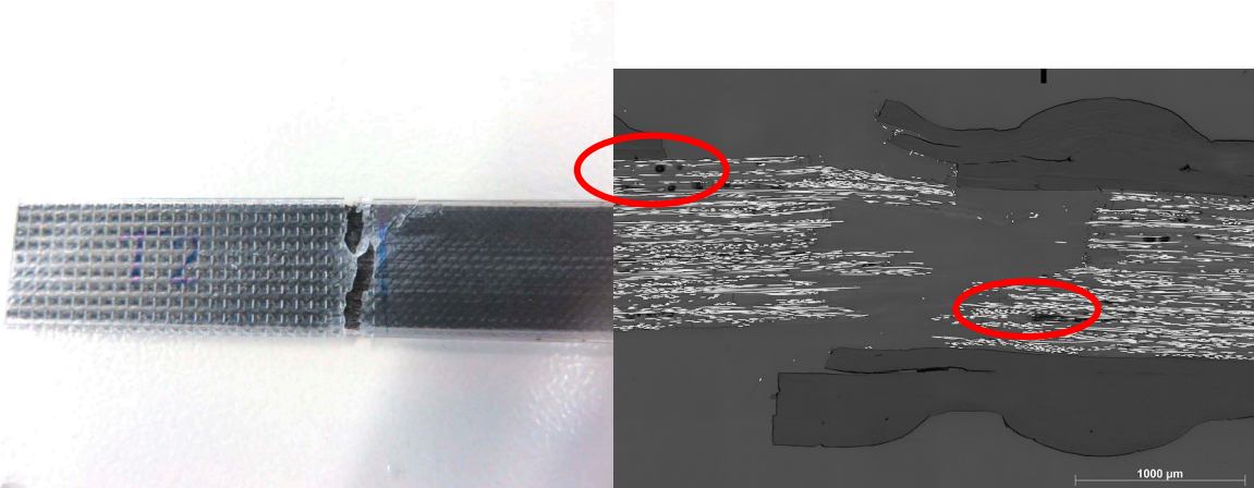
Figure 9: Failure mode of the tensile T2 coupon and micro structure cross section view of the failure mode. The nylon floor and top layers can be identified. Also significant void areas are observed in this cross section indicated in red
