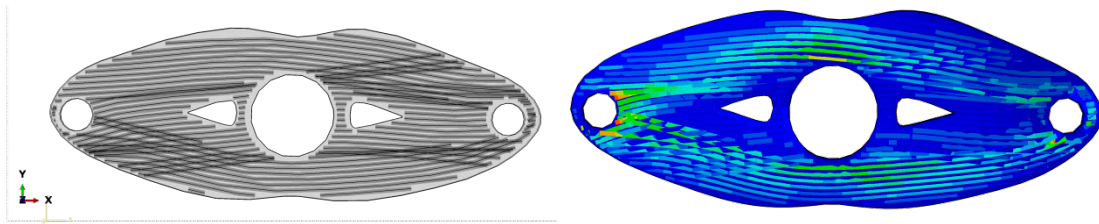
Figure 14: Optimized design with fibre steering for 3D printing. The finite element results on the right shows the independent mesh method on this design
