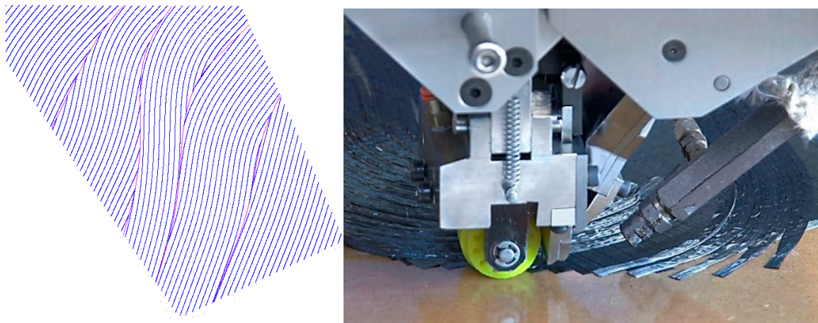
Figure 2: On the left the fibre steered design for a business jet horizontal stabilizer investigated in the TAPAS2 project [1], [2] . On the right the use of fibre steering on the composite fibre placement machine at NLR
