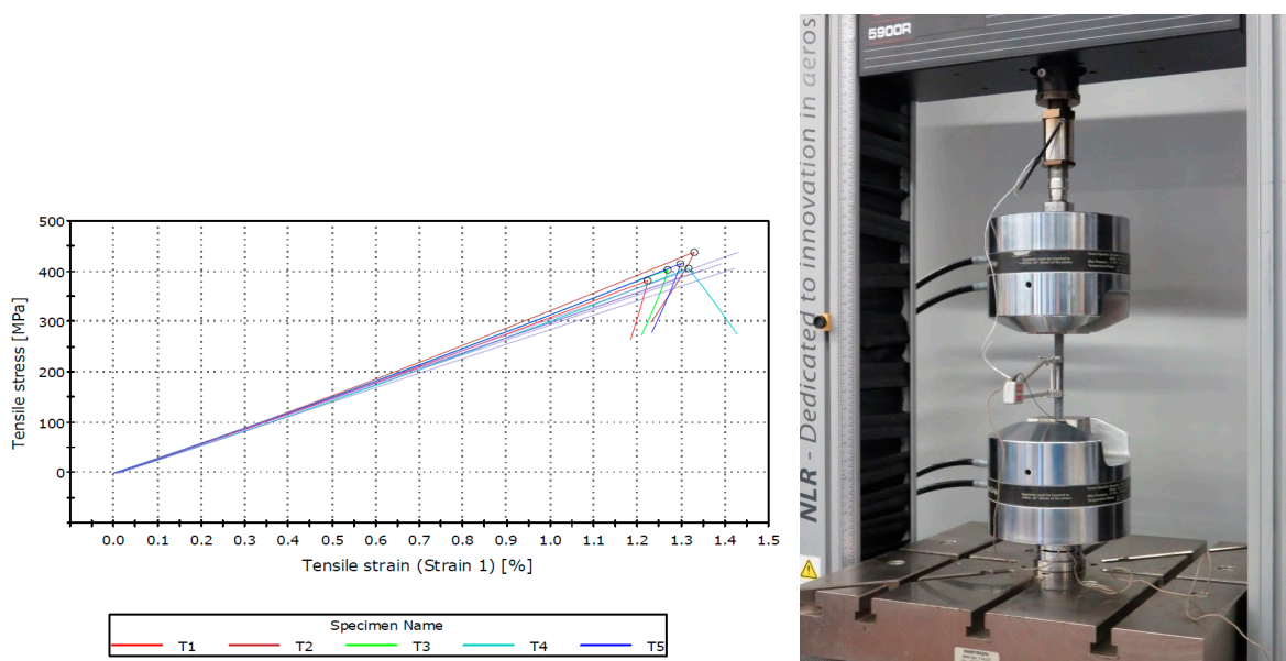
Figure 8: Results of the tensile tests for five coupons and test setup on the right
