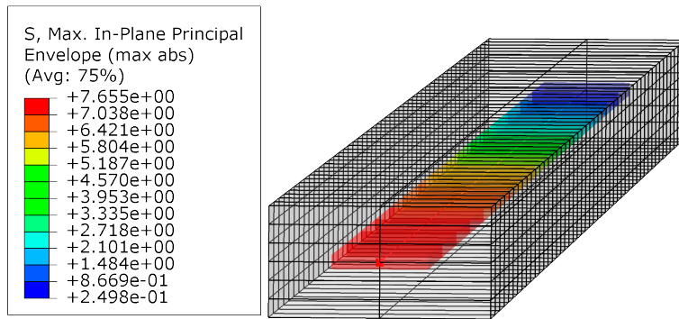
Figure 5: Mesh independent numerical model for a carbon fibre reinforced 3D printed example on one fibre. The loads are indicative. The coloured lines indicate the stress in the carbon fibres modelled as beam elements with a tension load in fibre direction
