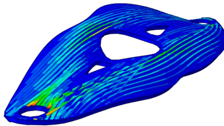
Figure 15: 3D view on the part with bending observed caused by the offset of the fibres in the nylon material
