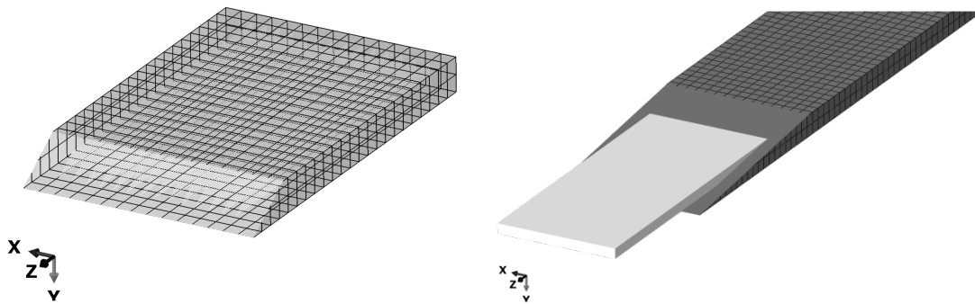
Figure 10: Finite element model of the coupon geometry with the nylon host geometry and the 112 individual carbon yarns
