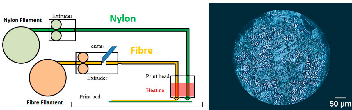
Figure 3: Schematic of the Mark Two ® 3D printer using a nylon base filament and continuous fibre filled filament. These are combined on the print bed. On the right a cross section of the carbon fibre filled filament where the low fibre volume fraction of 34.5% can be observed
