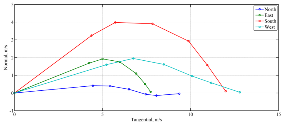
Figure 2 Measured (mean) wind components for wind originating from different wind-rose directions for an entire year. The circular markers show an increasing height at intervals of 0, 10 100, 300, 600 1000 and 2000 m.
