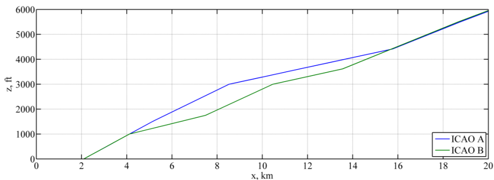
Figure 1 Modeled climb profile for B737
