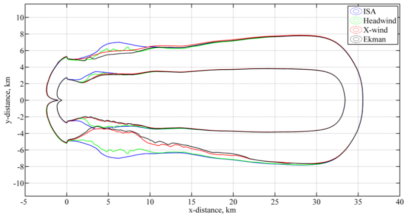
Figure 4 The 65 SEL and 55 SEL contours for the ICAO B procedure.
