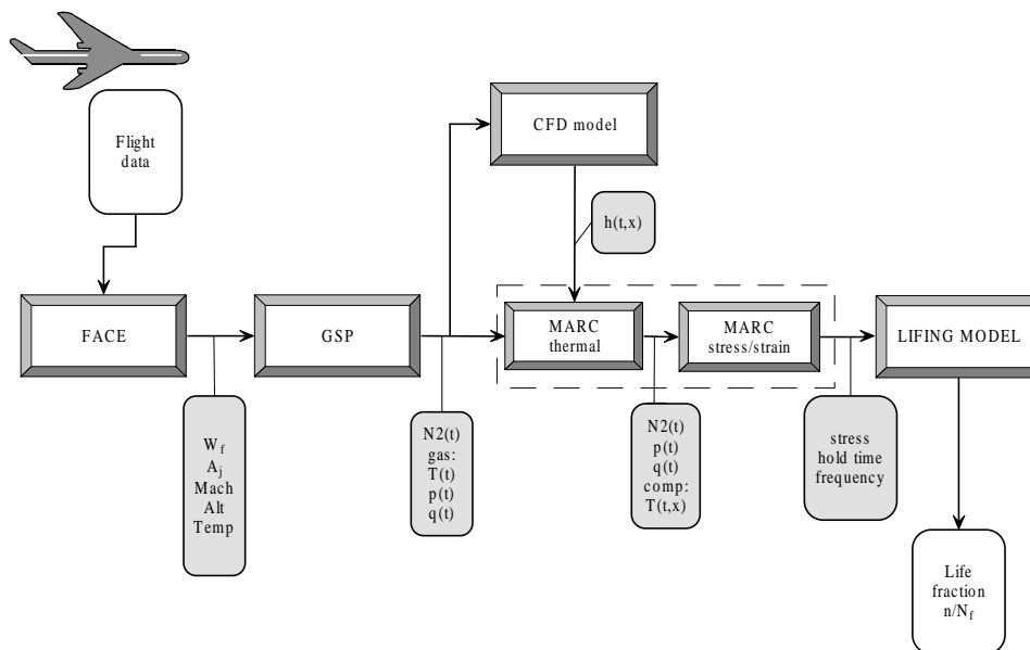
Figure 1: Schematic overview of the integrated analysis tool.
