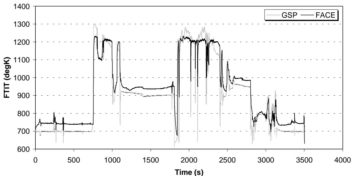
Figure 7: Comparison of FTIT as measured by FACE and calculated by GSP.
