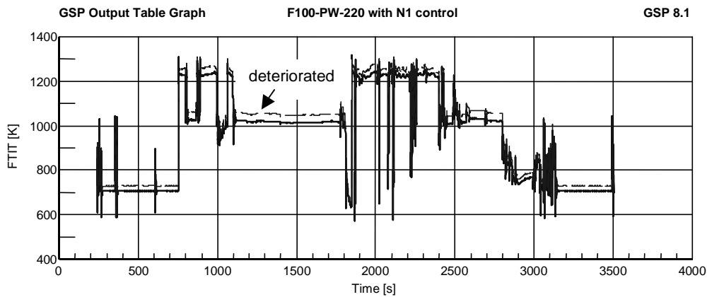
Figure 6: Effect of HPT deterioration on fan turbine inlet temperature FTIT.
