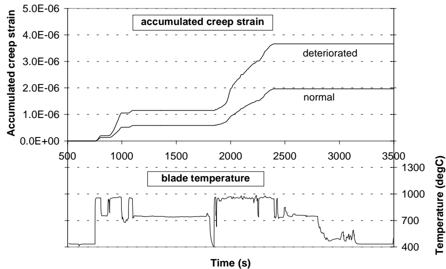
Figure 8: Effect of HPT deterioration on creep strain accumulation.
