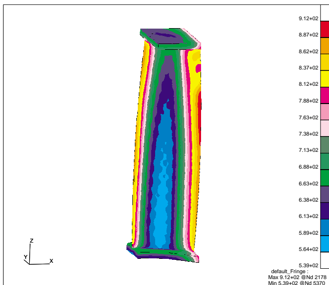
Figure 3: Temperature distribution (°C) in a turbine blade.
