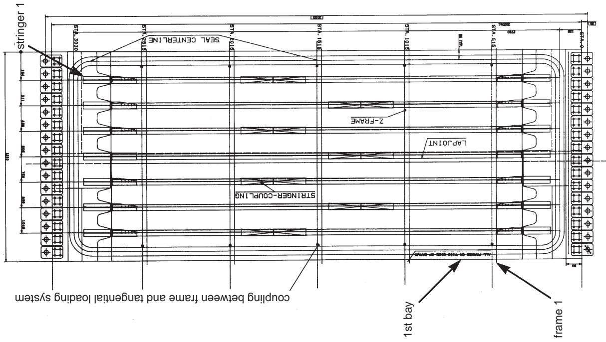
Figure 4 GLARE panel
