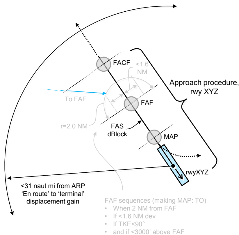
Figure 2-17: FAF special sequencing conditions
