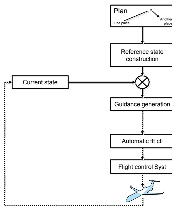
Figure 2-6: Aircraft generalized navigation function
