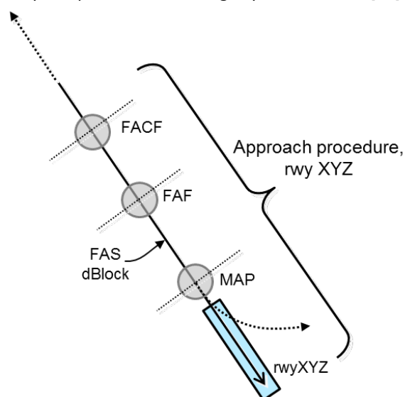
Figure 2-8: Approach - key elements
