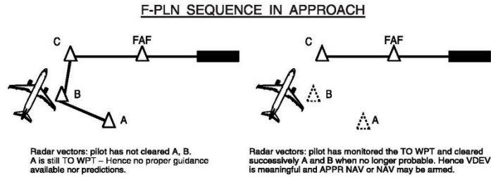
Figure 2-3: Airbus lateral intercept FMS path (all types)
