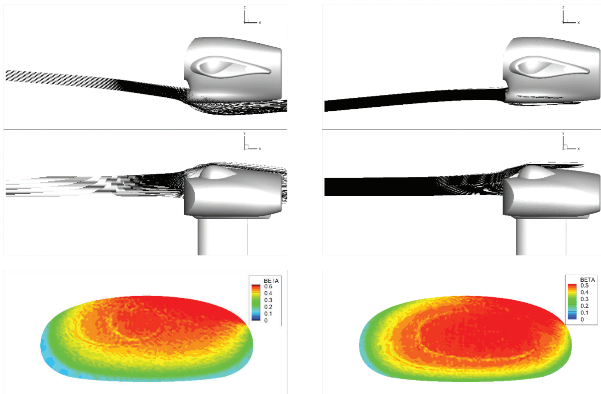
Figure 3 Droplet trajectories (top) and catching efficiency field inlet plane (bottom) for cruise condition ID#1 (left) and holding condition ID#3 (right)
