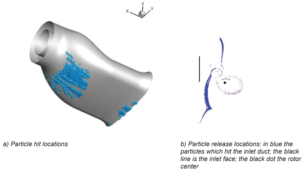
Figure 8 Droplet impingement for ground operations
