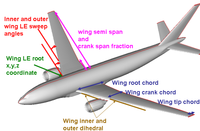
Fig. 1 Geometric design parameters of the wing planform as used in the multidisciplinary analysis system. Besides these parameters, also other parameters, like the positions of wing control surfaces, wing tanks and landing gears, can be varied in the multidisciplinary analysis system.
