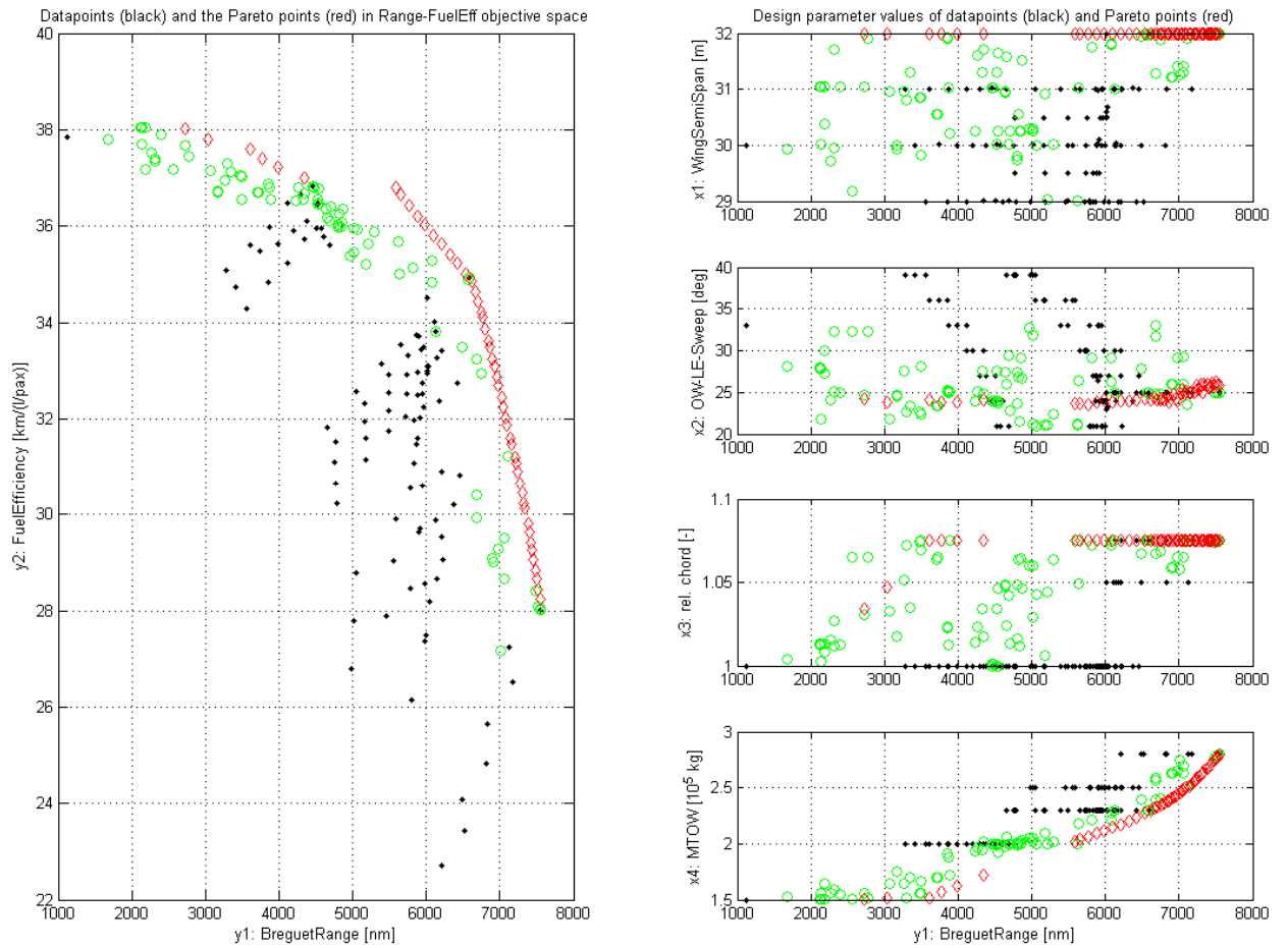
Fig. 5 Design points of data set (black dots), population after 3 generations (green circles), and Pareto front after 100 additional generations (red diamonds) for maximum range versus maximum fuel efficiency found with the kriging-linear-Gauss and kriging-constant-Exponential meta-models, respectively, for range and fuel efficiency. Results presented in objective space (left) and in the range-parameter sub-spaces (right) for each of the four design parameters.
