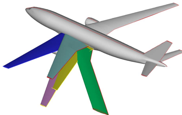
Fig. 2: Illustration of several different wing geometries (coloured left wing), as generated by the multidisciplinary analysis system with various values for wing span, sweep angle and chords. Also illustrated are the fixed geometries for fuselage and empennages.
