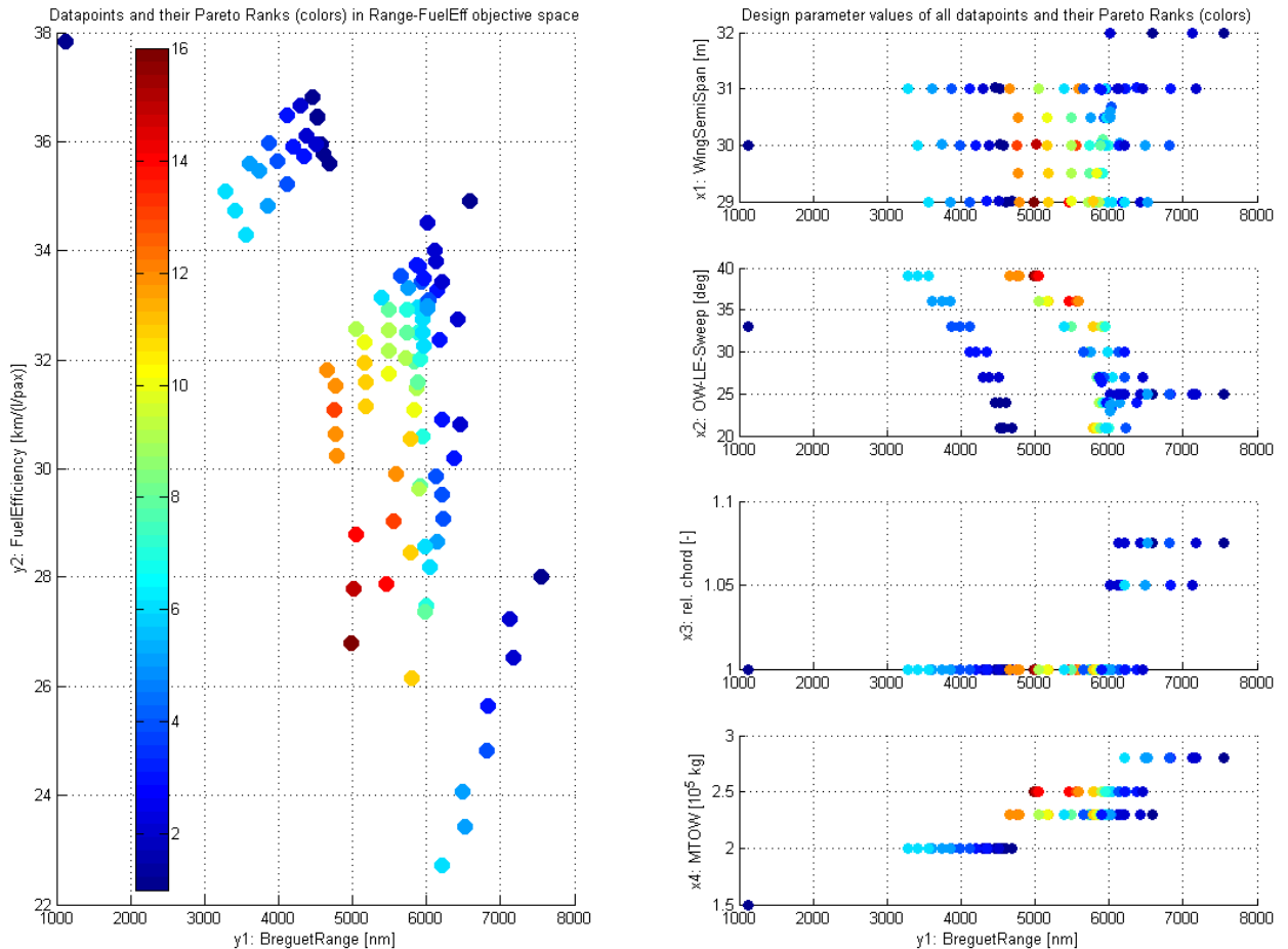
Fig. 4 The range and fuel results in the 99 design points in objective space (left) and in parameter space (right), coloured by their Pareto rank.
