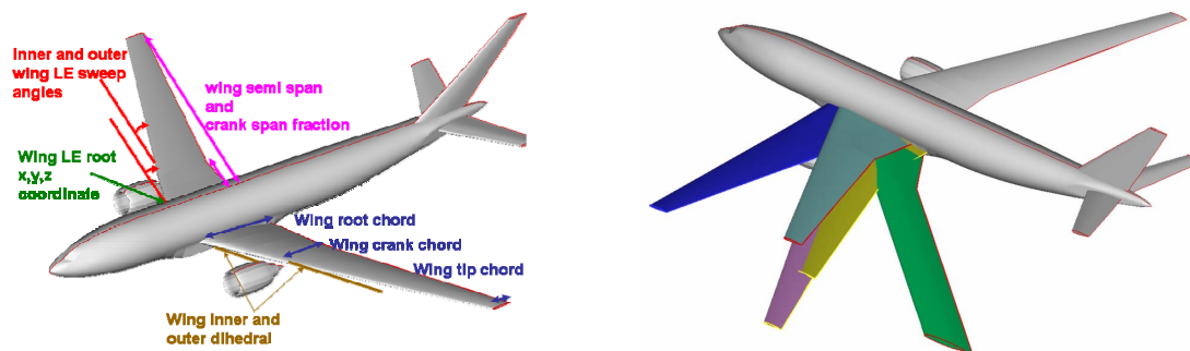
Wing design parameters (left) and aircraft wing geometry variations (right).
