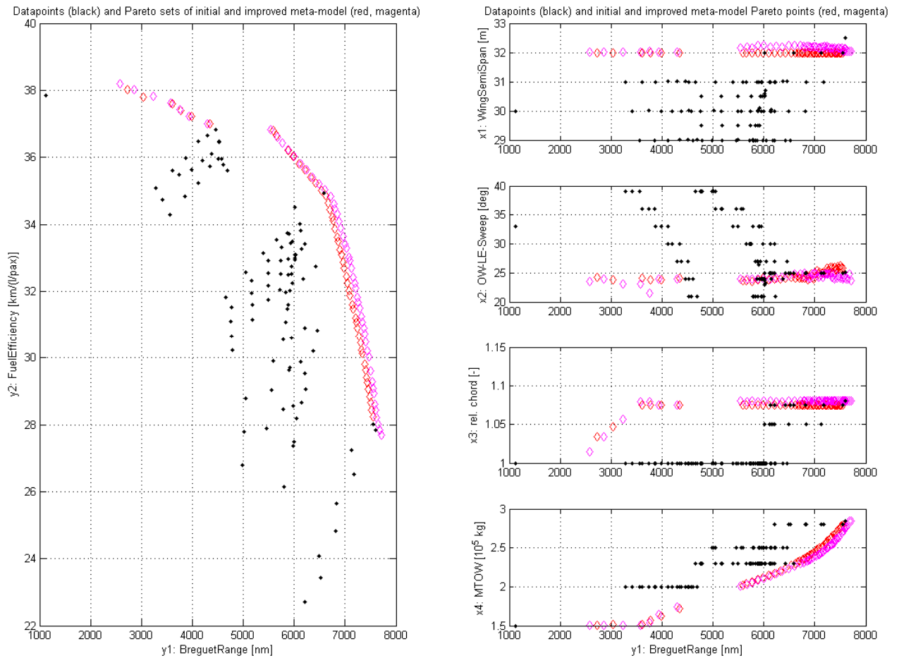
Fig. 7 Pareto fronts found with the initial meta-models (red diamonds) and the improved meta-models (magenta diamonds).
