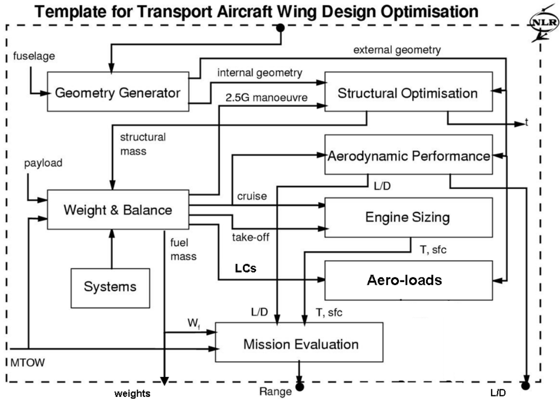
Fig. 3: Schematic overview of the multidisciplinary analysis system. The data communication among the different analyses, as indicated by the arrows, takes place through a single central database (the integrated design model).
