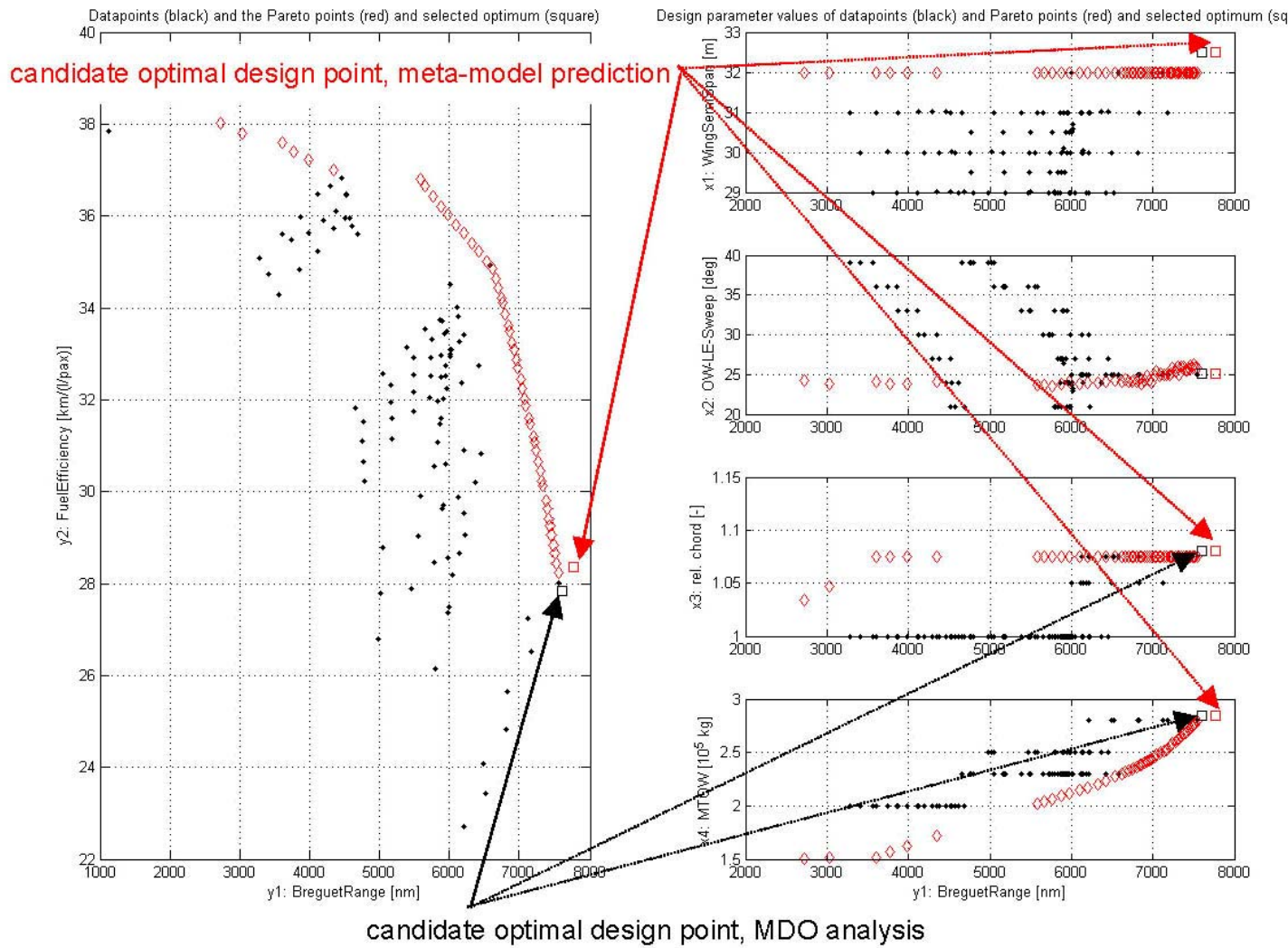
Fig. 6 Pareto front found with initial meta-model (red diamonds), data set (black dots), and MDO analysis and meta-model predictions for candidate optimal design point (black and red squares).
