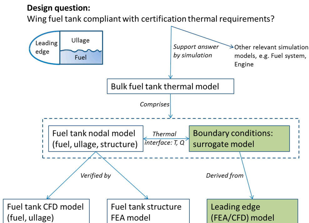
Figure 3: Model coupling and relation scheme of the fuel tank thermal analysis. The models in the green blocks will be further detailed in this paper (see section 5)
