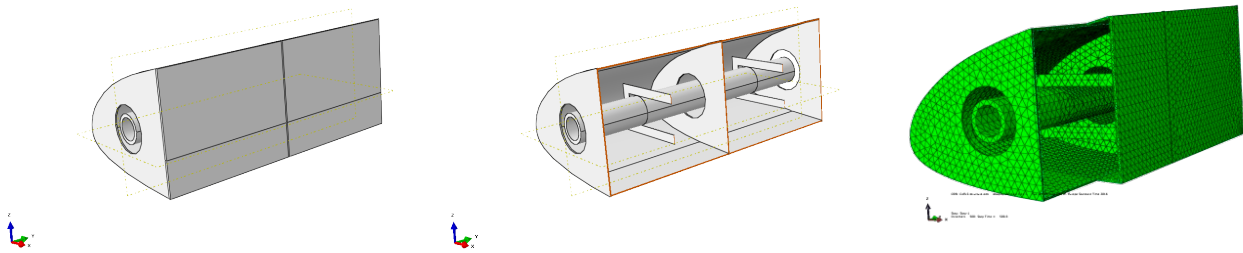
Figure 12: Wing structure part for which an FEA model is created. Left: the closed wing leading edge. Middle: a cut-out to show the internal structure showing the ribs, bleed pipe and bleed pipe supports. Right: the finite element mesh of the leading edge structure, bleed pipe and supports. Via a cut-out the internals are shown
