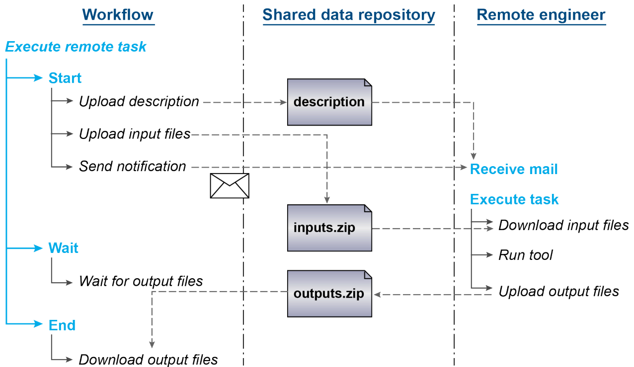
Figure 5: Simplified sequence diagram of the Brics single-task protocol
