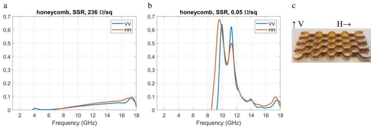
Figure 10: Measured absorption (A) of honeycomb with SRR in carbon ink (236 \Omega /sq) (a) and in silver ink (0.05 \Omega /sq) (b). The polarization is indicated in (c).
