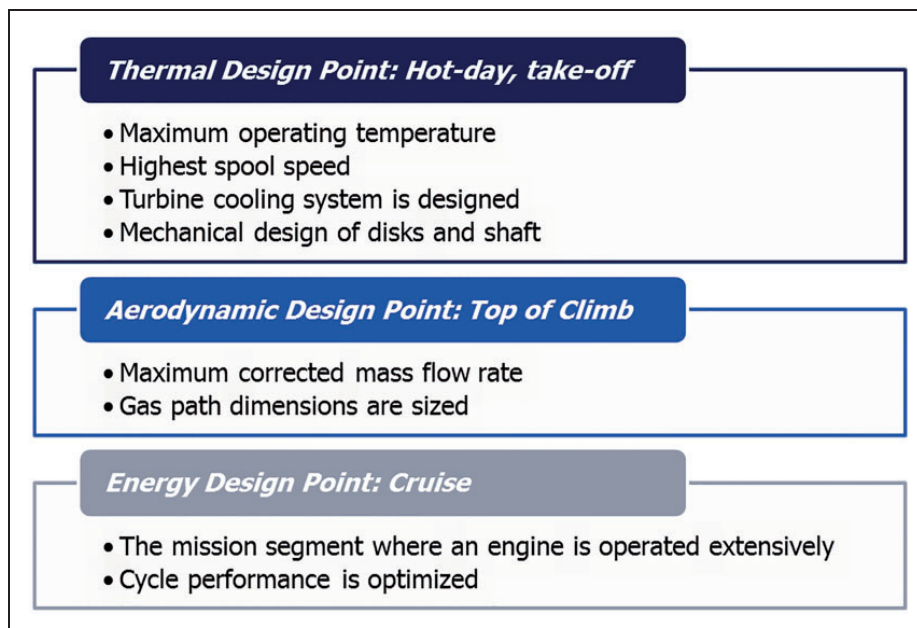
Figure 9. Various engine design conditions. 36
