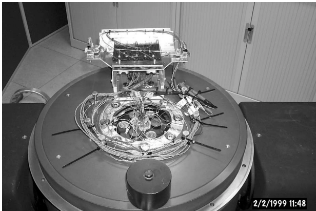
Figure 10 High-acceleration set-up
