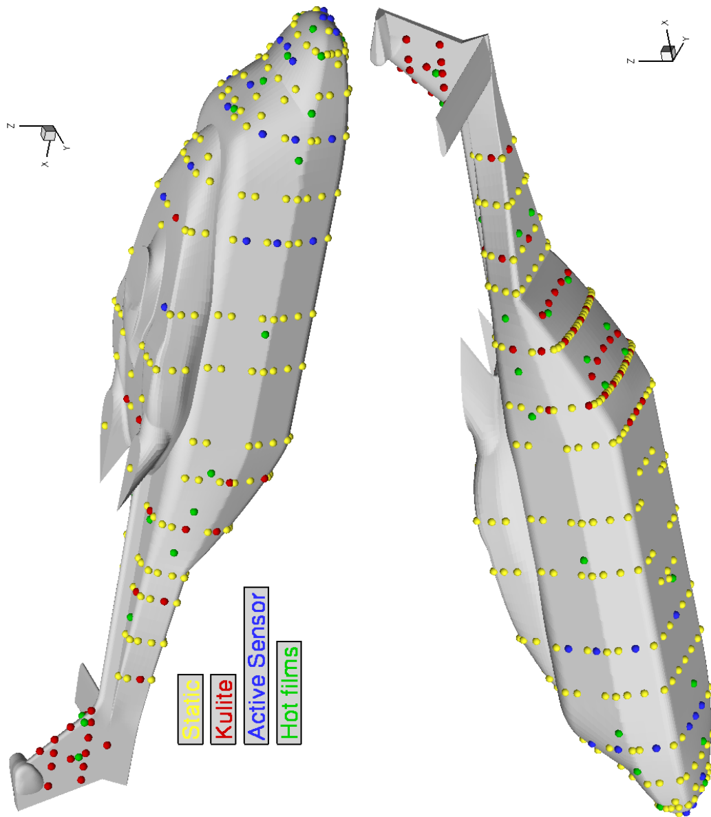
Figure 2: Overview of the sensor and hot film locations on the fuselage.
