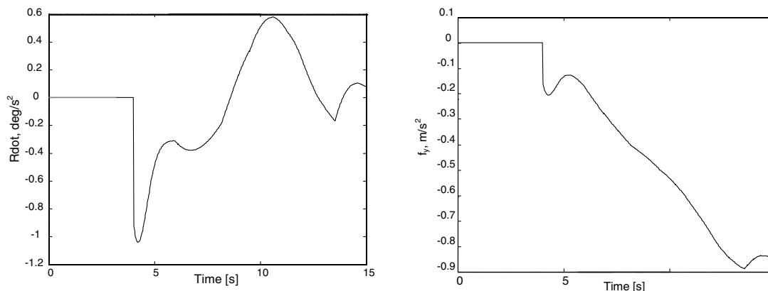
Fig. 4 Time history of yaw acceleration (left) and specific force (right) during an autoland decrab of F-100 aircraft model.
