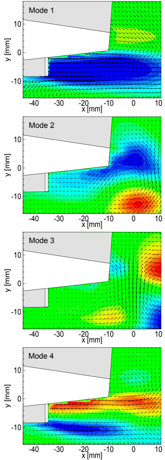
Figure 13: Dominant orthogonal modes of ramp-type AGF deployment cycle (colour contours indicate dimensionless streamwise velocity)
