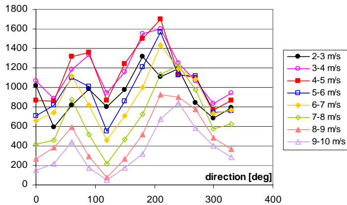
Fig. 3. Probability density for total wind speed and direction at Schiphol Airport (per 10^5 samples, [11]).
