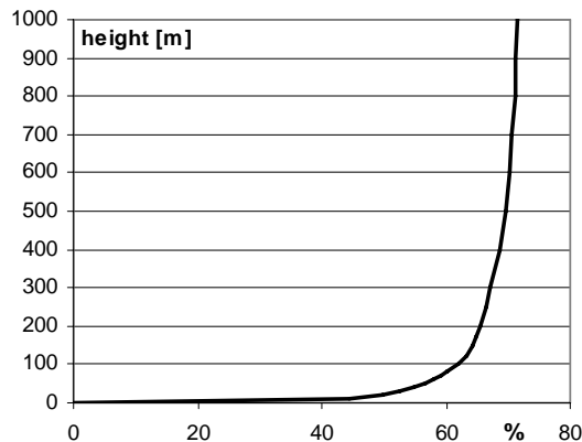
Fig. 8. Probability to exceed crosswind of 6 knts (Schiphol airport, from S-Wake [17]).
