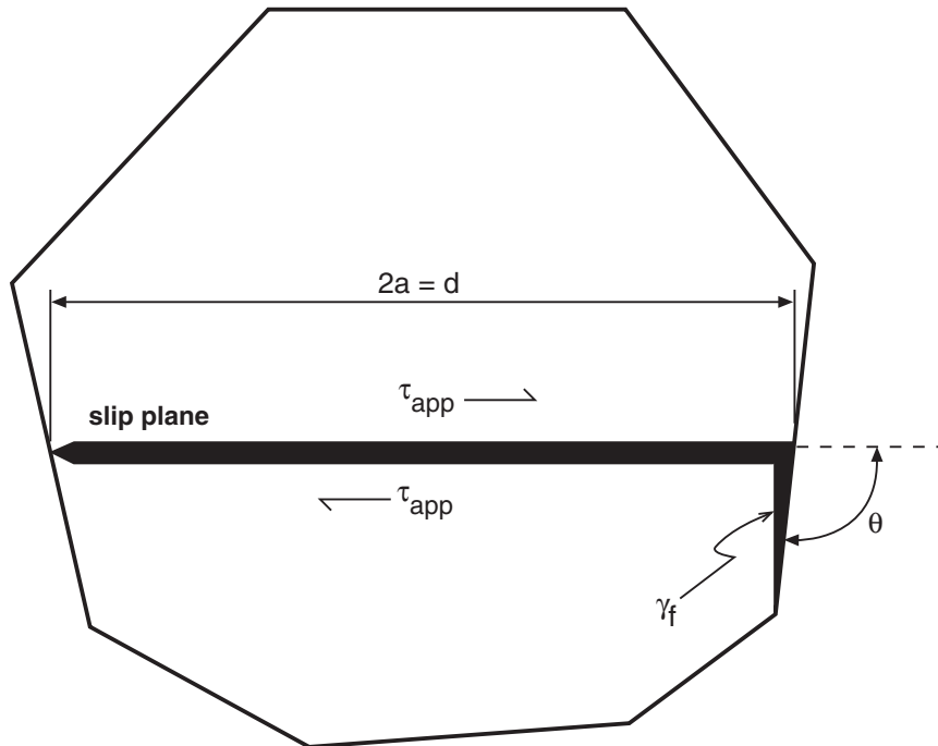
Fig. B.6 Schematics of grains containing slip band cracks under mode II shear loading by an applied shear stress, \tau_{app} , and initiation of grain boundary microcracks: (a) crack length 2a less than the grain diameter, d ; (b) crack length 2a is equal to the grain diameter, d . These configurations are applicable to corrosion-induced and synergistic embrittlement of archaeological silver
