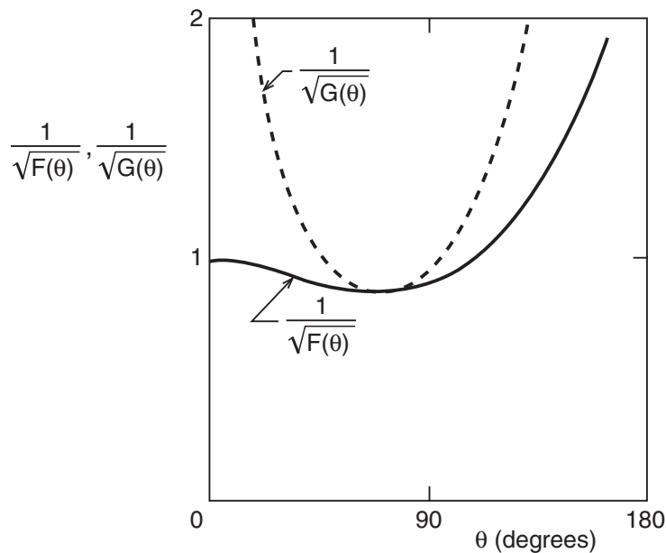
Fig. B.5 Inverse square roots of the angular functions F(\theta) and G(\theta) derived by Smith and Barnby (1967). F(\theta) is for a complete analysis of microcrack initiation ahead of an edge dislocation pile-up, see figure B.4. G(\theta) is for the same analysis but neglecting local shear stresses due to the pile-up
