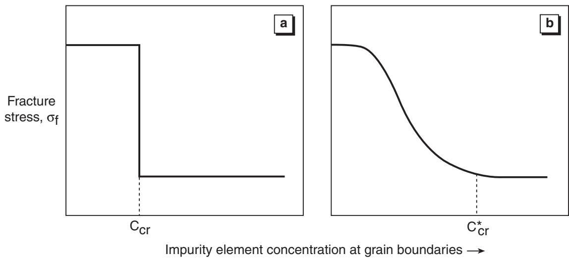
Fig. 5 Dependence of fracture stress, \sigma_f , on impurity element concentration at grain boundaries: (a) "threshold" model behaviour in which fracture stress is abruptly lowered at a critical impurity element concentration, C_{cr} ; (b) more realistic behaviour with fracture stress gradually decreasing to a minimum at a critical impurity element concentration, C_{cr}^* . After Thompson and Knott (1993)
