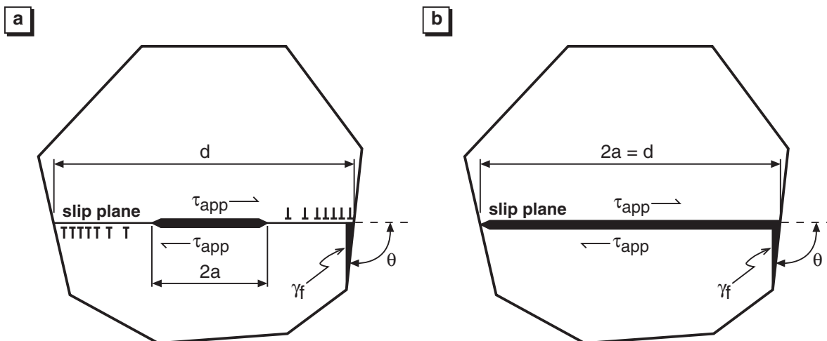
Fig. 8 Grains containing slip band cracks under mode II shear loading by an applied shear stress, \tau_{app} , and initiation of grain boundary microcracks: (a) crack length 2a less than the grain diameter, d ; (b) crack length 2a is equal to the grain diameter, d . These configurations are applicable to corrosion-induced and synergistic embrittlement of archaeological silver
