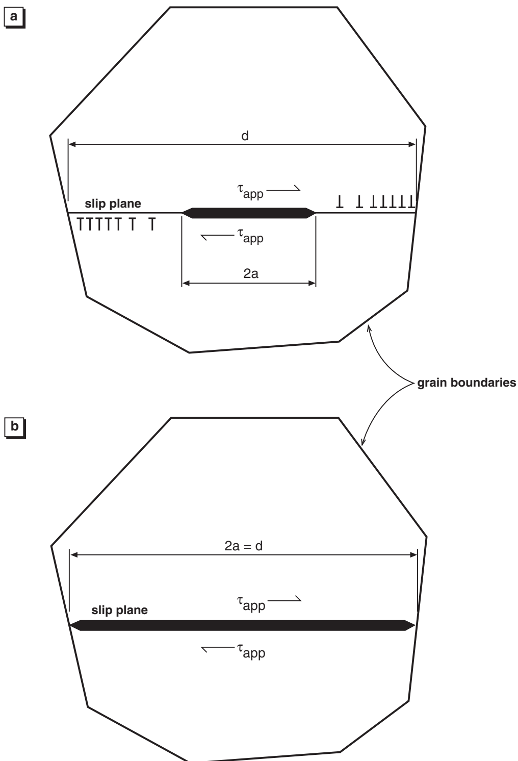
Fig. B.3 Schematics of grains containing slip band cracks under mode II shear loading by an applied shear stress, \tau_{app} : (a) crack length 2a less than the grain diameter, d ; (b) crack length 2a is equal to the grain diameter, d . These configurations are applicable to corrosion-induced embrittlement of archaeological silver
