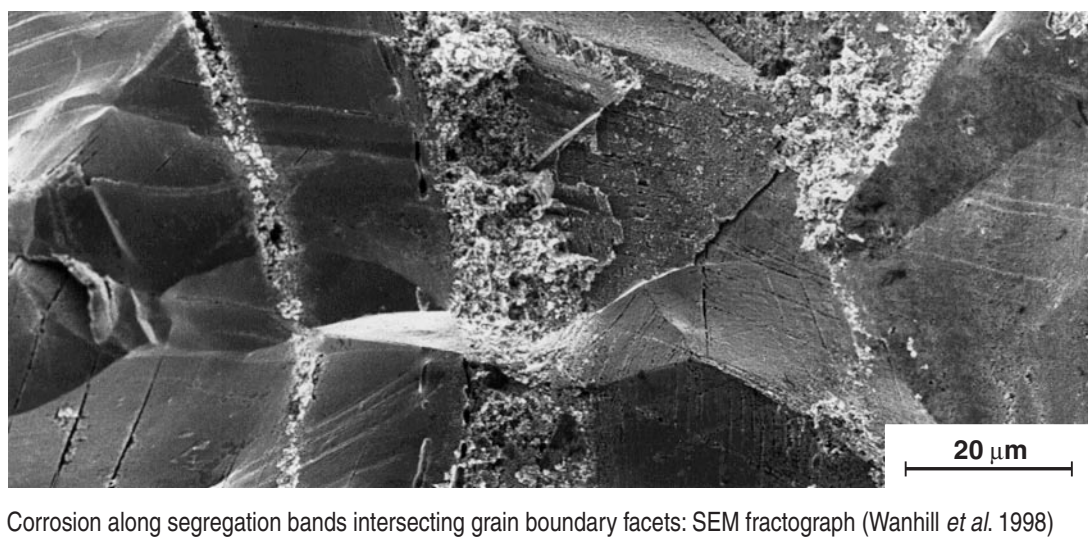
Fig. 4 Examples of synergistic embrittlement owing to microstructurally-induced embrittlement (intergranular fracture) and corrosion-induced embrittlement along slip lines, deformation twin boundaries and segregation bands: SEM = Scanning Electron Microscopy
