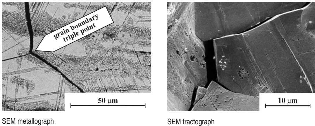
Fig. 3 Microstructurally-induced intergranular fracture in archaeological silver (Wanhill et al. 1998): SEM = Scanning Electron Microscopy
