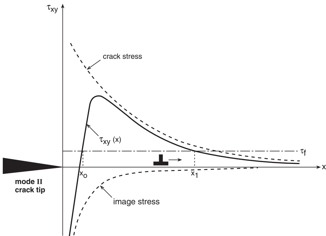
Fig. B.1 Schematic of the stress on an edge dislocation emitted from the tip of a sharp mode II crack along the coplanar slip plane. The effective shear stress, \tau_{xy}(x) , is obtained by adding the shear stress due to the crack and the dislocation image stress. The dislocation can glide in the x -direction if \tau_{xy}(x) is greater than the lattice friction stress, \tau_f . This schematic is a modification of one given by Ohr (1985)
