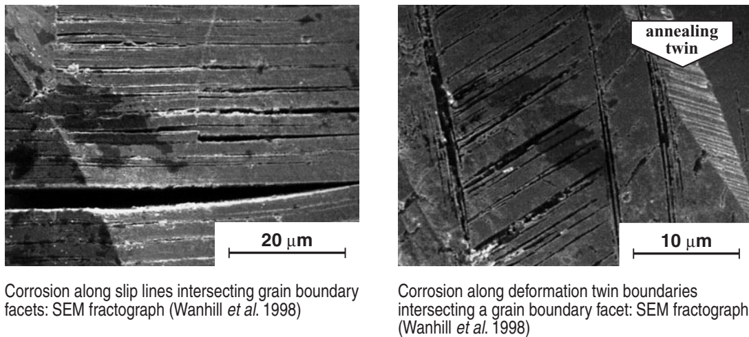
Fig. 3 Microstructurally-induced intergranular fracture in archaeological silver (Wanhill et al. 1998): SEM = Scanning Electron Microscopy
