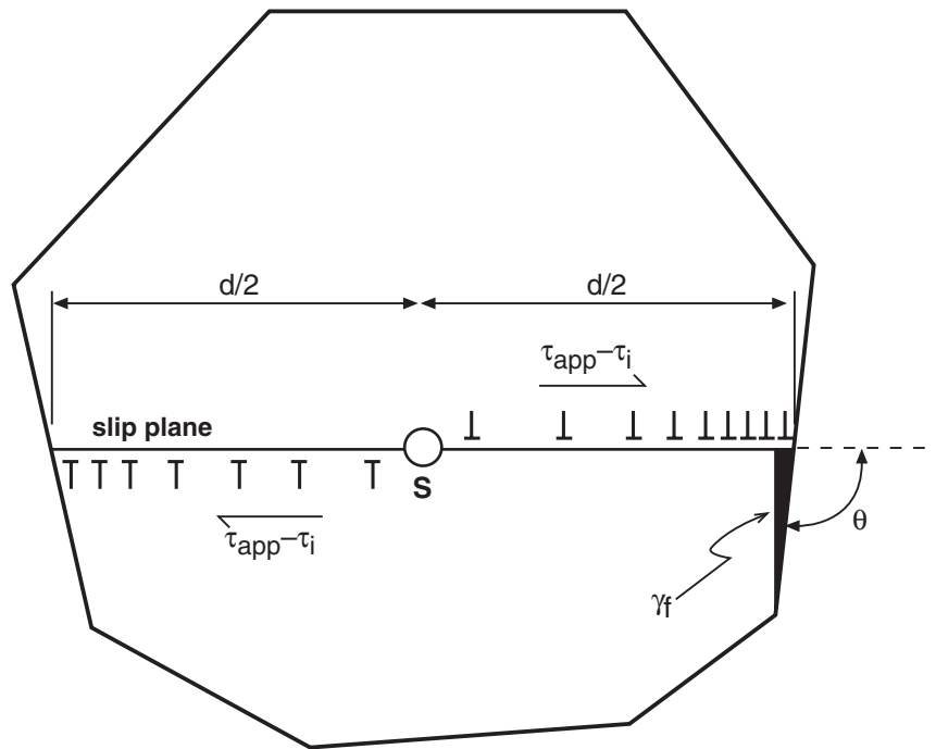
Fig. B.4 Schematic of a grain containing edge dislocation pile-ups at grain boundaries and initiation of a grain boundary microcrack. The dislocation source, S, emits dislocations under an effective shear stress, \tau_{app} - \tau_i , where \tau_{app} is the applied shear stress and \tau_i is the internal shear stress - the back stress - opposing dislocation glide away from the source. \gamma_f is the grain boundary fracture energy. This configuration is applicable to corrosion-induced and microstructurally-induced embrittlement of archaeological silver
