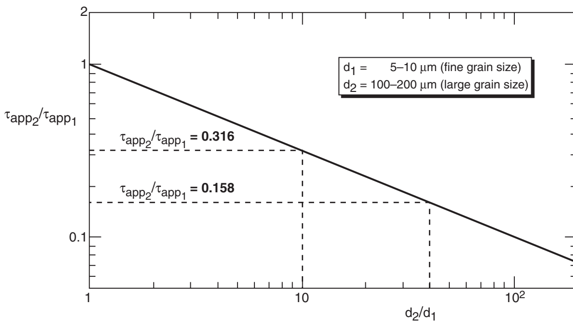
Fig. B.8 Dimensionless plot of the applied shear stress, \tau_{app} , versus average grain diameter, d , using the proportionality \tau_{app} \propto \sqrt{1/d}
