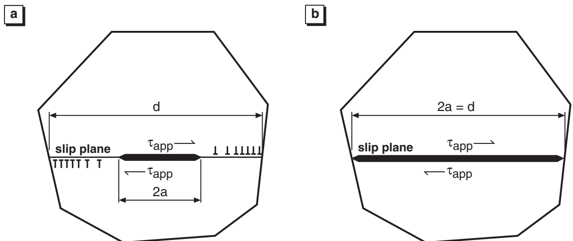
Fig. 6 Grains containing slip band cracks under mode II shear loading by an applied shear stress, \tau_{app} : (a) crack length 2a less than the grain diameter, d ; (b) crack length 2a is equal to the grain diameter, d . These configurations are applicable to corrosion-induced embrittlement of archaeological silver
