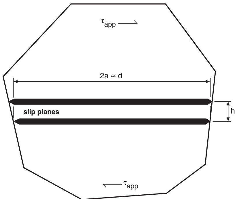
Fig. B.7 Schematic of a grain containing multiple slip band cracks under mode II shear loading by an applied shear stress, \tau_{app} . This configuration is applicable to corrosion-induced embrittlement of archaeological silver, and is a modification of the configuration in figure B.3b
