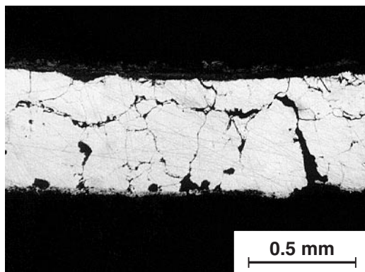
Intergranular corrosion: metallograph (Werner 1965)
