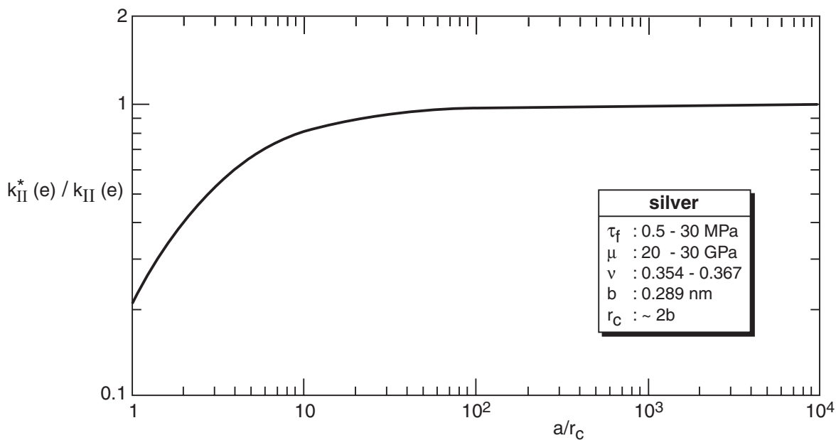
Fig. B.2 Dimensionless plot of the mode II stress intensity factors required for emission of edge dislocations from the tips of finite length cracks
