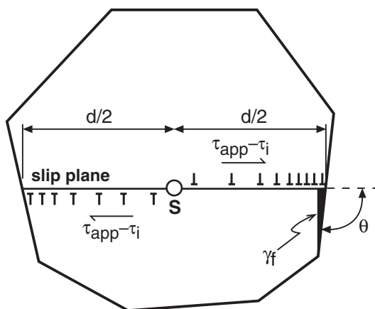
Fig. 7 Grain containing edge dislocation pile-ups at grain boundaries and initiation of a grain boundary microcrack. The dislocation source, S , emits dislocations under an effective shear stress, \tau_{app} - \tau_i , where \tau_{app} is the applied shear stress and \tau_i is the internal shear stress - the back stress - opposing dislocation glide away from the source. \gamma_f is the grain boundary fracture energy. This configuration is applicable to corrosion-induced and microstructurally-induced embrittlement of archaeological silver
