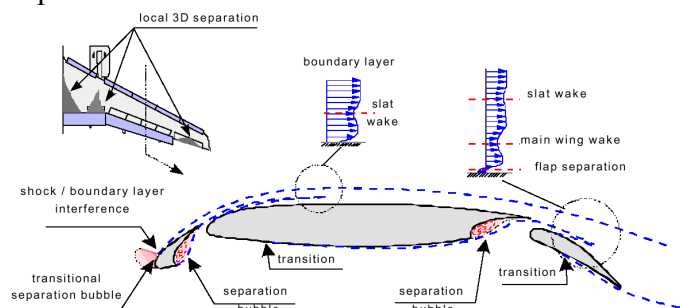
Fig. 9 Flow physics of high lift systems.
