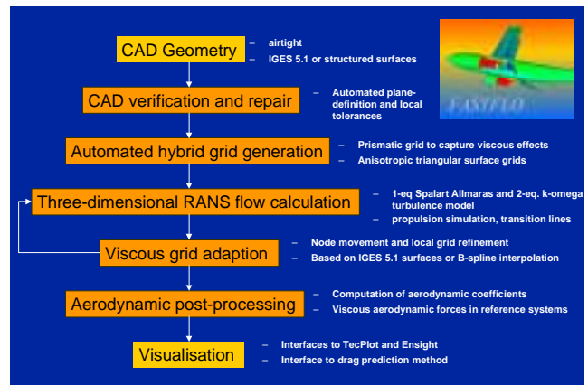
Fig. 1. Overview of the algorithmic components in the hybrid grid based CFD system as developed in the FASTFLO II project. The functionality per algorithmic component is listed.
