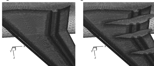
Fig. 10 Zoom of the surface grids of the slat-wing-flap configuration without and with flap track fairings.
