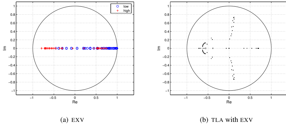
Fig. 5 Eigenvalue spectra of the EXV smoother and two-level algorithm in the unsteady diffusion dominated case ( \sigma = 1 and \text{Re}_h = 0.01 , last row of Table 4).
