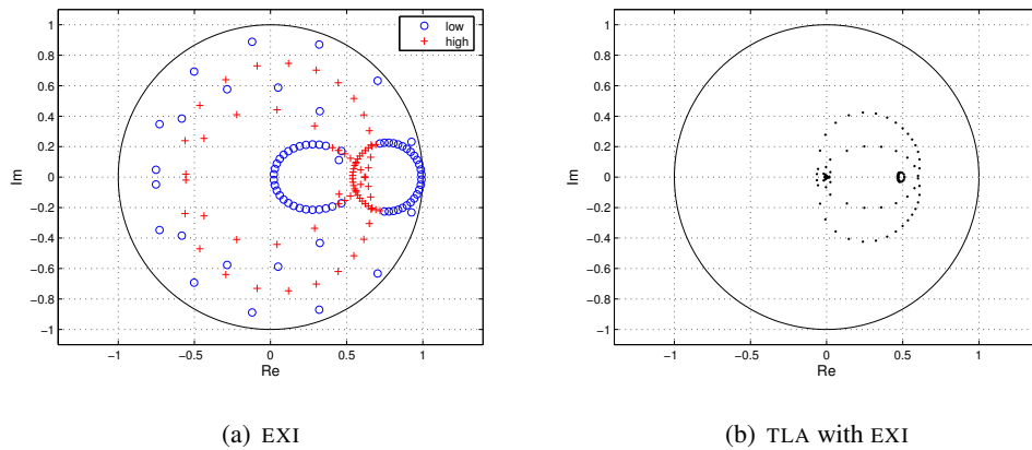
Fig. 2 Eigenvalue spectra of the EXI smoother and two-level algorithm in the steady advection dominated case ( \sigma = 100 and Re_h = 100 , first row of Table 1).
