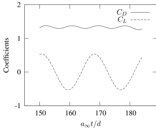
Fig. 9 Periodic evolution of the lift and drag coefficients C_L and C_D for the cylinder at M_\infty = 0.3 and Re_\infty = 200 .
