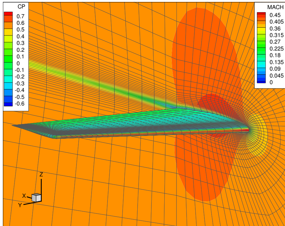
Fig. 11 Impression of the grid, the Mach number isolines and the pressure coefficient C_p on the ONERA M6 wing at M_\infty = 0.4 , Re_\infty = 10^4 and \alpha = 1^\circ .
