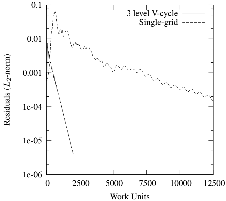
Fig. 7 Convergence to steady-state for the cylinder at M_\infty = 0.3 and Re_\infty = 40 on the 64 \times 64 \times 4 grid.
