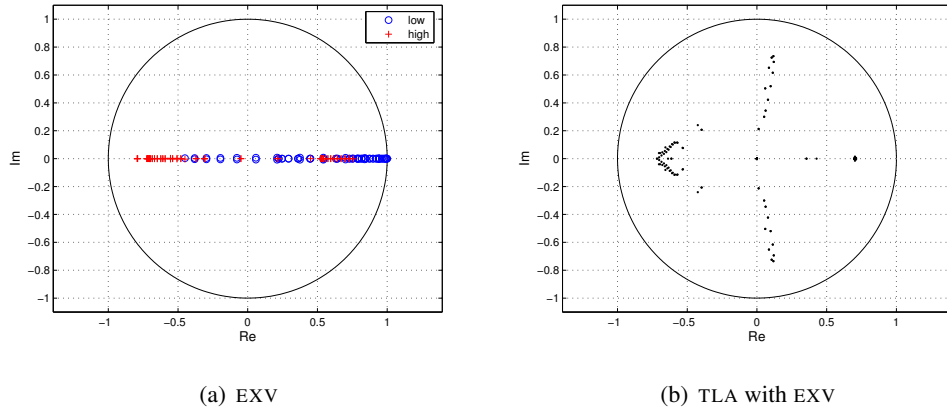
Fig. 3 Eigenvalue spectra of the EXV smoother and two-level algorithm in the steady diffusion dominated case ( \sigma = 100 and Re_h = 0.01 , last row of Table 2).
