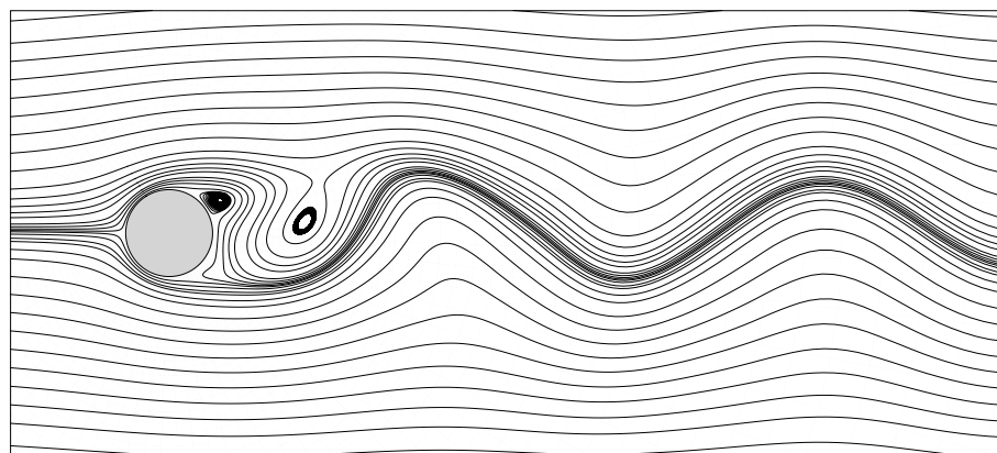
(b) streamlines
