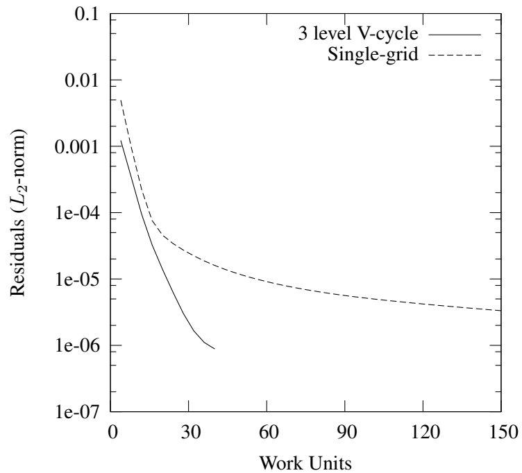
Fig. 10 Typical convergence in pseudo-time for a physical time-step a_\infty \Delta t/d = 0.5 for the cylinder at M_\infty = 0.3 and Re_\infty = 200 on the 80 \times 84 \times 4 grid.
