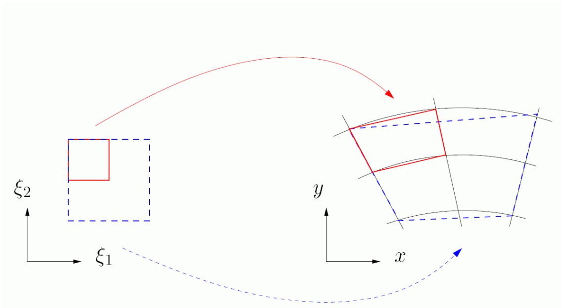
Fig. 1 Relation between two grid levels in computational and physical space.
