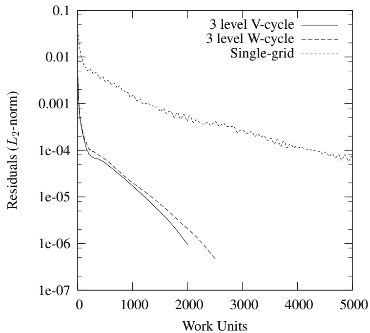
Fig. 12 Convergence in pseudo-time for the ONERA M6 wing at M_\infty = 0.4 , Re_\infty = 10^4 and \alpha = 1^\circ .
