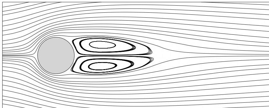
(b) streamlines
