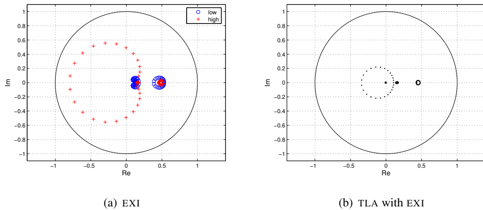
Fig. 4 Eigenvalue spectra of the EXI smoother and two-level algorithm in the unsteady advection dominated case ( \sigma = 1 and Re_h = 100 , first row of Table 3).
