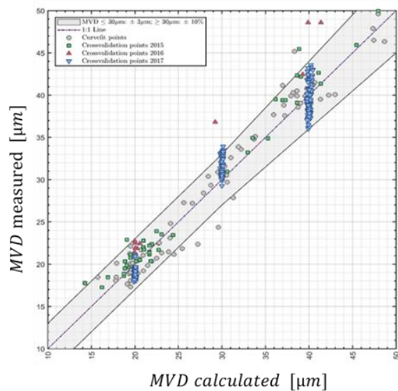
Figure 10: Comparison between measured data and the curve fit for MVD since 2014.
