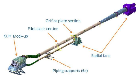
Figure 1: Full-scale intake model as used during the intake IWT of the KUH-1 at RTA. Total length is approximately 32 meters.
