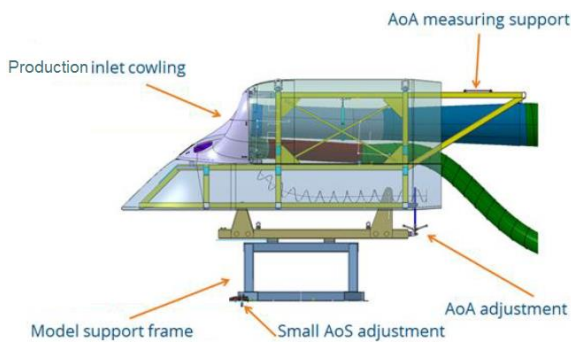
Figure 2: KUH-1 wind tunnel model including production intake cowling.
