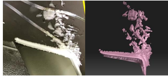
Figure 15: 3-D scan of ice accreted on left-hand engine cooling inlet.
