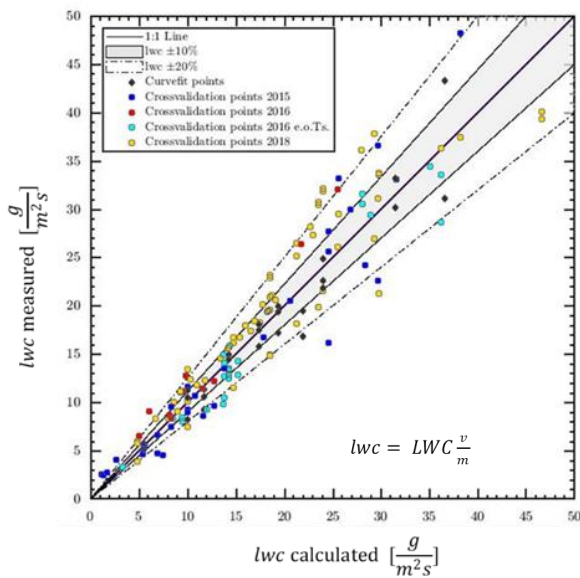
Figure 9: Comparison between measured data and the curve fit for LWC since 2014.
