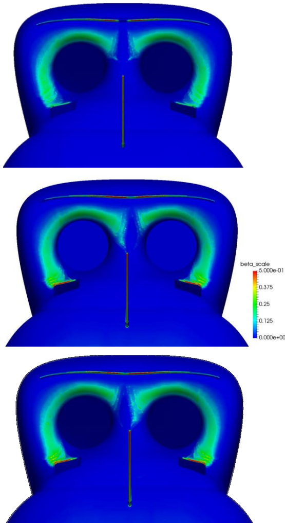
Figure 13: Comparison of predicted drop collection efficiency in free-flight at 10,000 ft pressure altitude (top), and in Weber (middle) and Reynolds number (bottom) scaled sea level test conditions inside RTA test section. Courtesy: AeroTex UK.
