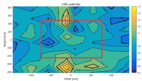
Figure 12: LWC uniformity measurement at 50 m/s with LWC 0,95 g/m³ in the empty test section.
