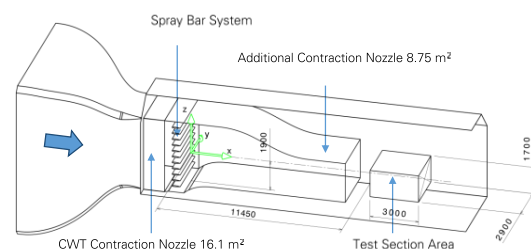
Figure 7: Test configuration with additional contraction nozzle ( 8.75 \text{ m}^2 cross section), as used during the KUH-1 test.
