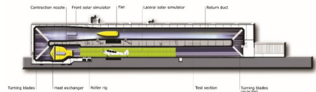
Figure 5: Large Climatic Wind Tunnel.
