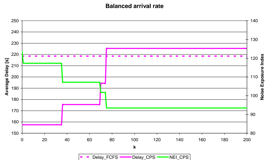
Figure 6: Scheduler results for an arrival rate near the runway capacity
