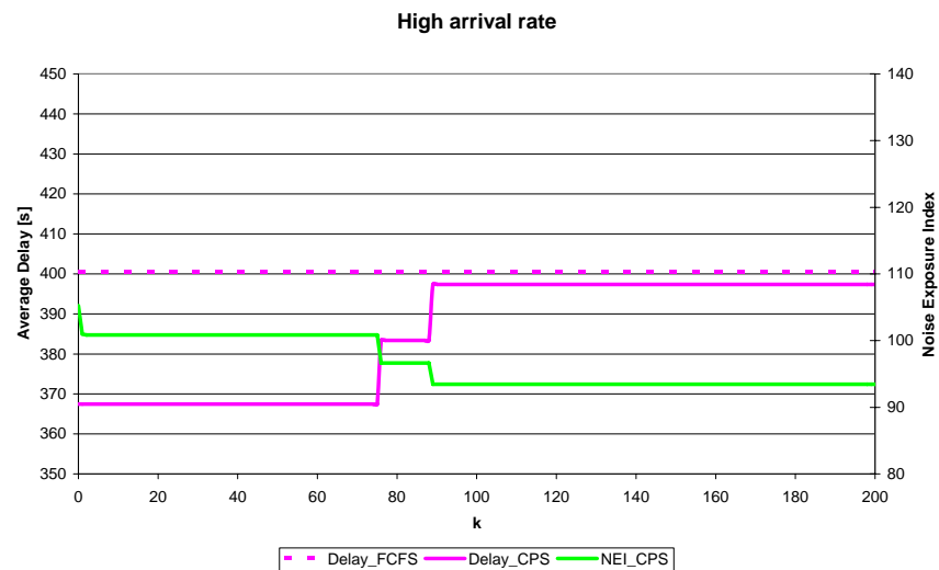
Figure 5: Scheduler results for an arrival rate higher than the runway capacity
