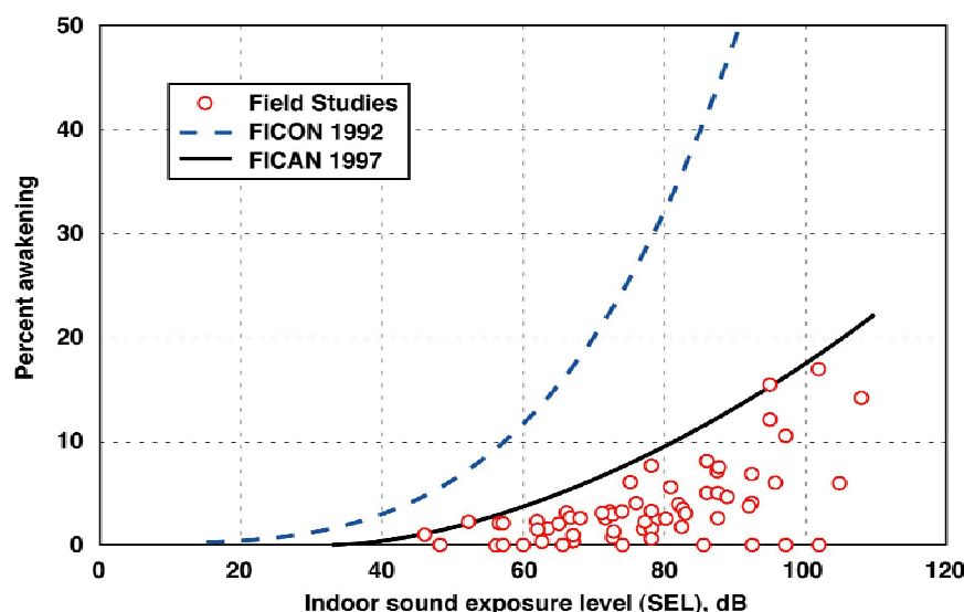
Figure 3: FICAN proposed sleep disturbance dose-response relationship (source: Ref. 15)
