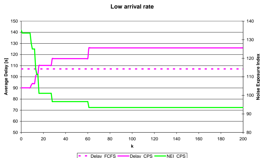
Figure 7: Scheduler results for an arrival rate lower than the runway capacity
