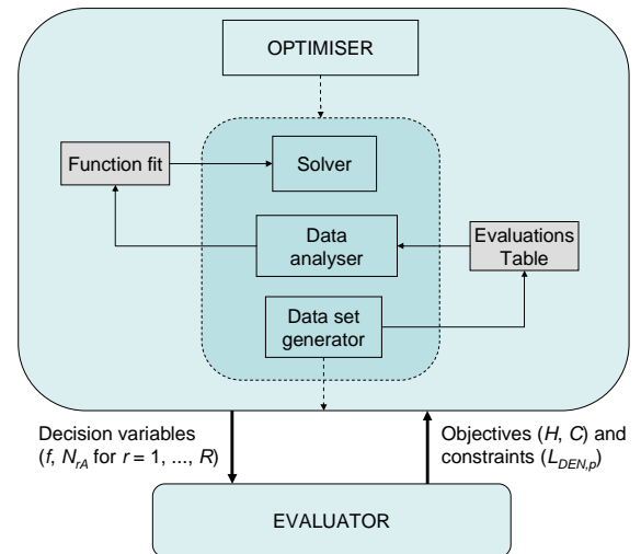
Fig. 2. Data flow in the optimiser module
